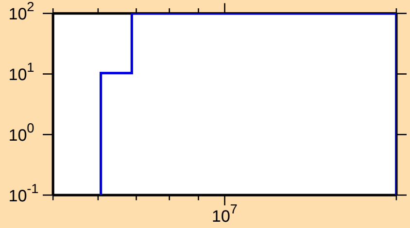
\Delta\sigma/\sigma vs. E for ^{225}\text{At}(n,p)
