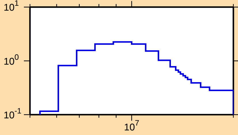
\sigma vs. E for ^{225}\text{At}(n,2n)
