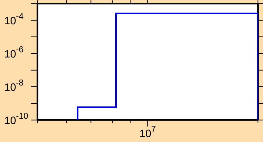
\sigma vs. E for ^{225}\text{At}(n,p)
