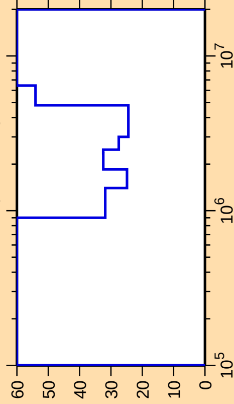
\Delta\sigma/\sigma vs. E for ^{225}\text{At}(n,\text{ncont.})
