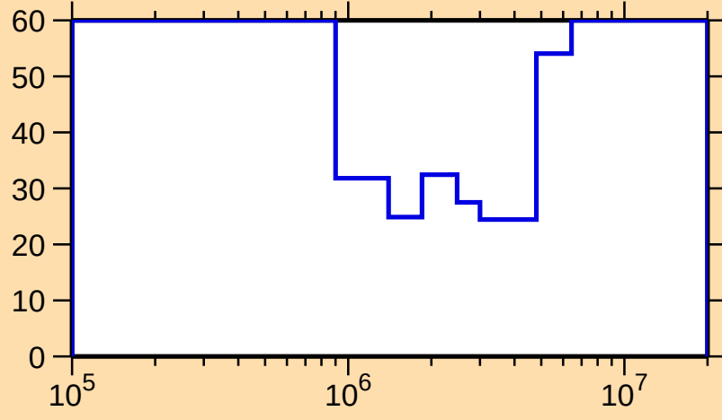
\Delta\sigma/\sigma vs. E for ^{225}\text{At}(n,n\text{cont.})
