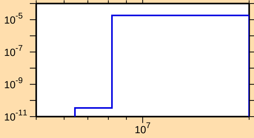
\sigma vs. E for ^{225}\text{At}(n,n\alpha)
