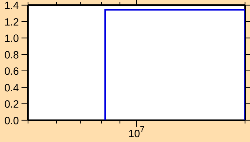
\sigma vs. E for ^{225}\text{At}(n,3n)
