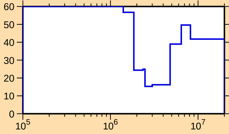
\Delta\sigma/\sigma vs. E for ^{225}\text{At}(n,\text{tot.})
