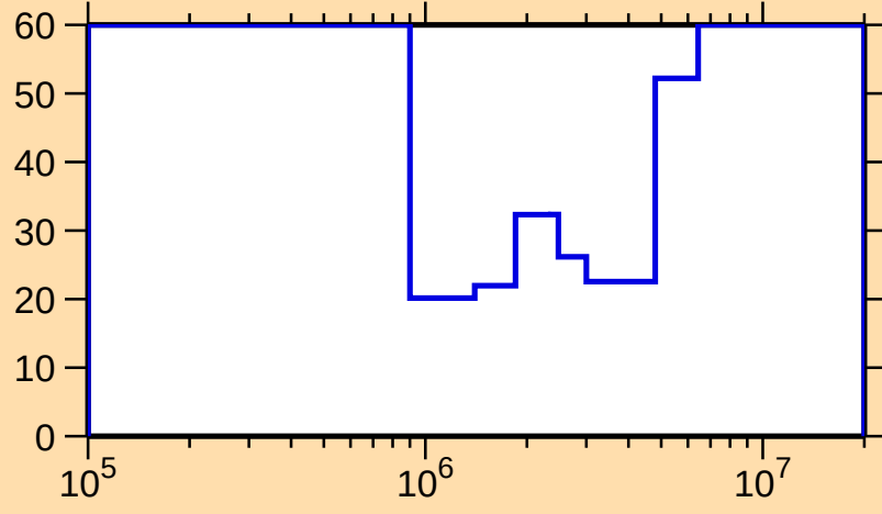
\Delta\sigma/\sigma vs. E for ^{225}\text{At}(n,\text{inel.})
