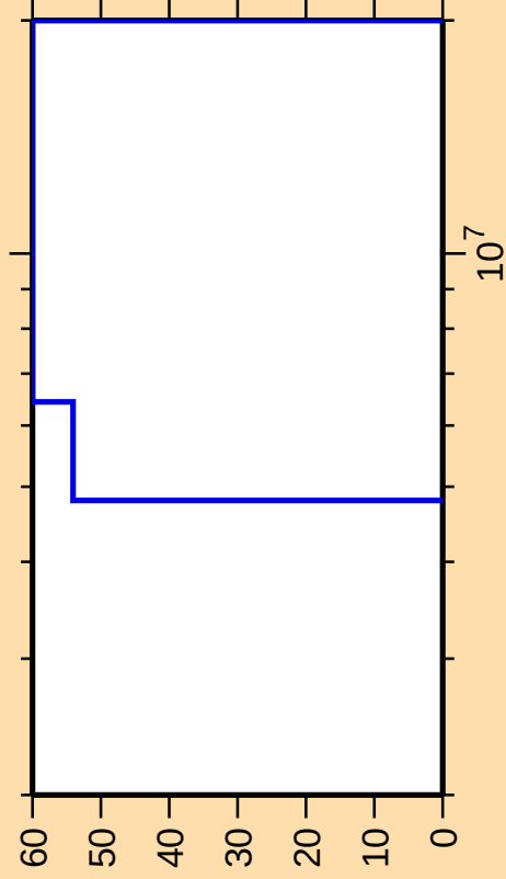
\Delta\sigma/\sigma vs. E for ^{225}\text{At}(n,n\text{cont.})
