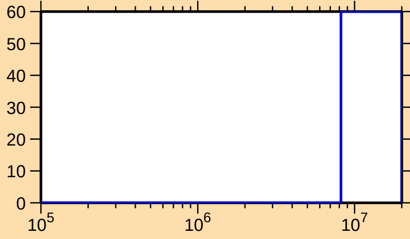
\Delta\sigma/\sigma vs. E for ^{225}\text{At}(n,f)
