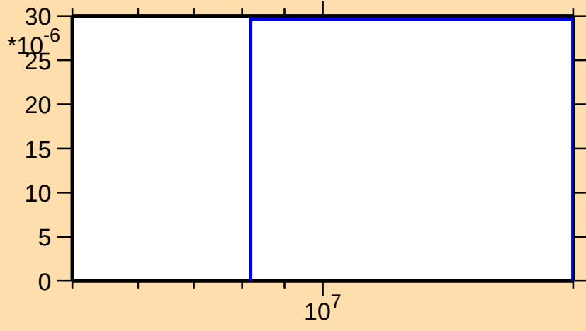
\sigma vs. E for ^{225}\text{At}(n,np)
