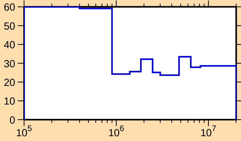
\Delta\sigma/\sigma vs. E for ^{225}\text{At}(n,\text{nonel.})
