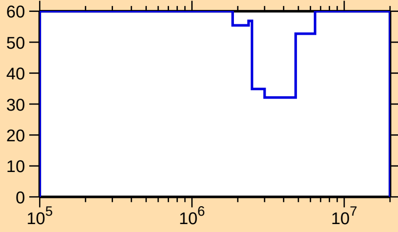
\Delta\sigma/\sigma vs. E for ^{225}\text{At}(n,\text{el.})
