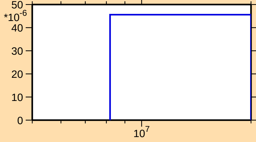
\sigma vs. E for ^{225}\text{At}(n,d)
