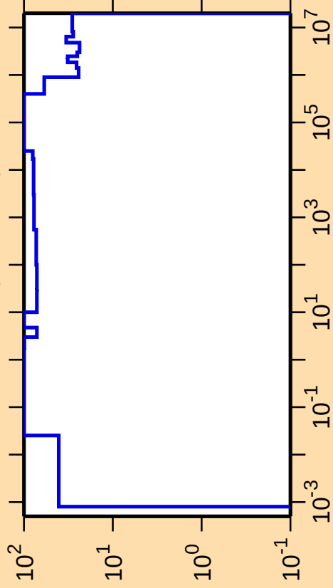
\Delta\sigma/\sigma vs. E for ^{225}\text{At}(n,\text{nonel.})
