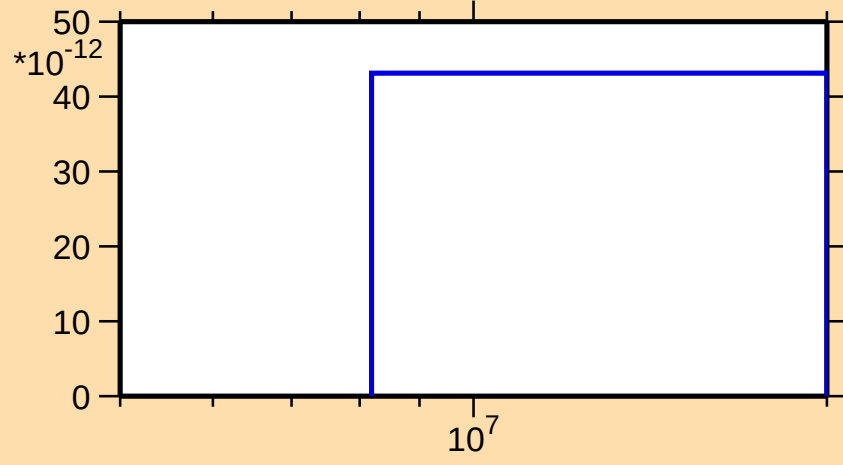
\sigma vs. E for ^{225}\text{At}(n,3n\alpha)
