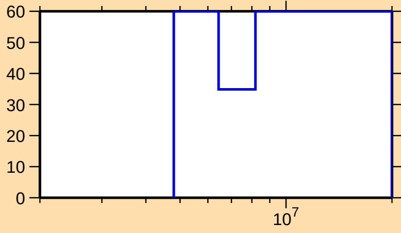
\Delta\sigma/\sigma vs. E for ^{225}\text{At}(n,2n)
