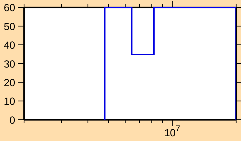
\Delta\sigma/\sigma vs. E for ^{225}\text{At}(n,2n)
