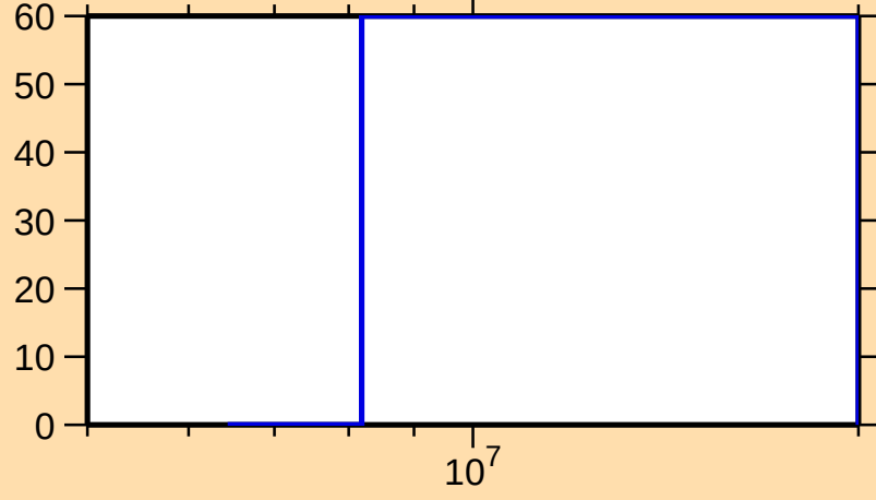
\Delta\sigma/\sigma vs. E for ^{225}\text{At}(n,f)
