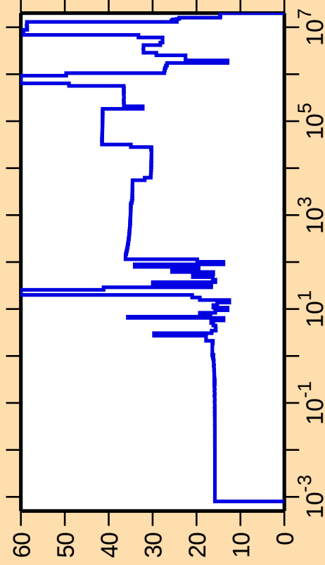
\Delta\sigma/\sigma vs. E for ^{226}\text{At}(n,\text{el.})
