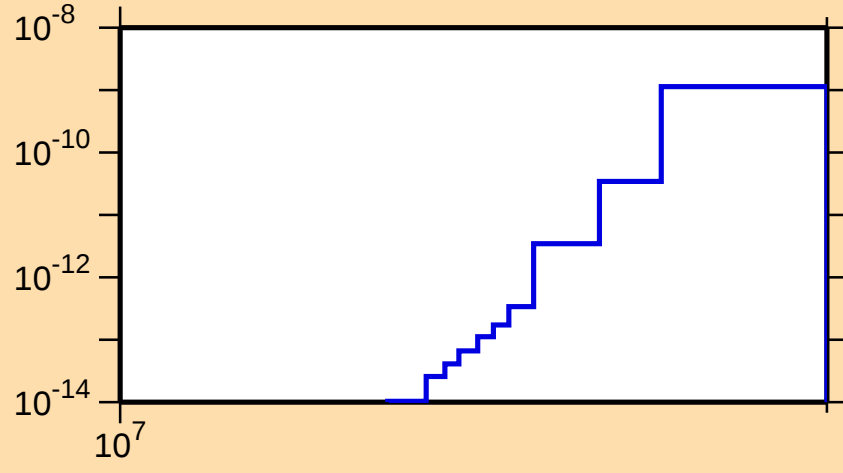
\sigma vs. E for ^{226}\text{At}(n,3n\alpha)
