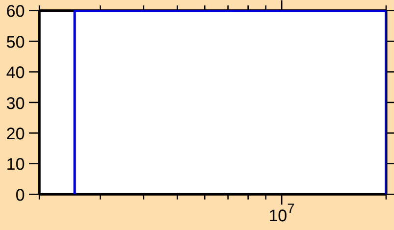
\Delta\sigma/\sigma vs. E for ^{226}\text{At}(n,\gamma)
