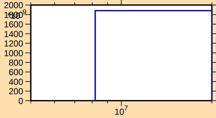
\sigma vs. E for ^{226}\text{At}(n,\text{nt})
