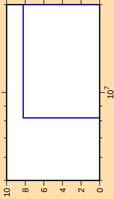
\Delta\sigma/\sigma vs. E for ^{226}\text{At}(\text{mt } 11)
