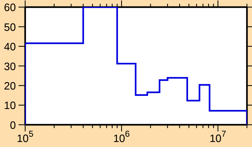
\Delta\sigma/\sigma vs. E for ^{226}\text{At}(n,\text{tot.})
