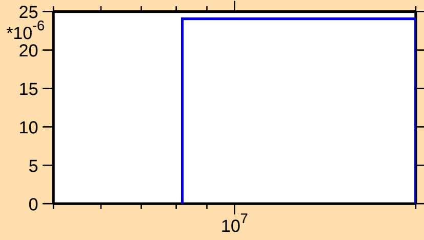
\sigma vs. E for ^{226}\text{At}(n,np)
