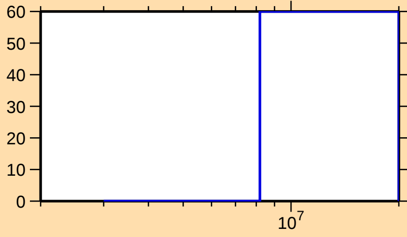
\Delta\sigma/\sigma vs. E for ^{226}\text{At}(n,f)
