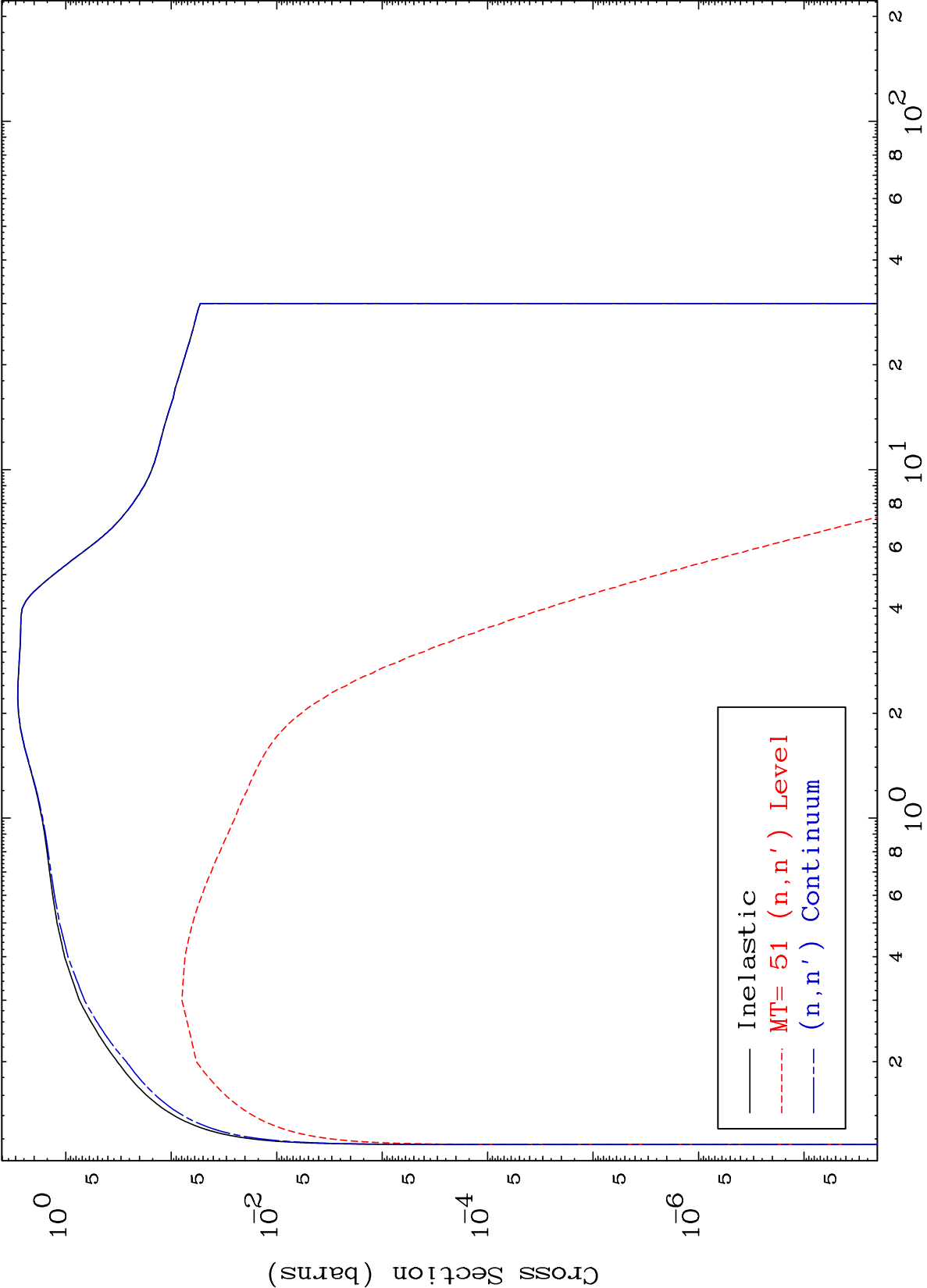
(n,n') Level 293 Kelvin Cross Sections
