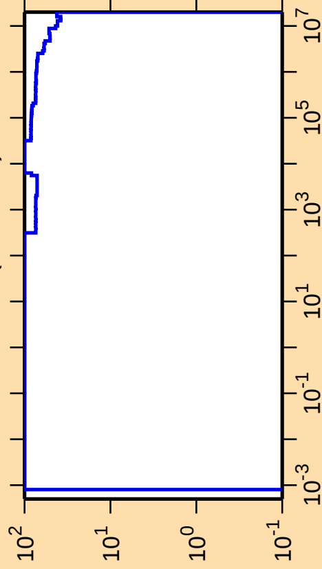
\Delta\sigma/\sigma vs. E for ^{176}\text{Au}(n,\text{nonel.})
