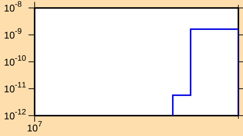
\sigma vs. E for ^{176}\text{Au}(n,nt)
