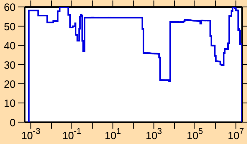
\Delta\sigma/\sigma vs. E for ^{176}\text{Au}(n,\text{tot.})
