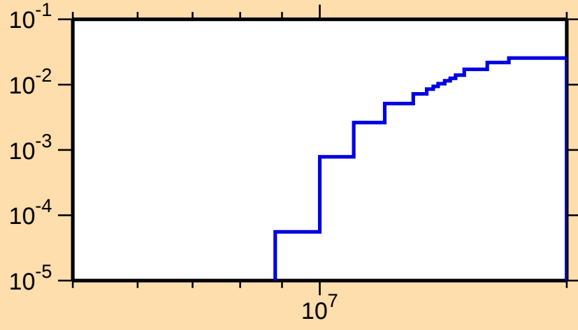
\sigma vs. E for ^{176}\text{Au}(n,2n)
