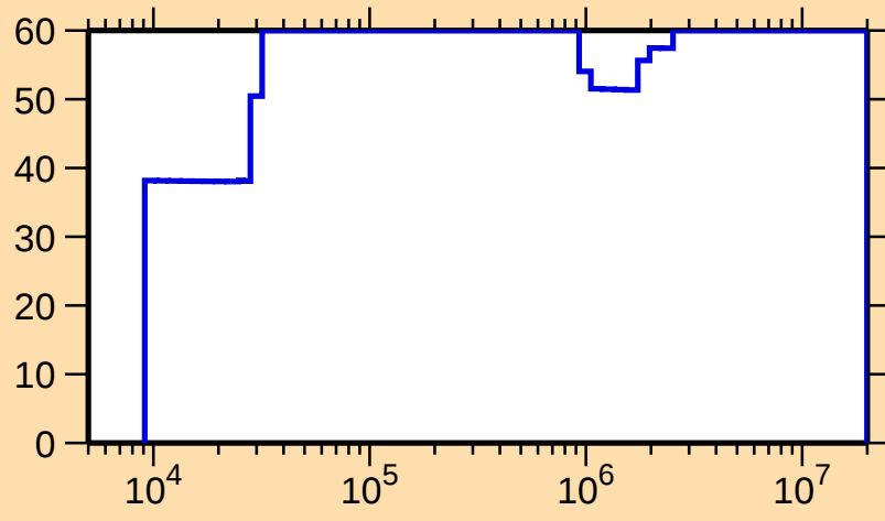
\Delta\sigma/\sigma vs. E for ^{176}\text{Au}(n,\text{el.})
