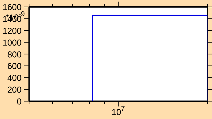
\sigma vs. E for ^{176}\text{Au}(n,pt)
