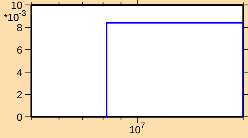
\sigma vs. E for ^{176}\text{Au}(n,2n)
