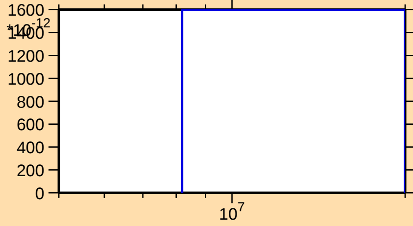
\sigma vs. E for ^{176}\text{Au}(\text{mt } 34)
