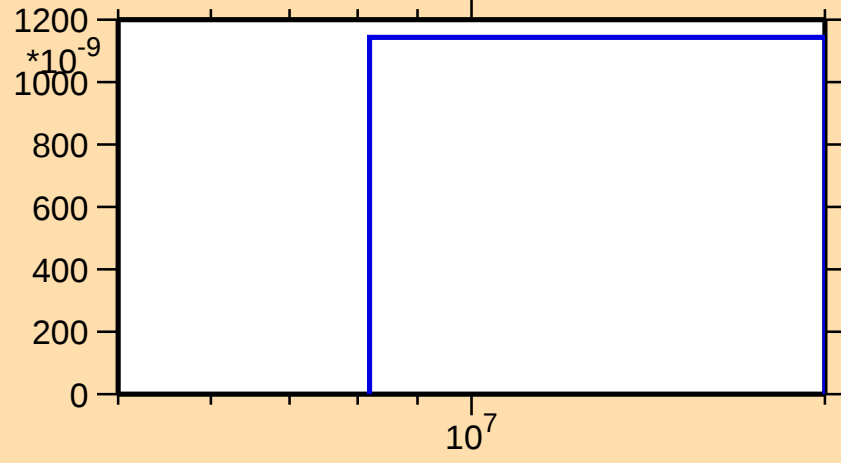
\sigma vs. E for ^{176}\text{Au}(n,nd)
