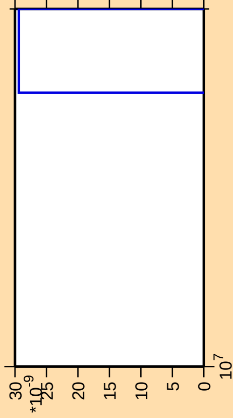
\Delta\sigma/\sigma vs. E for ^{177}\text{Au}(\text{mt } 42)
