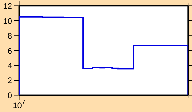
\Delta\sigma/\sigma vs. E for ^{177}\text{Au}(n,\text{el.})
