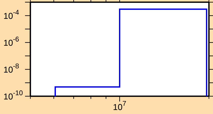
\sigma vs. E for ^{177}\text{Au}(n,t)
