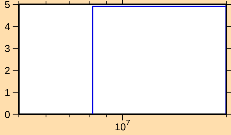
\Delta\sigma/\sigma vs. E for ^{177}\text{Au}(n,\text{nonel.})
