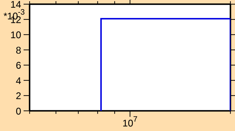
\sigma vs. E for ^{177}\text{Au}(n,2n)
