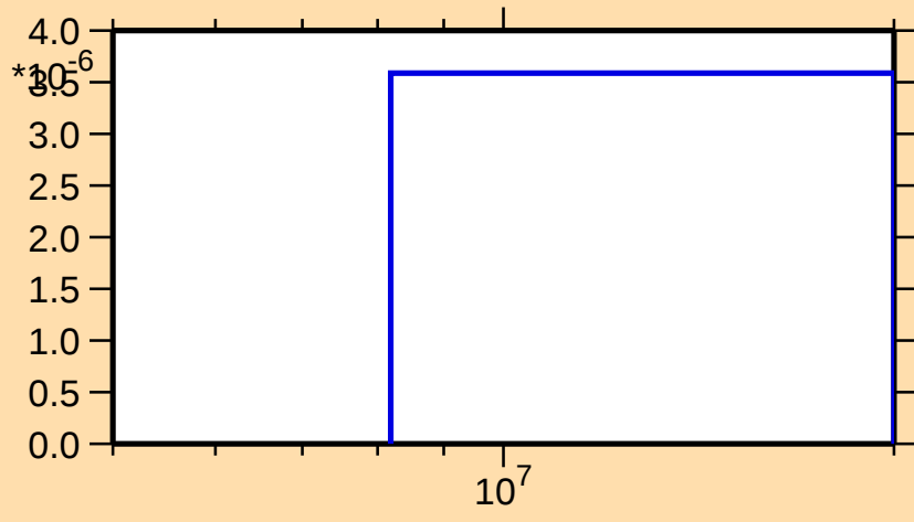
\sigma vs. E for ^{177}\text{Au}(n,2n\alpha)
