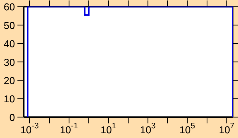
\Delta\sigma/\sigma vs. E for ^{177}\text{Au}(n,\gamma)
