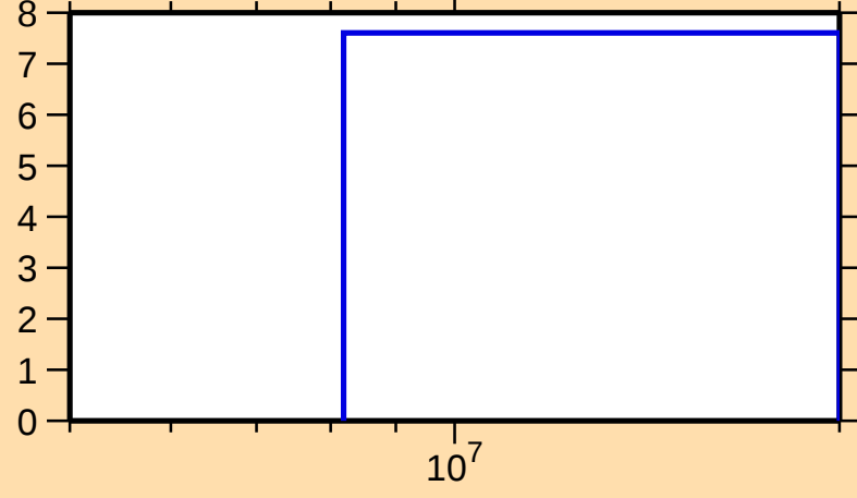
\Delta\sigma/\sigma vs. E for ^{177}\text{Au}(n,\text{el.})
