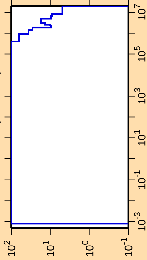
\Delta\sigma/\sigma vs. E for ^{177}\text{Au}(n,\text{nonel.})
