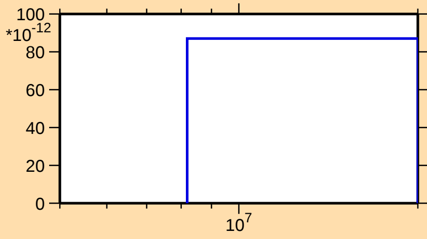
\sigma vs. E for ^{177}\text{Au}(n,nt)
