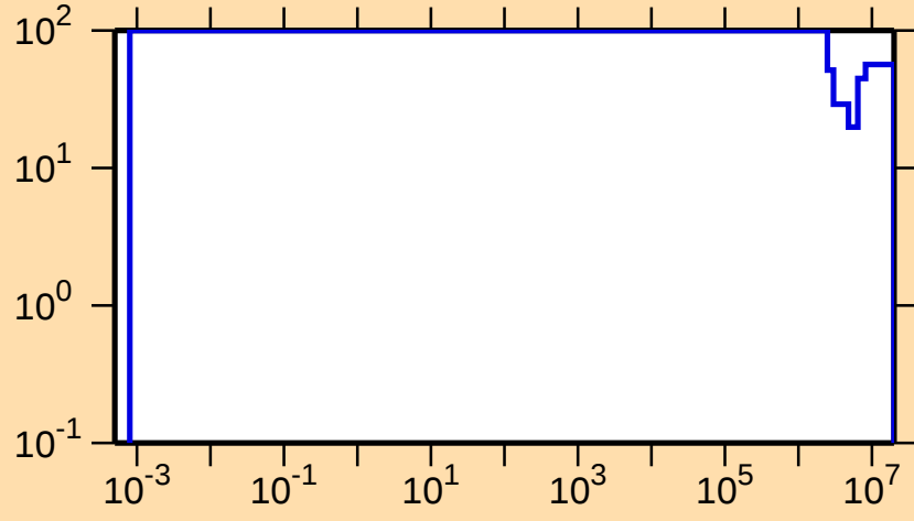
\Delta\sigma/\sigma vs. E for ^{177}\text{Au}(n,p)
