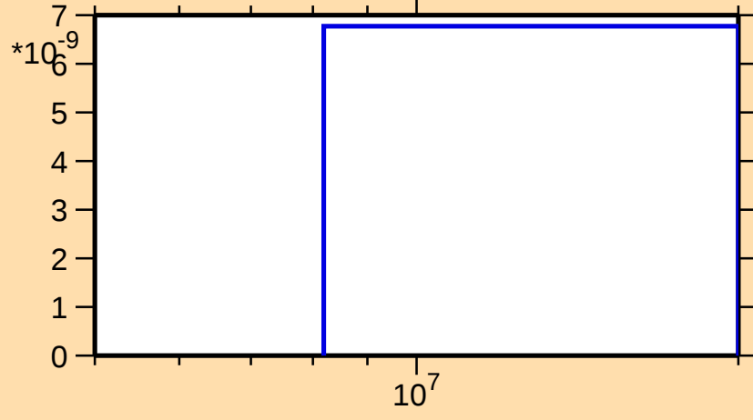
\sigma vs. E for ^{177}\text{Au}(n,\text{pt})
