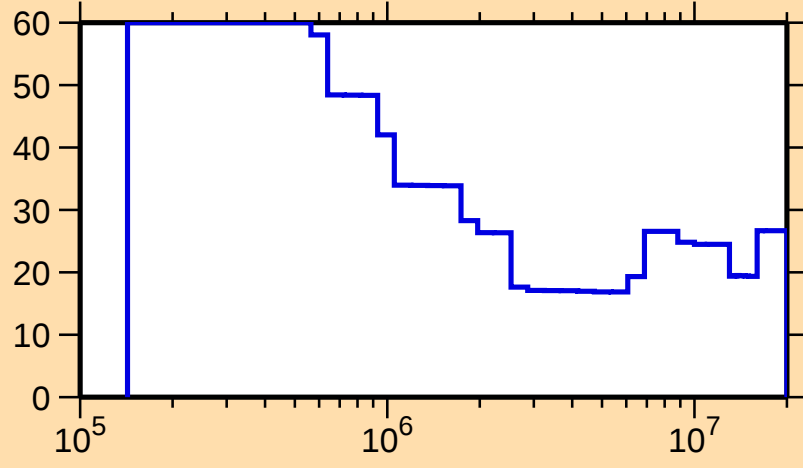
\Delta\sigma/\sigma vs. E for ^{180}\text{Au}(n,n\text{onel.})
