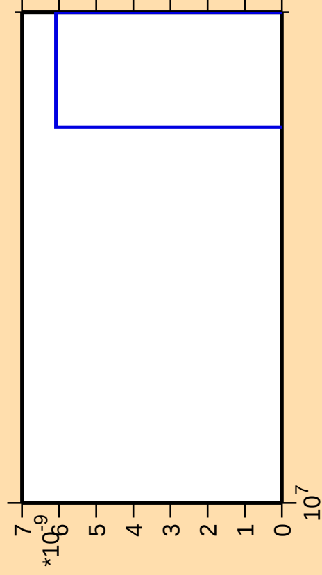
\Delta\sigma/\sigma vs. E for ^{180}\text{Au}(\text{mt } 42)
