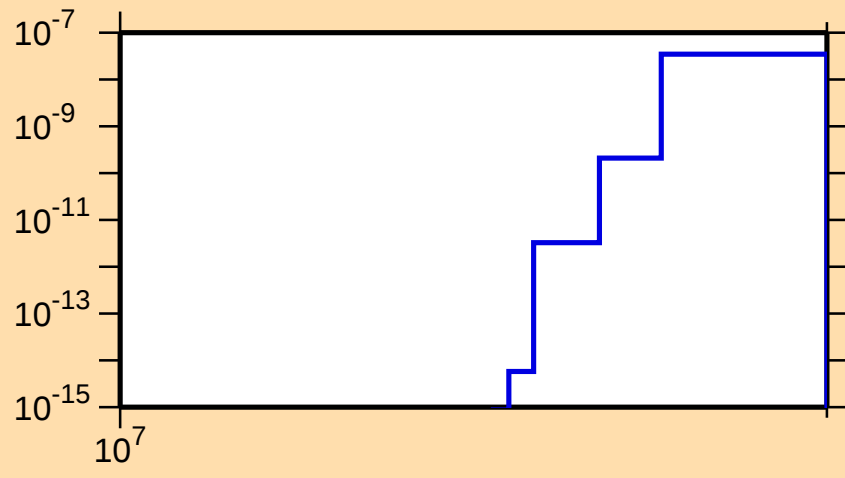
\sigma vs. E for ^{180}\text{Au}(n,nt)
