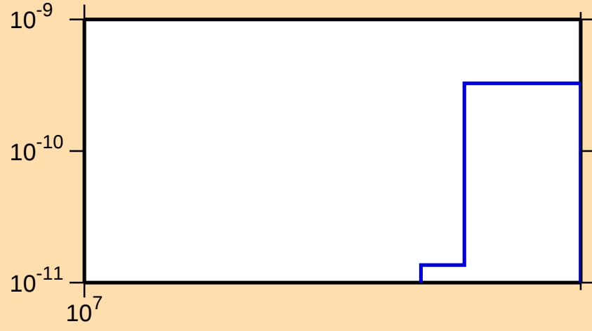
\sigma vs. E for ^{181}\text{Au} (mt 34)
