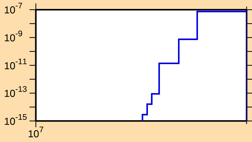
\sigma vs. E for ^{181}\text{Au}(n,nt)
