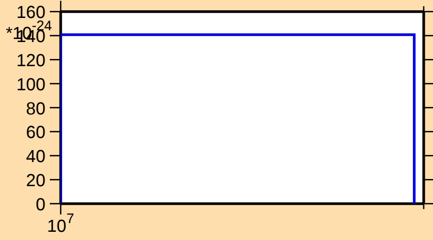
\sigma vs. E for ^{181}\text{Au}(\text{mt } 42)
