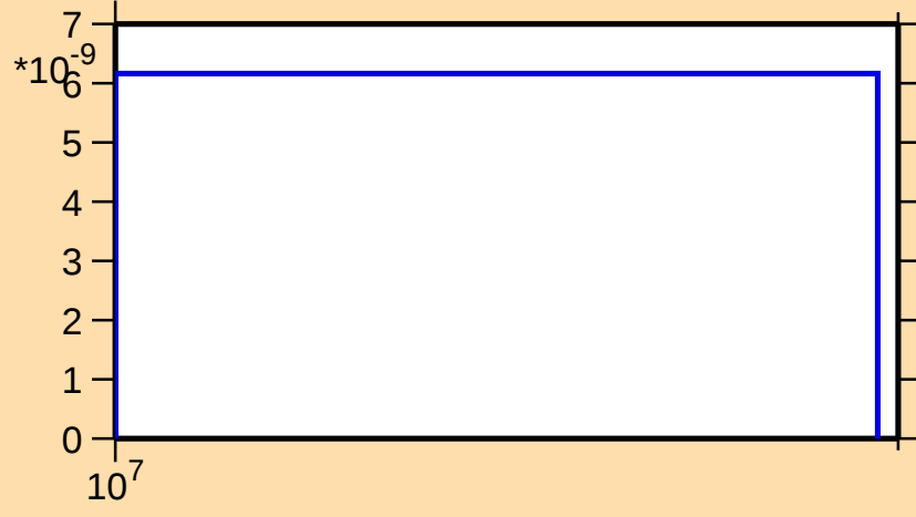
\sigma vs. E for ^{181}\text{Au}(n,3n\alpha)
