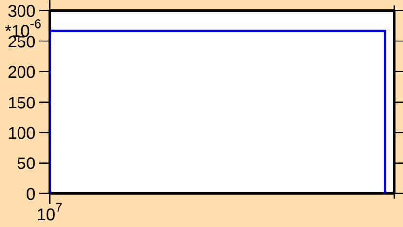
\sigma vs. E for ^{181}\text{Au}(n,2np)
