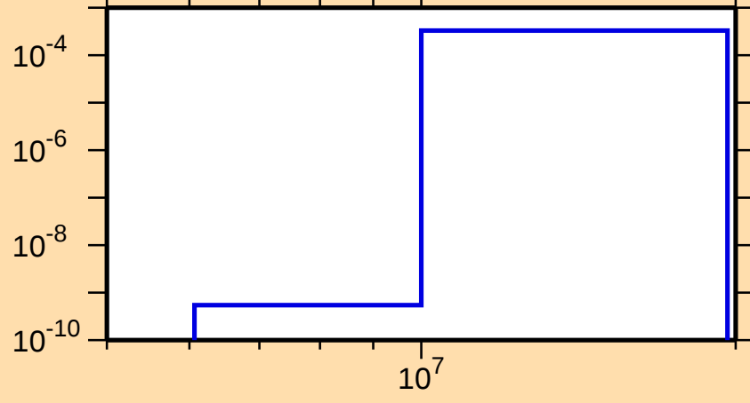
\sigma vs. E for ^{181}\text{Au}(n,t)
