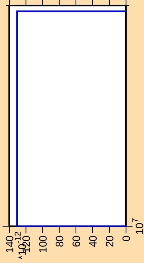
\Delta\sigma/\sigma vs. E for ^{181}\text{Au}(\text{mt } 42)
