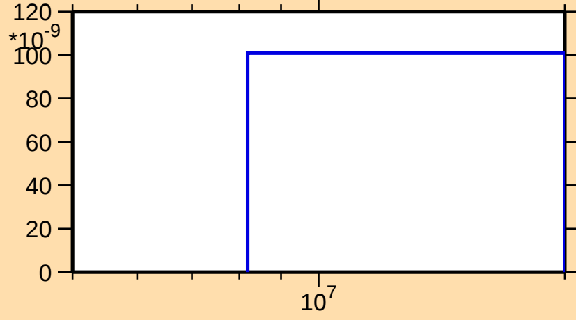
\sigma vs. E for ^{181}\text{Au}(n,\text{pd})
