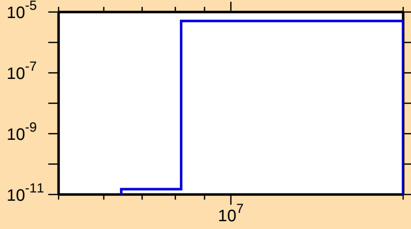
\sigma vs. E for ^{181}\text{Au}(n,\text{He}3)
