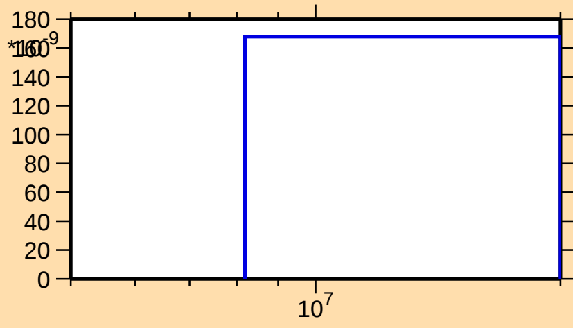
\sigma vs. E for ^{181}\text{Au}(n,\text{nd})
