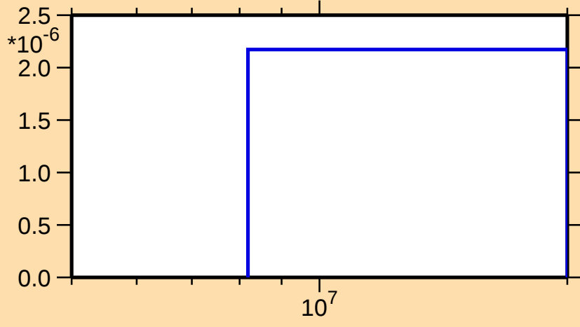
\sigma vs. E for ^{181}\text{Au}(n,2n\alpha)
