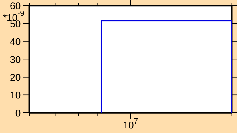
\sigma vs. E for ^{181}\text{Au}(n,3n)
