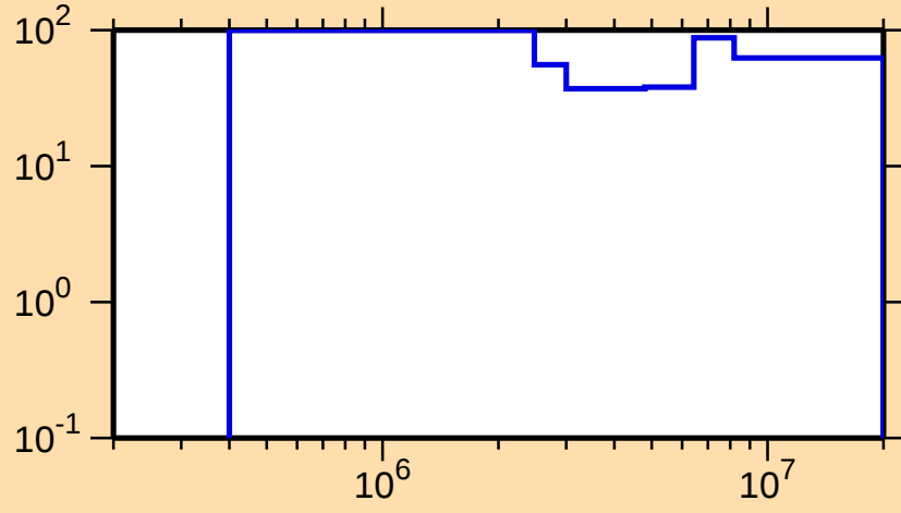
\Delta\sigma/\sigma vs. E for ^{185}\text{Au}(n, n_1)
