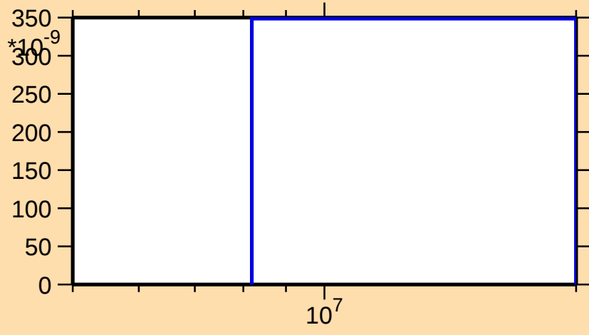
\sigma vs. E for ^{185}\text{Au}(n,\text{He}3)
