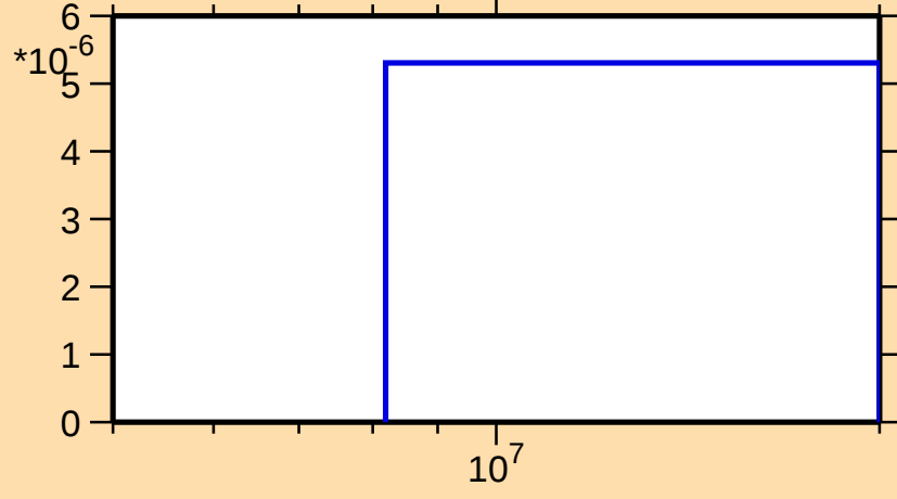
\sigma vs. E for ^{185}\text{Au}(n,3n)
