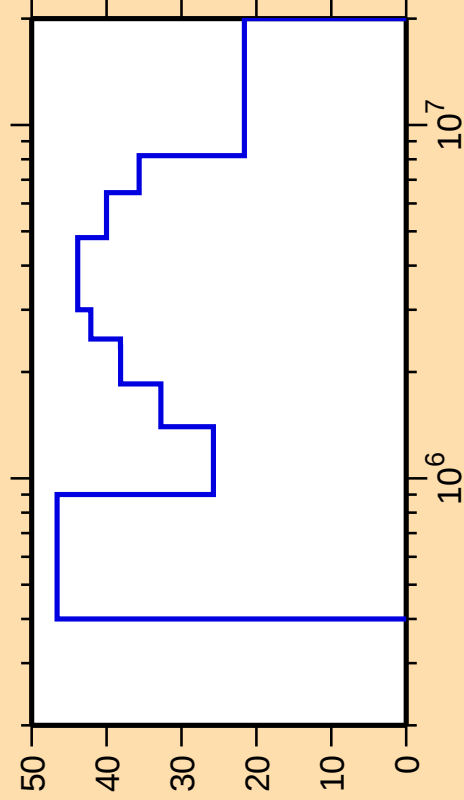
\Delta\sigma/\sigma vs. E for ^{185}\text{Au}(n,n_{\text{cont}})
