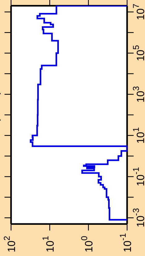
\Delta\sigma/\sigma vs. E for ^{186}\text{Au}(n,\text{el.})
