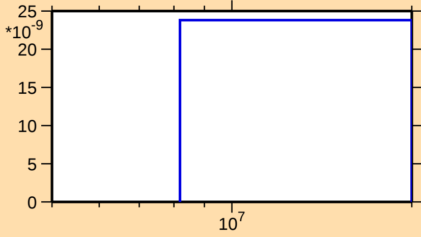
\sigma vs. E for ^{186}\text{Au}(\text{mt } 45)
