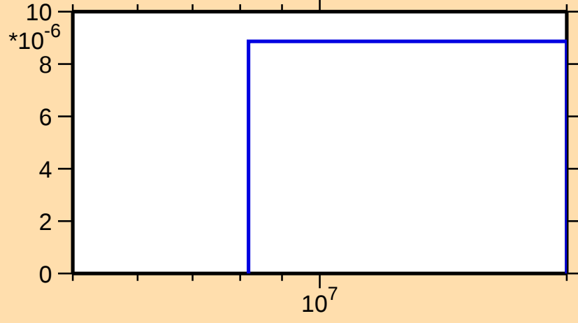
\sigma vs. E for ^{186}\text{Au}(n,3n)
