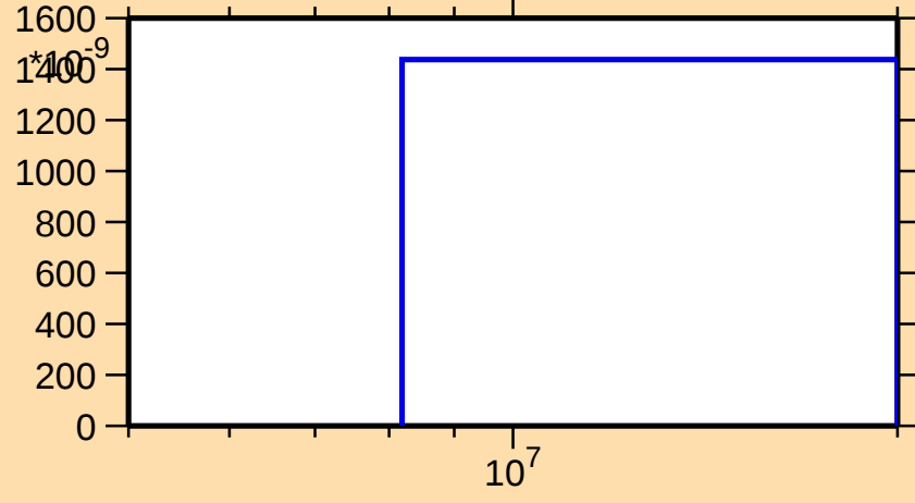
\sigma vs. E for ^{186}\text{Au}(n,\text{nd})
