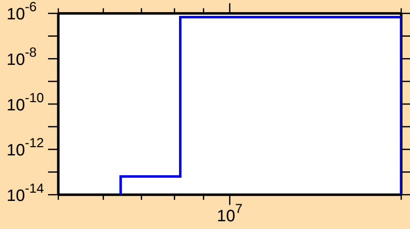
\sigma vs. E for ^{186}\text{Au}(n,\text{He}3)
