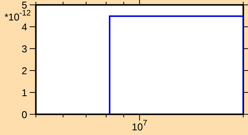
\sigma vs. E for ^{186}\text{Au}(\text{mt } 34)
