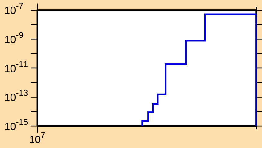
\sigma vs. E for ^{187}\text{Au}(n,nt)
