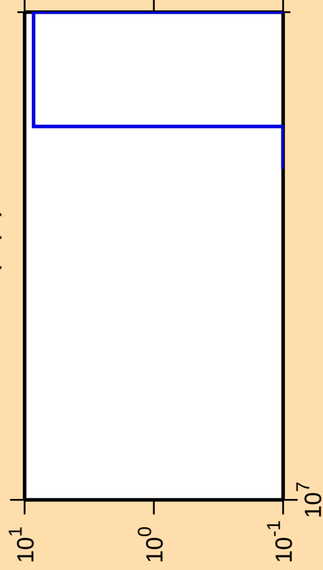
\Delta\sigma/\sigma vs. E for ^{187}\text{Au}(n,\text{pt})
