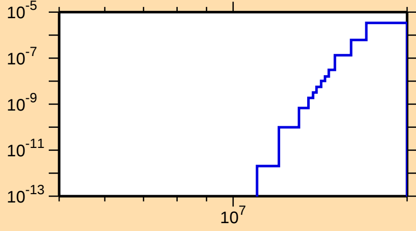
\sigma vs. E for ^{187}\text{Au}(n,2n\alpha)
