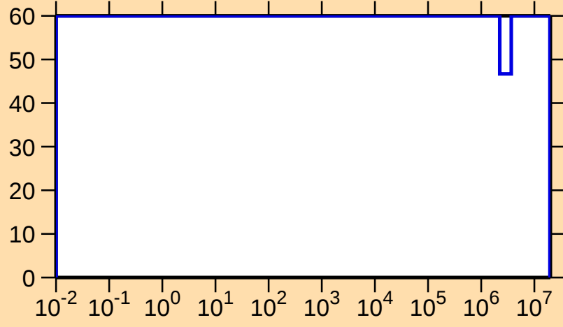
\Delta\sigma/\sigma vs. E for ^{187}\text{Au}(n,p)
