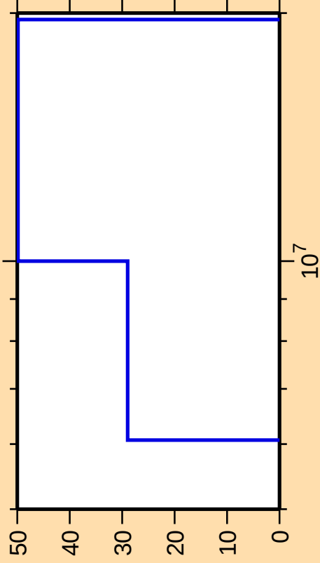
\Delta\sigma/\sigma vs. E for ^{187}\text{Au}(n,n\text{cont.})
