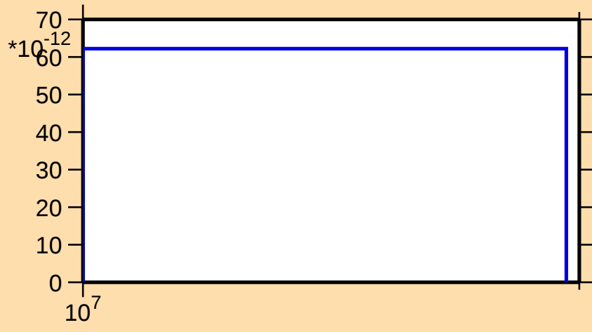
\sigma vs. E for ^{187}\text{Au}(\text{mt117})
