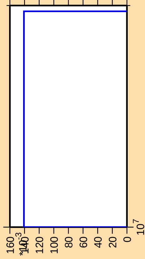
\Delta\sigma/\sigma vs. E for ^{187}\text{Au}(\text{mt } 34)
