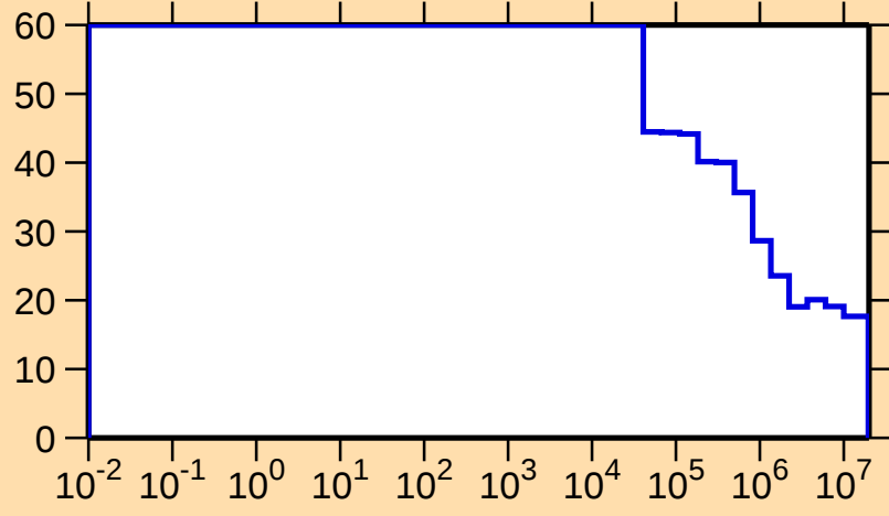
\Delta\sigma/\sigma vs. E for ^{187}\text{Au}(n,\text{nonel.})
