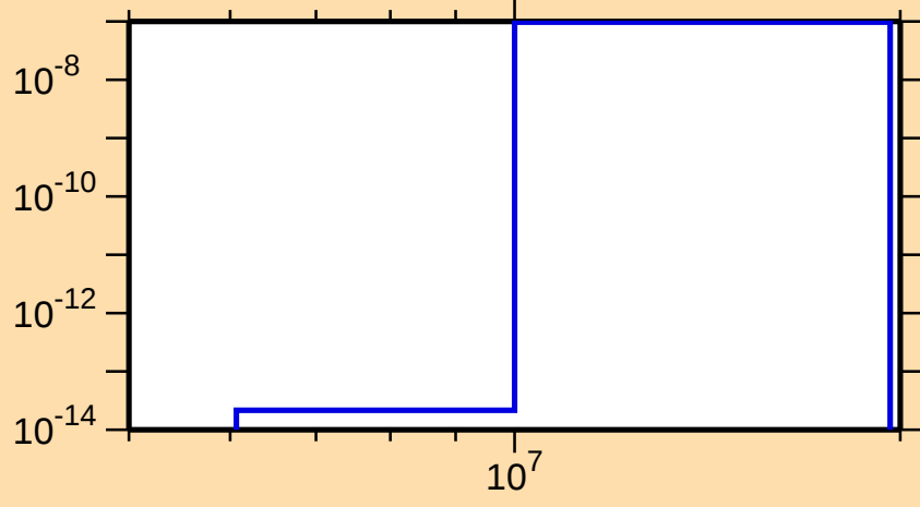
\sigma vs. E for ^{187}\text{Au}(n,\text{He3})
