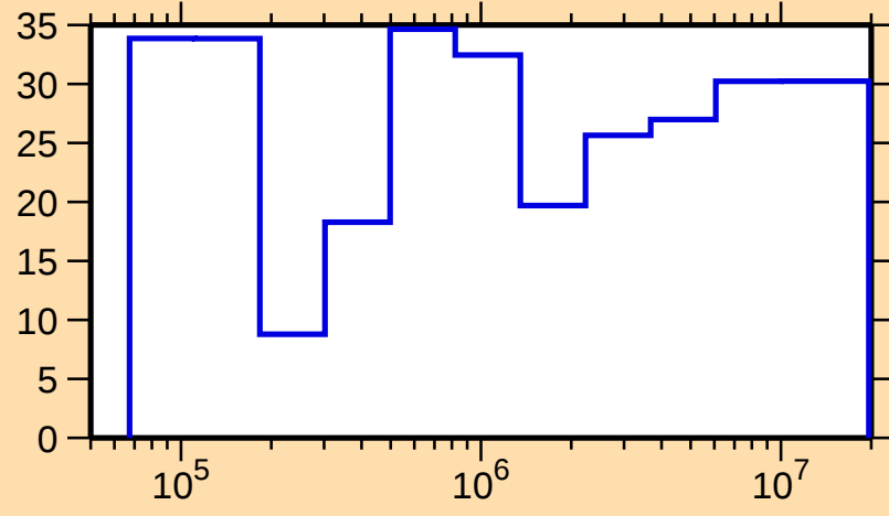
\Delta\sigma/\sigma vs. E for ^{187}\text{Au}(n,\text{tot.})
