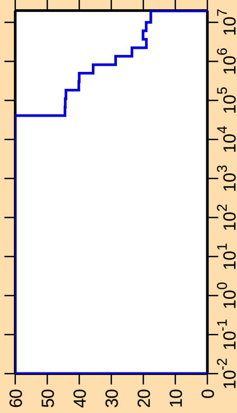
\Delta\sigma/\sigma vs. E for ^{187}\text{Au}(n,\text{nonel.})
