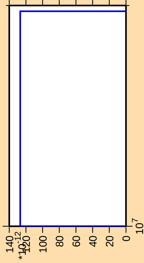
\Delta\sigma/\sigma vs. E for ^{187}\text{Au}(\text{mt } 42)
