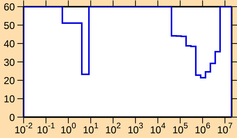
\Delta\sigma/\sigma vs. E for ^{187}\text{Au}(n,\gamma)
