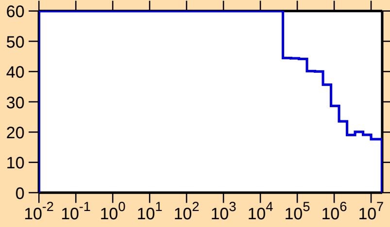
\Delta\sigma/\sigma vs. E for ^{187}\text{Au}(n,\text{nonel.})
