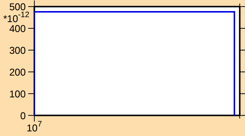
\sigma vs. E for ^{187}\text{Au}(n,nt)
