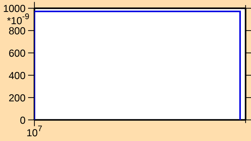
\sigma vs. E for ^{187}\text{Au}(n,2np)
