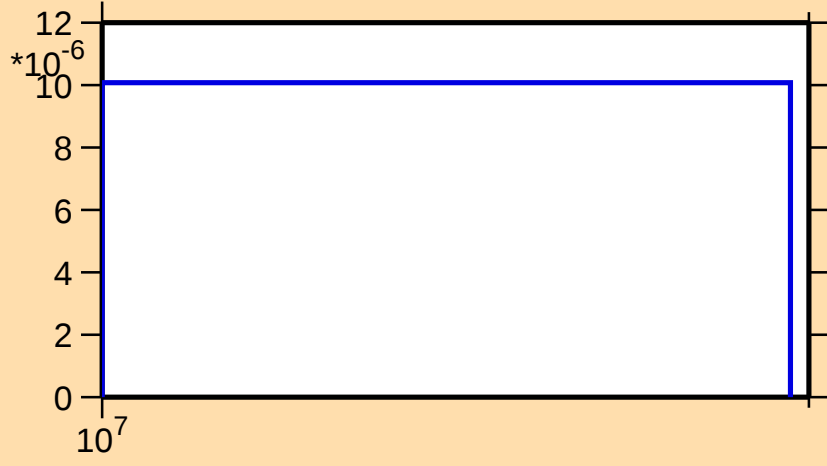
\sigma vs. E for ^{187}\text{Au}(n,3n)
