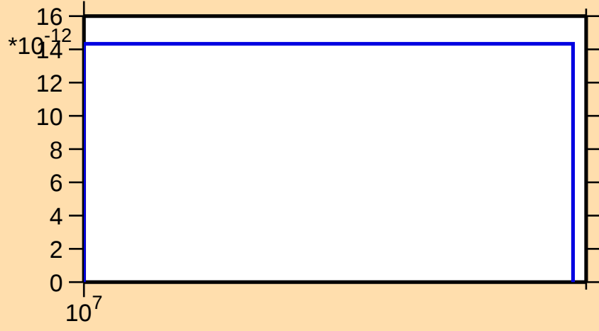
\sigma vs. E for ^{187}\text{Au}(n,\text{pd})
