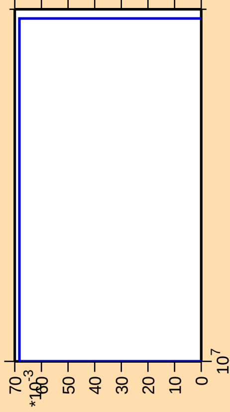
\Delta\sigma/\sigma vs. E for ^{187}\text{Au}(n,\text{pt})
