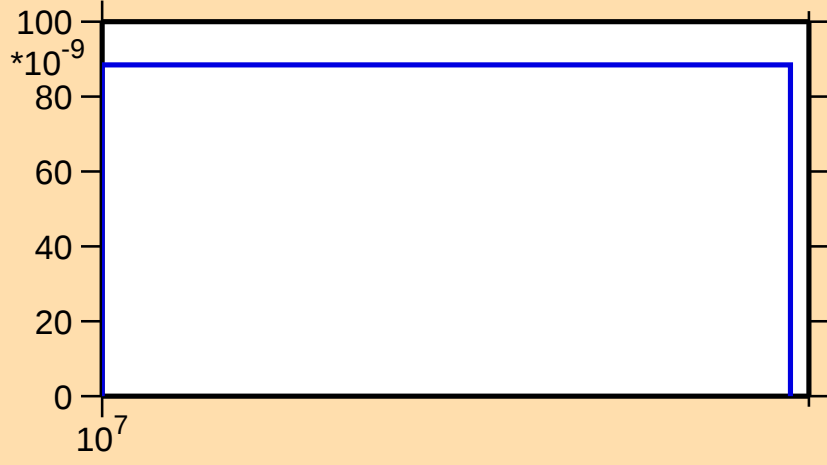
\sigma vs. E for ^{187}\text{Au}(n,2n\alpha)
