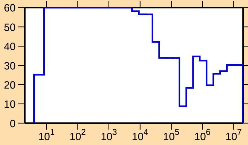
\Delta\sigma/\sigma vs. E for ^{187}\text{Au}(n,\text{tot.})
