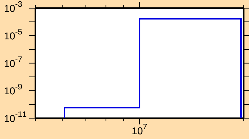
\sigma vs. E for ^{187}\text{Au}(n,t)
