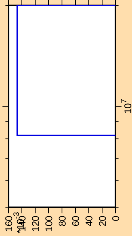
\Delta\sigma/\sigma vs. E for ^{187}\text{Au}(\text{mt } 34)
