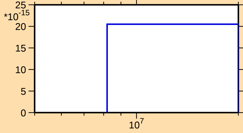
\sigma vs. E for ^{187}\text{Au}(n,\text{pt})
