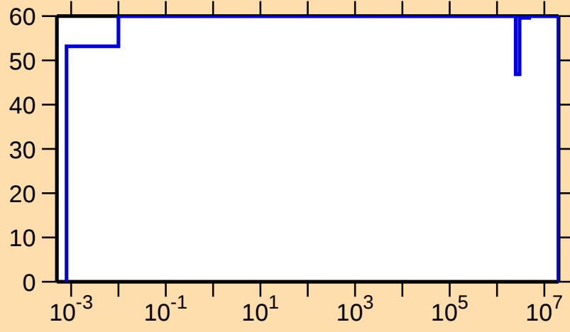
\Delta\sigma/\sigma vs. E for ^{187}\text{Au}(n,p)
