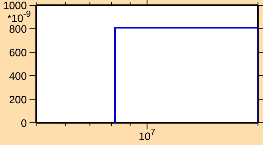
\sigma vs. E for ^{187}\text{Au}(n,2np)
