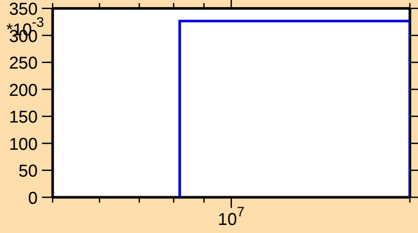
\sigma vs. E for ^{187}\text{Au}(n,2n)
