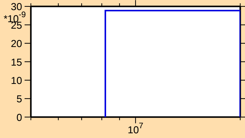
\sigma vs. E for ^{187}\text{Au}(n,\text{nd})
