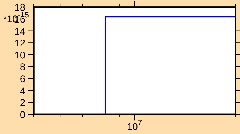
\sigma vs. E for ^{187}\text{Au}(\text{mt } 34)
