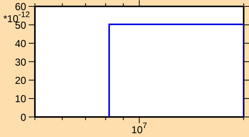
\sigma vs. E for ^{187}\text{Au}(\text{mt117})
