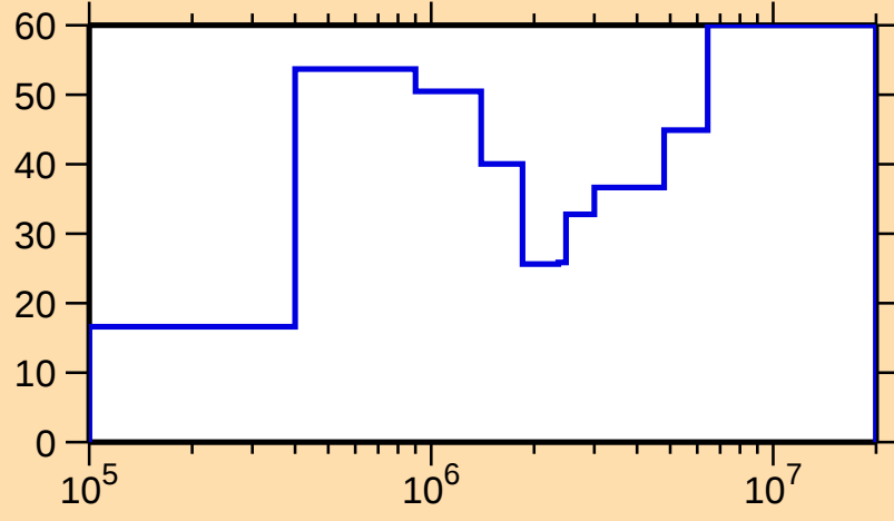
\Delta\sigma/\sigma vs. E for ^{187}\text{Au}(n,\text{el.})
