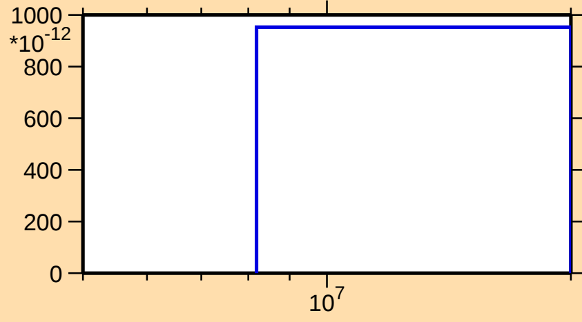
\sigma vs. E for ^{187}\text{Au}(\text{mt } 45)
