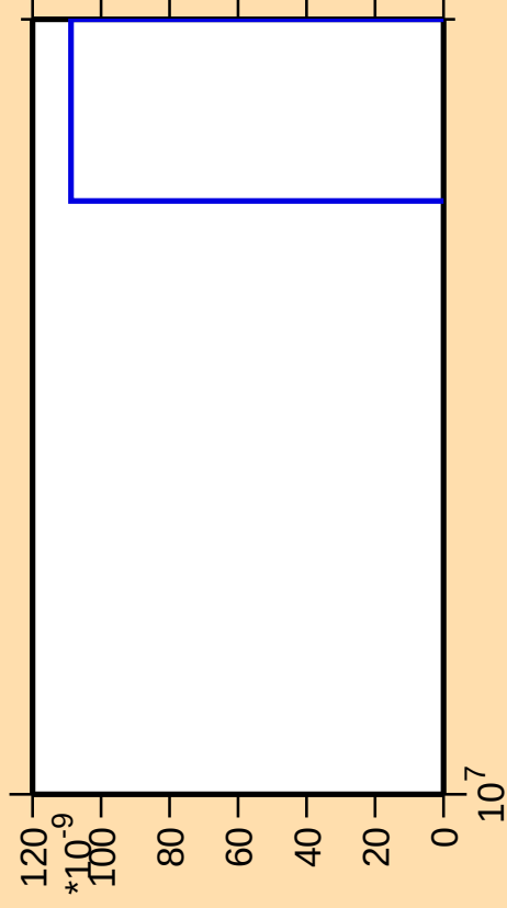
\Delta\sigma/\sigma vs. E for ^{190}\text{Au}(\text{mt } 42)
