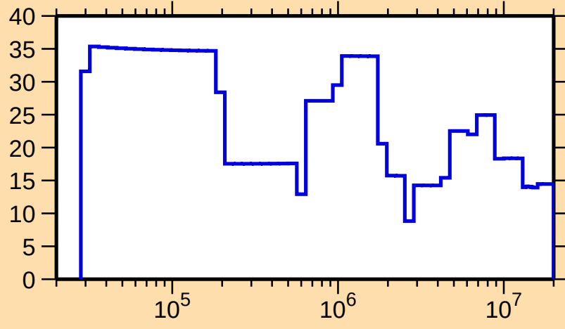
\Delta\sigma/\sigma vs. E for ^{190}\text{Au}(n,\text{el.})
