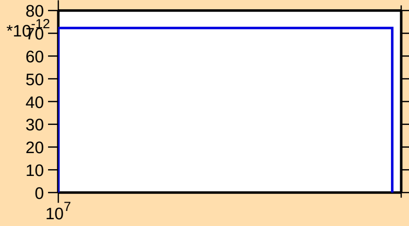
\sigma vs. E for ^{190}\text{Au}(\text{mt } 45)
