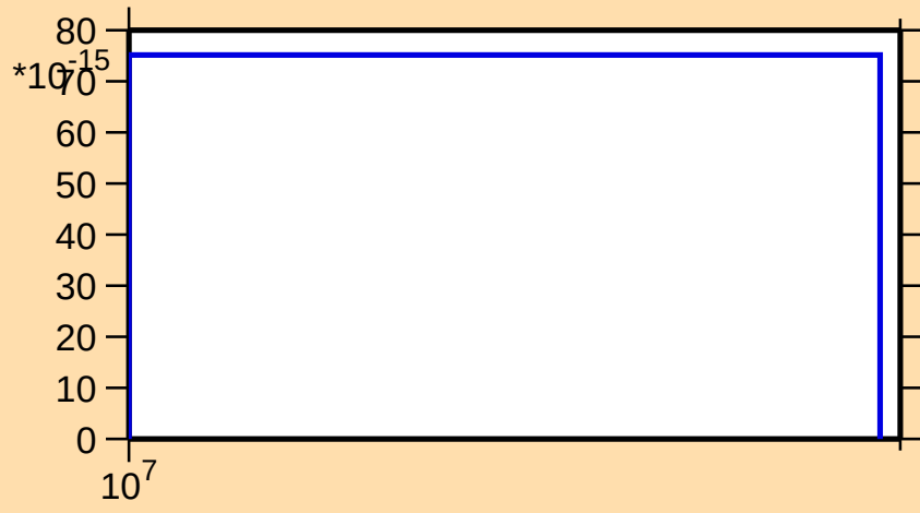
\sigma vs. E for ^{190}\text{Au}(\text{mt } 34)
