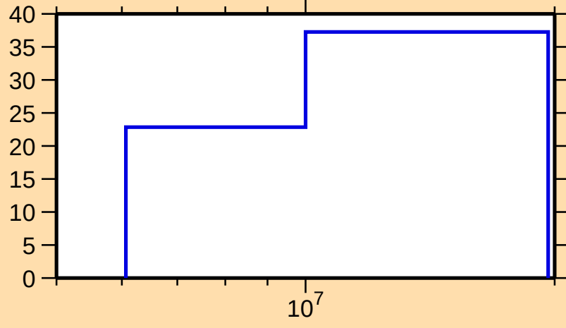
\Delta\sigma/\sigma vs. E for ^{190}\text{Au}(n,\text{inel.})
