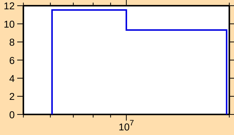
\Delta\sigma/\sigma vs. E for ^{190}\text{Au}(n,\text{tot.})
