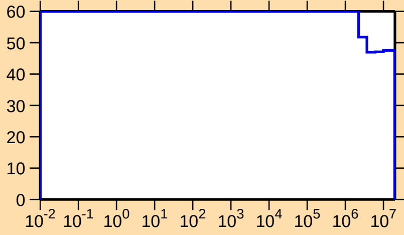
\Delta\sigma/\sigma vs. E for ^{190}\text{Au}(n,p)
