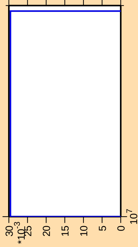
\Delta\sigma/\sigma vs. E for ^{190}\text{Au}(n,3n\alpha)
