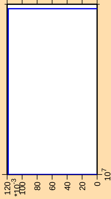
\Delta\sigma/\sigma vs. E for ^{190}\text{Au}(n,\text{pt})
