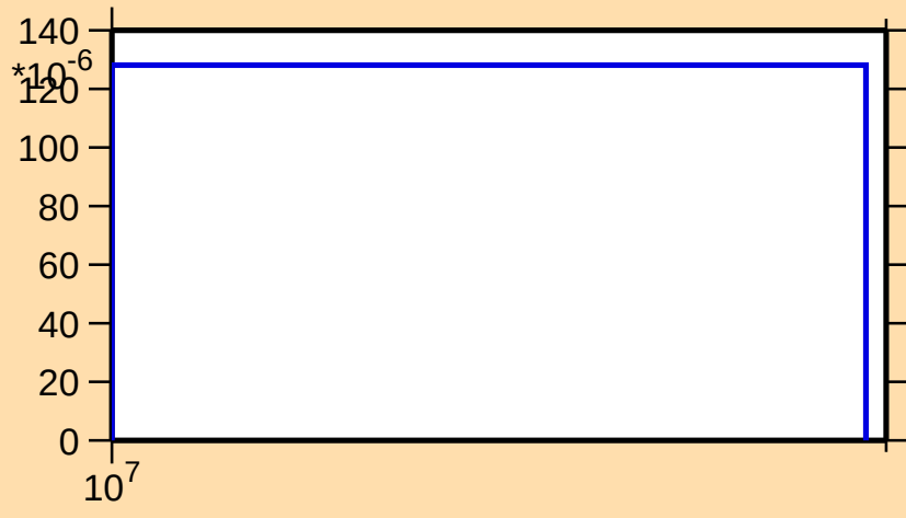
\sigma vs. E for ^{190}\text{Au}(n,3n)
