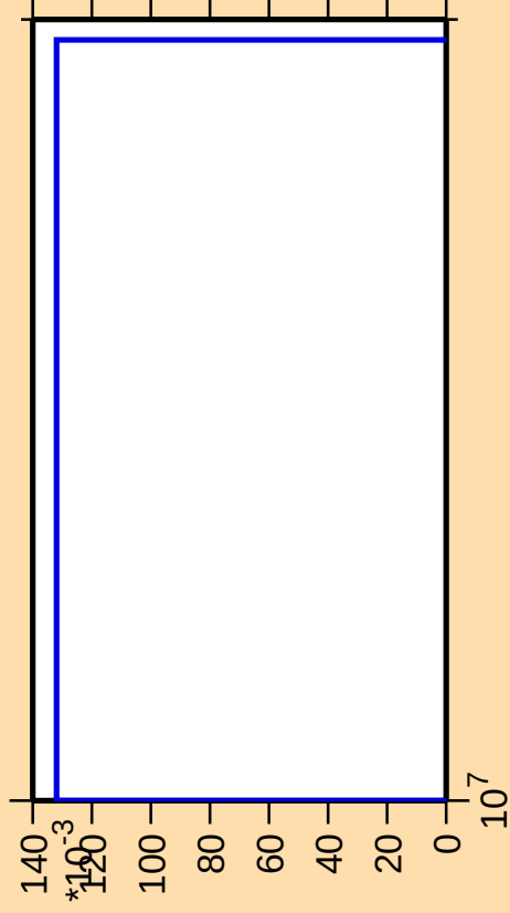
\Delta\sigma/\sigma vs. E for ^{190}\text{Au}(n,\text{pd})
