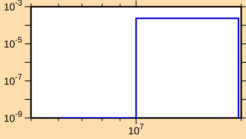
\sigma vs. E for ^{190}\text{Au}(n,t)
