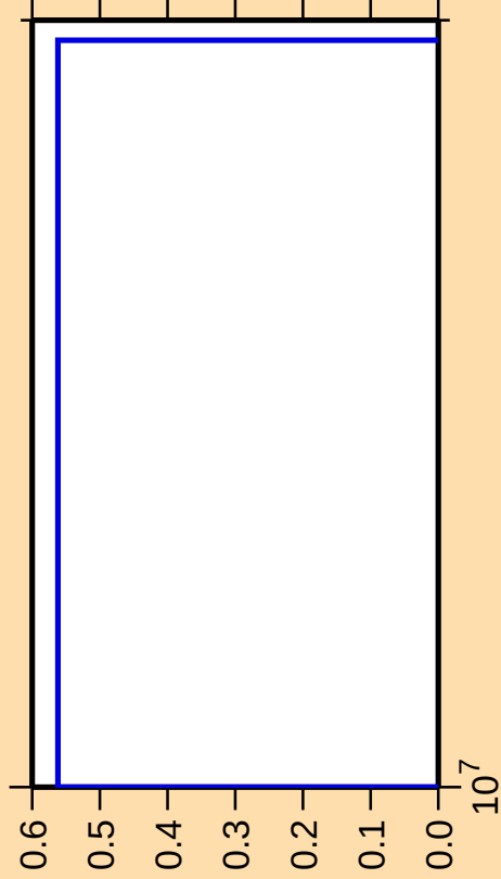
\Delta\sigma/\sigma vs. E for ^{190}\text{Au}(\text{mt } 34)
