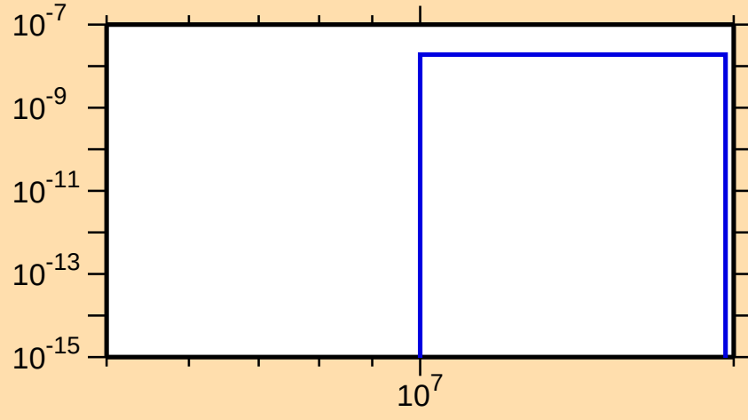
\sigma vs. E for ^{190}\text{Au}(n,\text{He}3)
