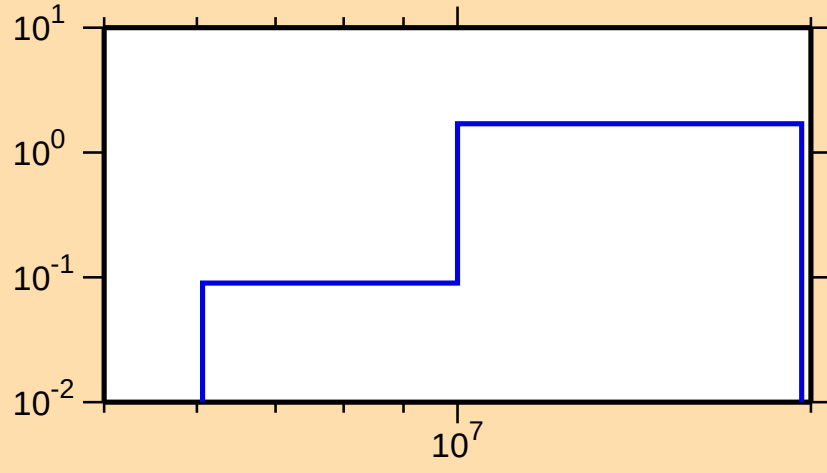
\sigma vs. E for ^{190}\text{Au}(n,2n)
