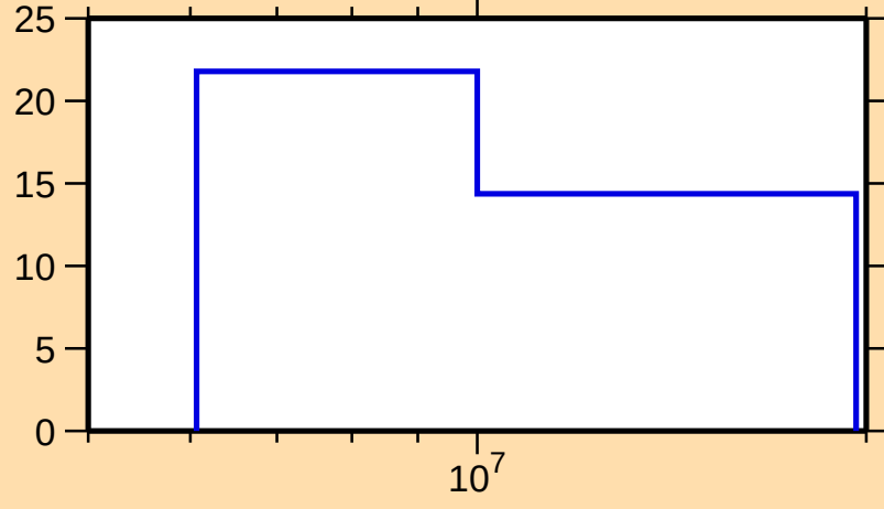
\Delta\sigma/\sigma vs. E for ^{190}\text{Au}(n,\text{el.})
