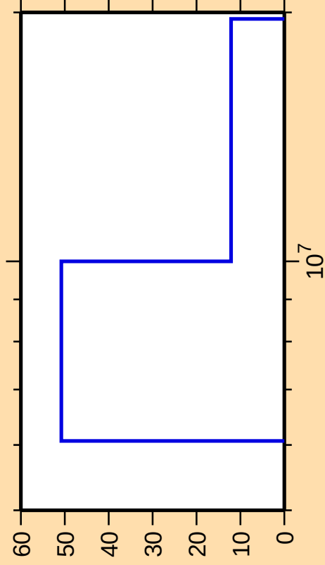
\Delta\sigma/\sigma vs. E for ^{190}\text{Au}(n,2n)
