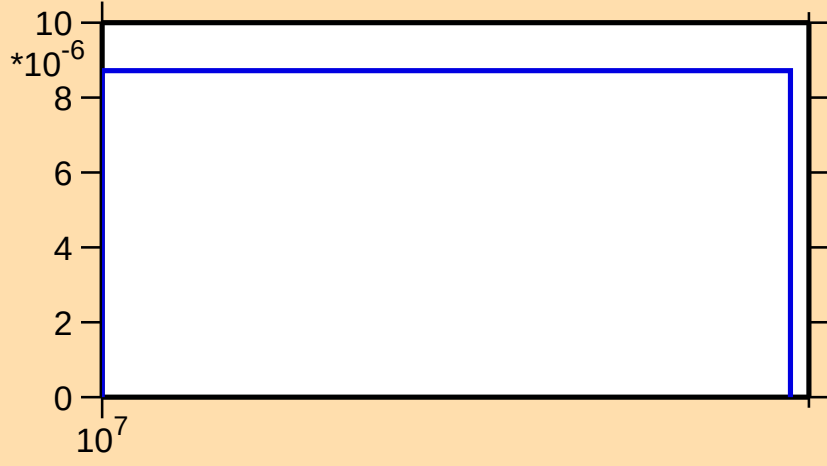
\sigma vs. E for ^{190}\text{Au}(n,2np)
