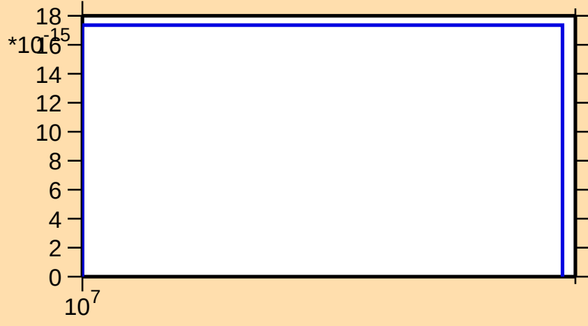
\sigma vs. E for ^{190}\text{Au}(n,\text{pt})
