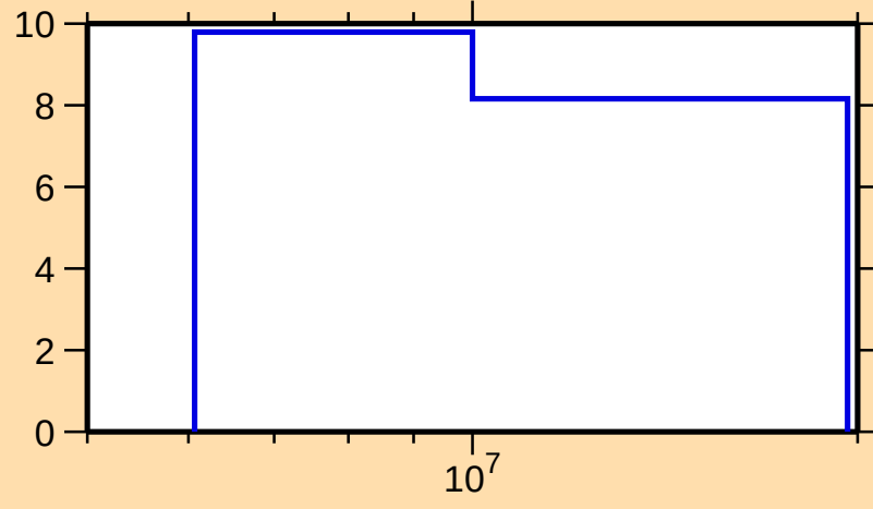
\Delta\sigma/\sigma vs. E for ^{190}\text{Au}(n,\text{nonel.})
