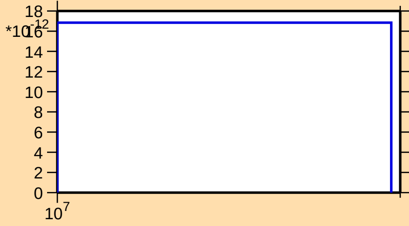
\sigma vs. E for ^{190}\text{Au}(\text{mt117})
