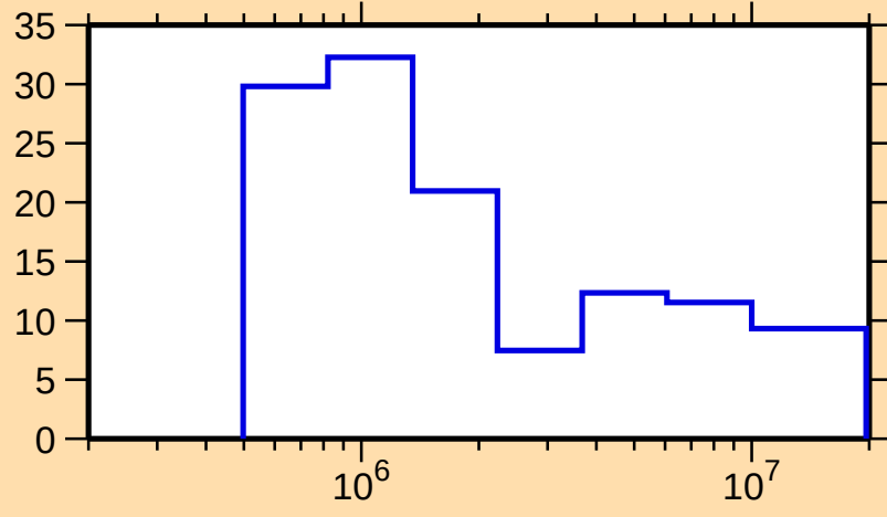
\Delta\sigma/\sigma vs. E for ^{190}\text{Au}(n,\text{tot.})
