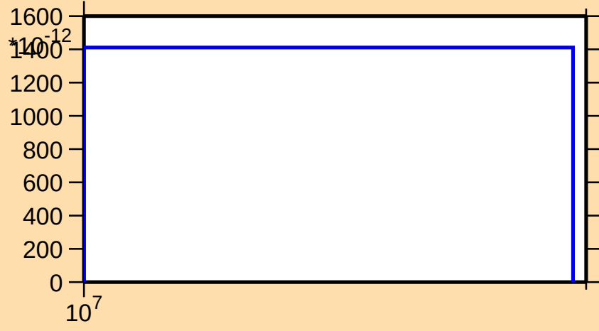
\sigma vs. E for ^{190}\text{Au}(n,nt)
