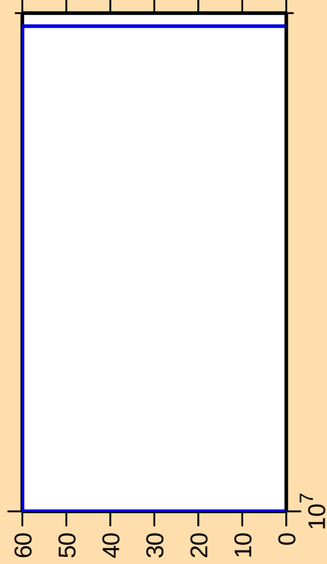
\Delta\sigma/\sigma vs. E for ^{190}\text{Au}(\text{mt } 45)
