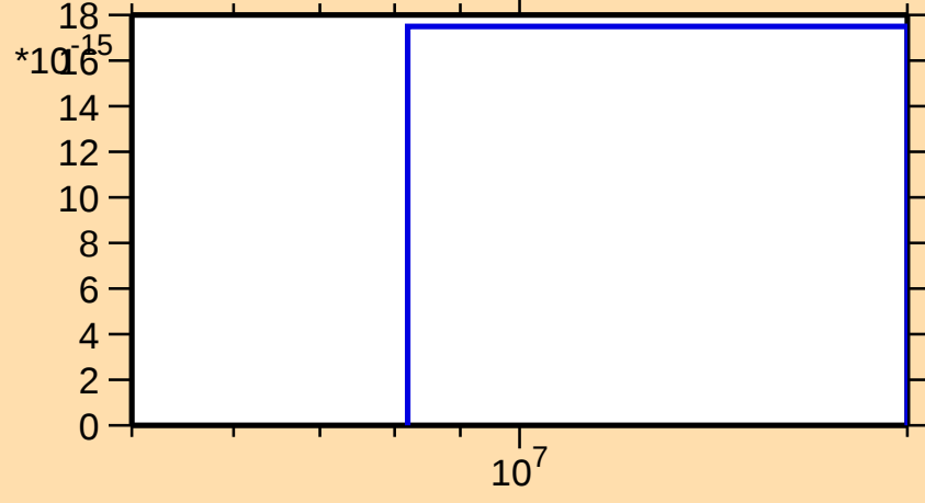
\sigma vs. E for ^{190}\text{Au}(n,pt)
