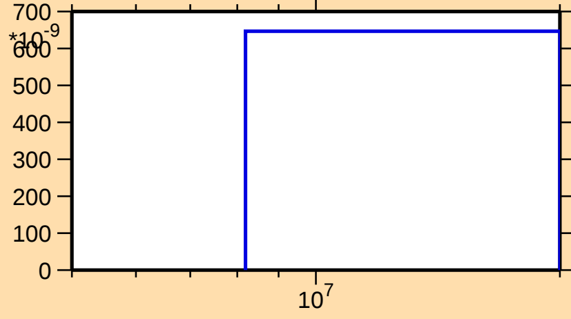
\sigma vs. E for ^{190}\text{Au}(n,\text{nd})
