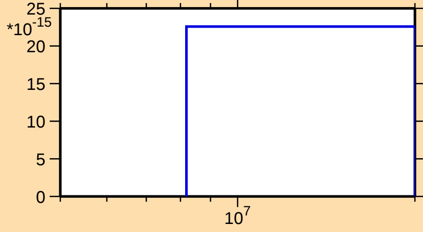
\sigma vs. E for ^{190}\text{Au}(n,\text{pd})
