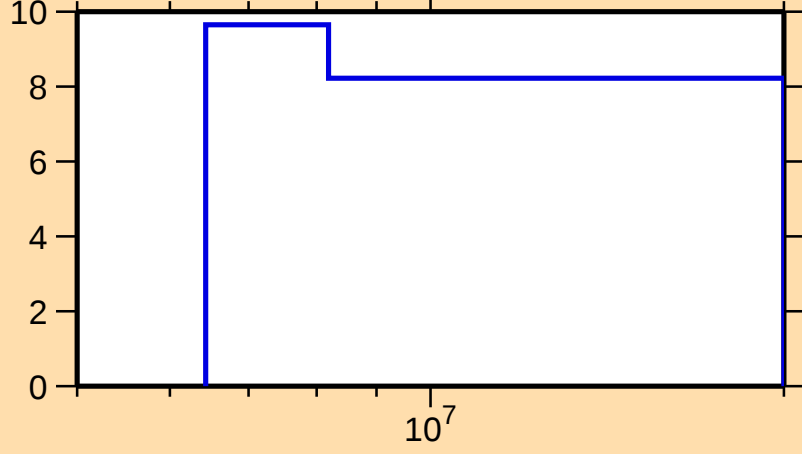
\Delta\sigma/\sigma vs. E for ^{190}\text{Au}(n,\text{nonel.})
