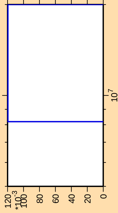
\Delta\sigma/\sigma vs. E for ^{190}\text{Au}(n,pt)
