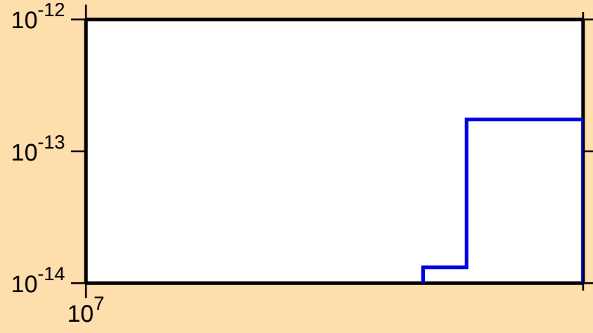
\sigma vs. E for ^{193}\text{Au}(\text{mt117})
