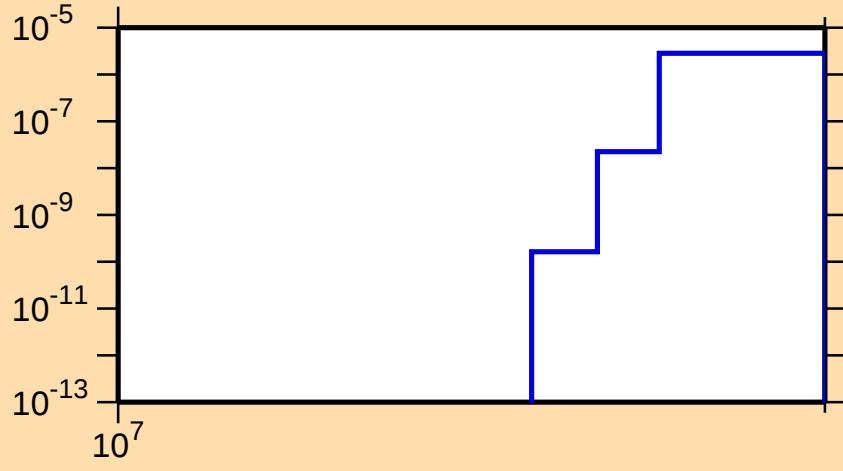
\sigma vs. E for ^{193}\text{Au}(n,2np)
