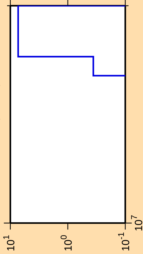
\Delta\sigma/\sigma vs. E for ^{193}\text{Au}(\text{mt } 45)
