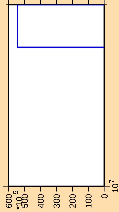
\Delta\sigma/\sigma vs. E for ^{193}\text{Au}(\text{mt } 42)
