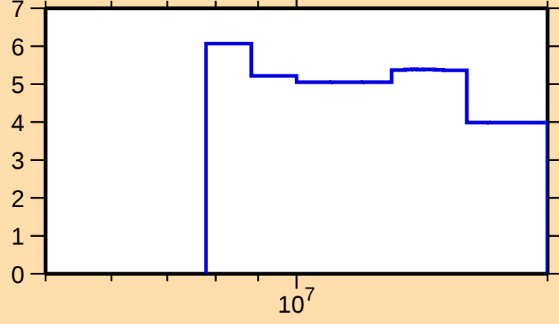
\Delta\sigma/\sigma vs. E for ^{193}\text{Au}(n,\text{nonel.})
