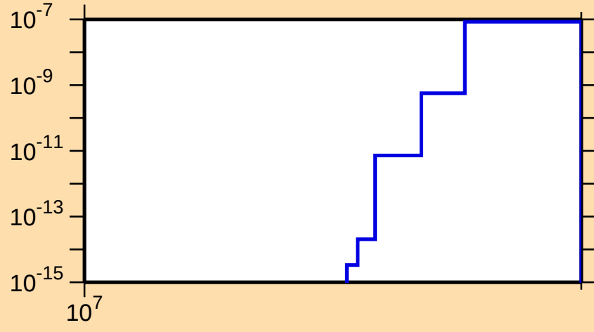
\sigma vs. E for ^{193}\text{Au}(n,nt)
