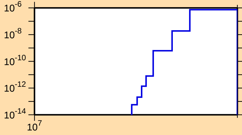
\sigma vs. E for ^{193}\text{Au}(n,\text{nd})
