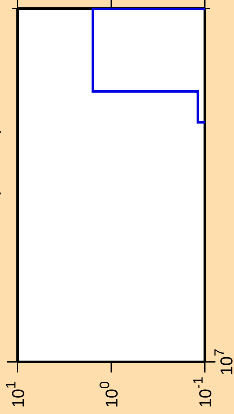
\Delta\sigma/\sigma vs. E for ^{193}\text{Au}(\text{mt117})
