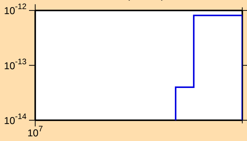
\sigma vs. E for ^{193}\text{Au}(\text{mt } 45)
