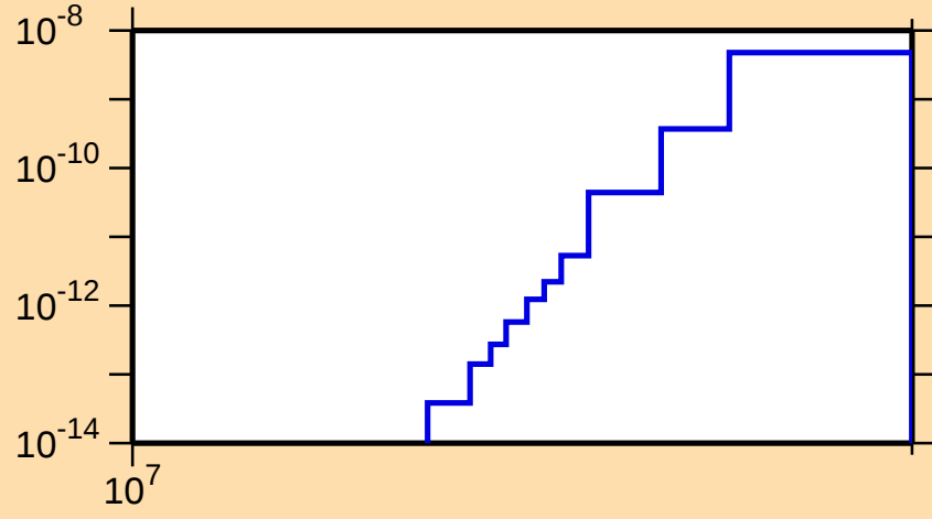
\sigma vs. E for ^{193}\text{Au}(n,\text{He3})
