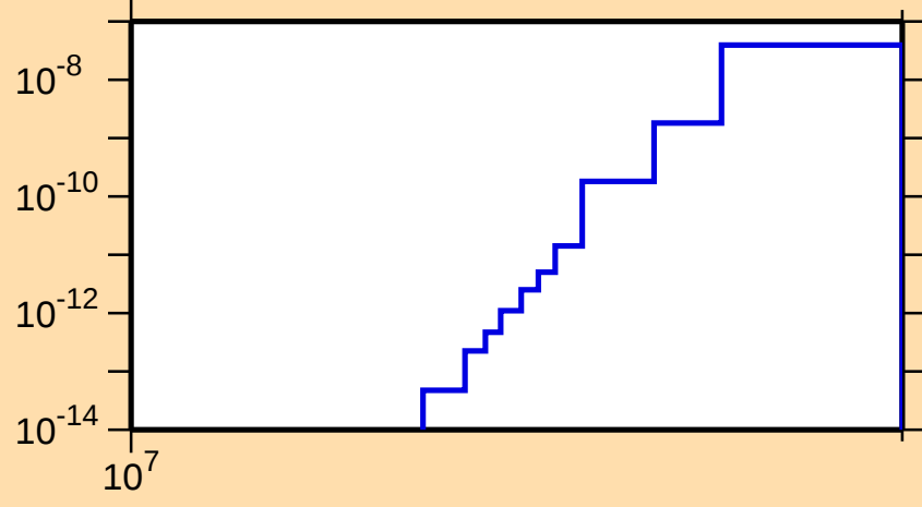
\sigma vs. E for ^{193}\text{Au}(n,2n\alpha)
