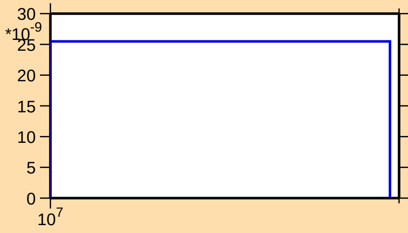
\sigma vs. E for ^{193}\text{Au}(n,2np)
