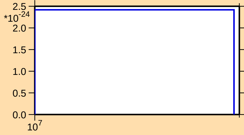
\sigma vs. E for ^{193}\text{Au}(\text{mt } 42)
