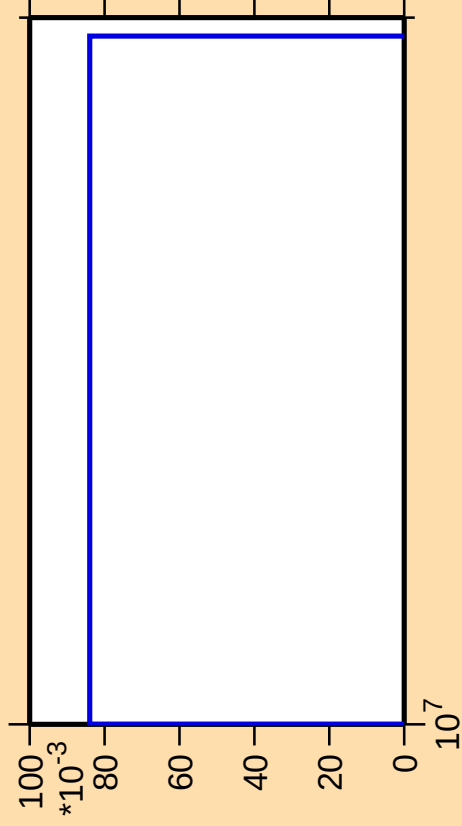
\Delta\sigma/\sigma vs. E for ^{193}\text{Au}(\text{mt } 45)
