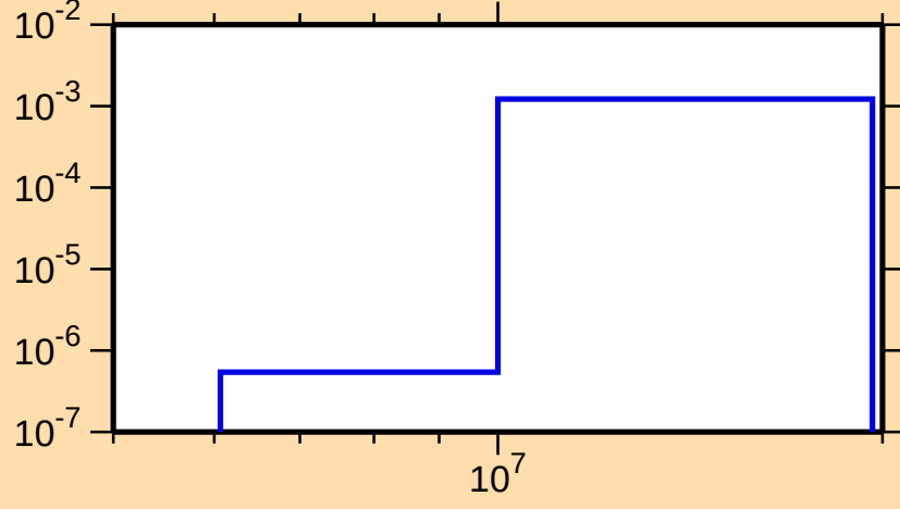
\sigma vs. E for ^{193}\text{Au}(n,np)
