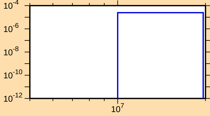
\sigma vs. E for ^{193}\text{Au}(n,t)
