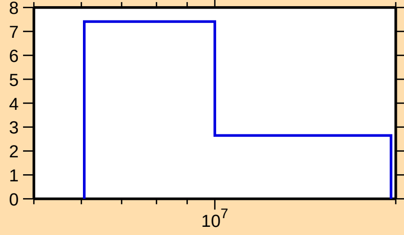
\Delta\sigma/\sigma vs. E for ^{193}\text{Au}(n,\text{tot.})
