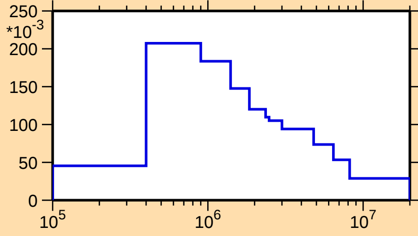
\sigma vs. E for ^{193}\text{Au}(n,n_2)
