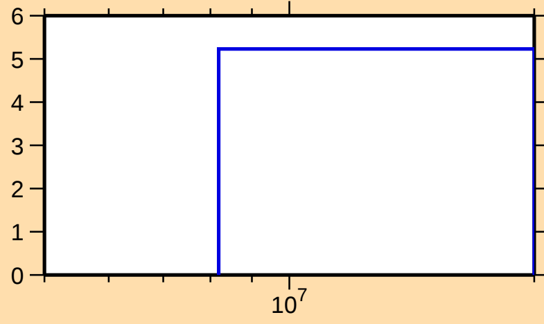
\Delta\sigma/\sigma vs. E for ^{193}\text{Au}(n,\text{nonel.})
