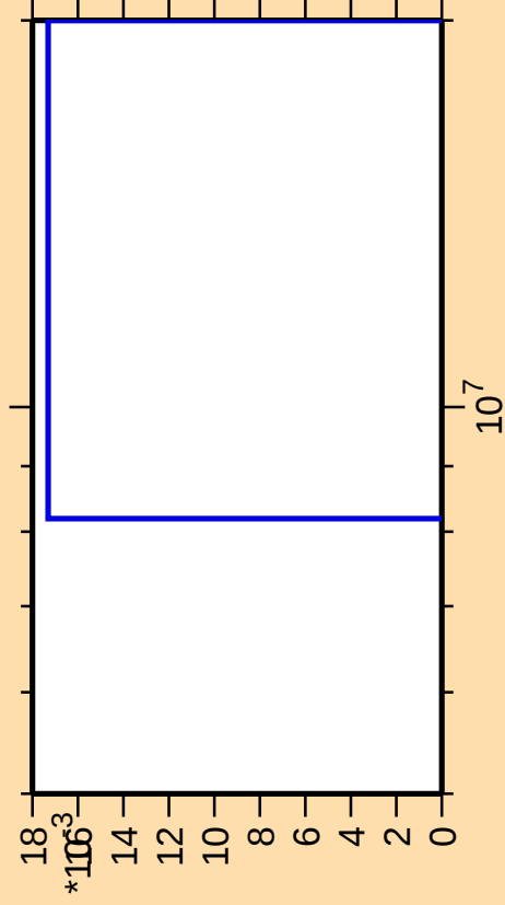
\Delta\sigma/\sigma vs. E for ^{193}\text{Au}(\text{mt117})
