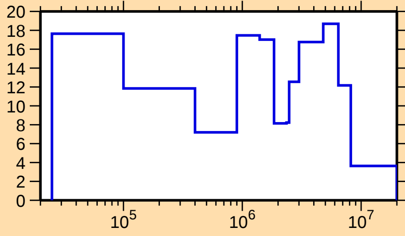
\Delta\sigma/\sigma vs. E for ^{193}\text{Au}(n,\text{el.})
