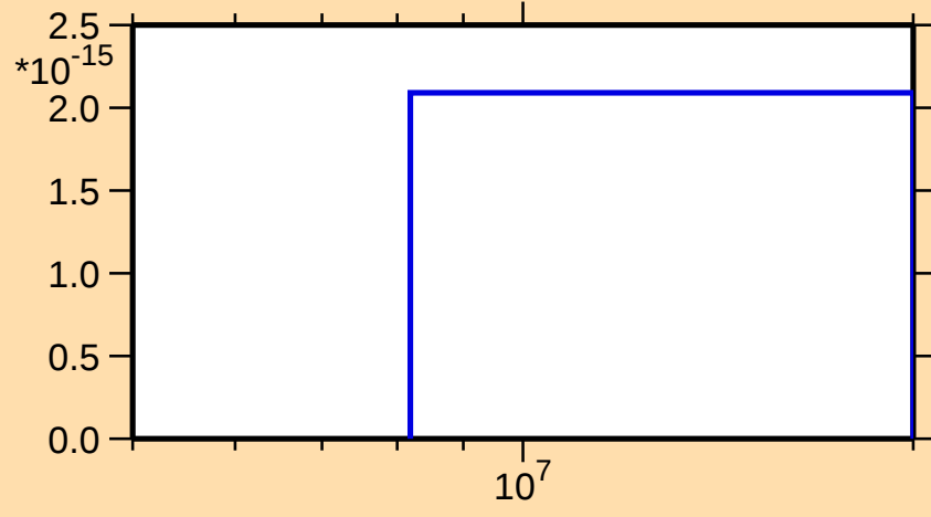
\sigma vs. E for ^{193}\text{Au}(\text{mt117})
