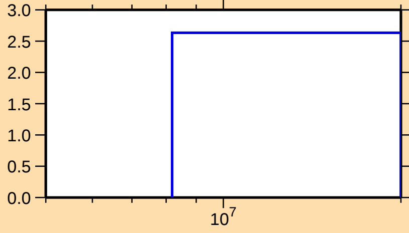
\Delta\sigma/\sigma vs. E for ^{193}\text{Au}(n,\text{tot.})
