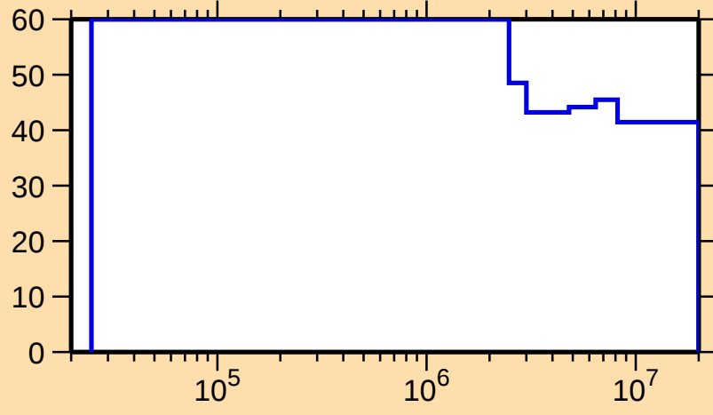
\Delta\sigma/\sigma vs. E for ^{193}\text{Au}(n,n_1)
