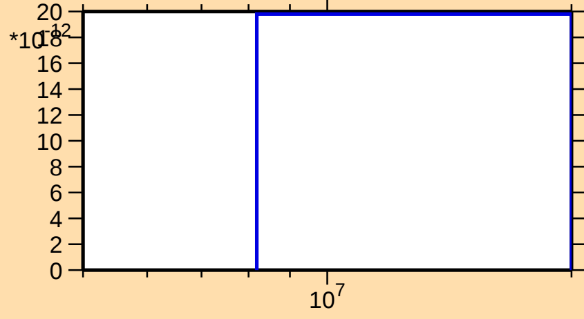
\sigma vs. E for ^{193}\text{Au}(n,p\alpha)
