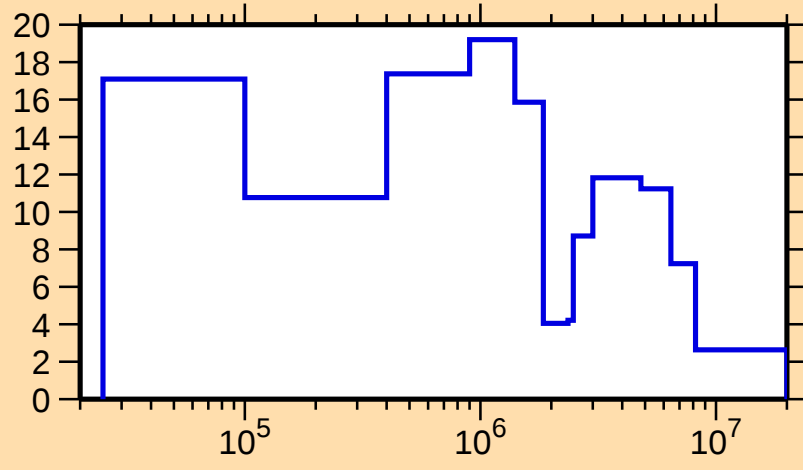
\Delta\sigma/\sigma vs. E for ^{193}\text{Au}(n,\text{tot.})
