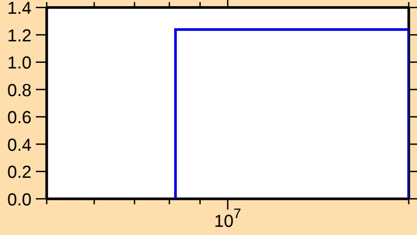
\sigma vs. E for ^{193}\text{Au}(n,2n)
