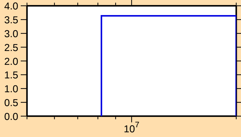
\Delta\sigma/\sigma vs. E for ^{193}\text{Au}(n,\text{el.})
