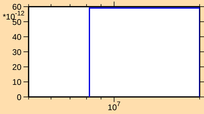
\sigma vs. E for ^{193}\text{Au}(n,\text{He}3)
