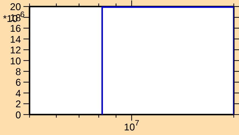
\sigma vs. E for ^{193}\text{Au}(n,t)
