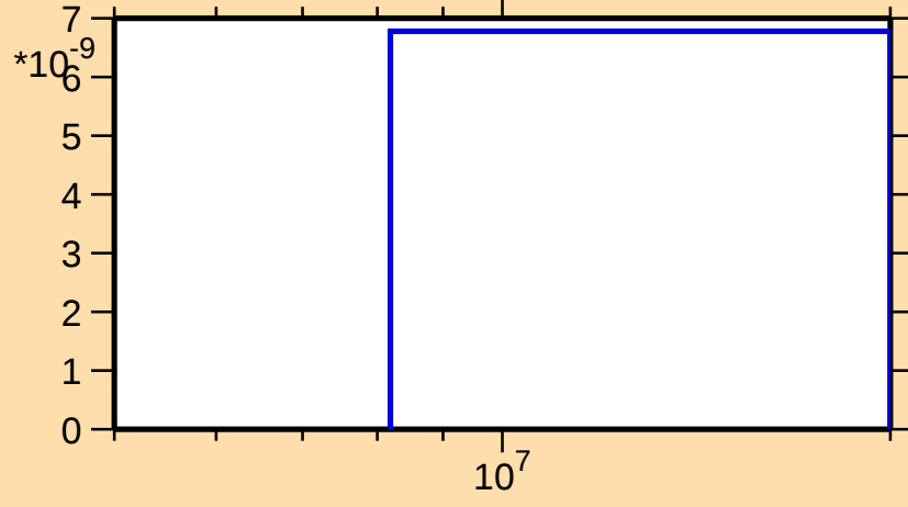
\sigma vs. E for ^{193}\text{Au}(n,\text{nd})
