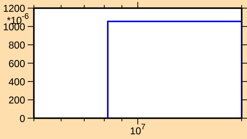
\sigma vs. E for ^{193}\text{Au}(n,3n)
