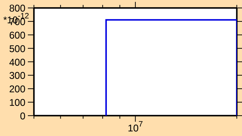
\sigma vs. E for ^{193}\text{Au}(n,nt)
