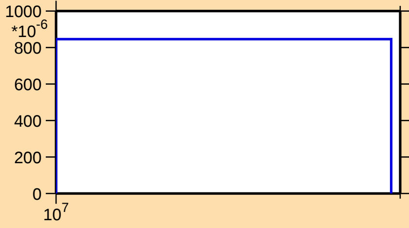
\sigma vs. E for ^{193}\text{Au}(n,3n)
