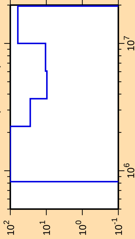
\Delta\sigma/\sigma vs. E for ^{193}\text{Au}(n,n\text{cont.})
