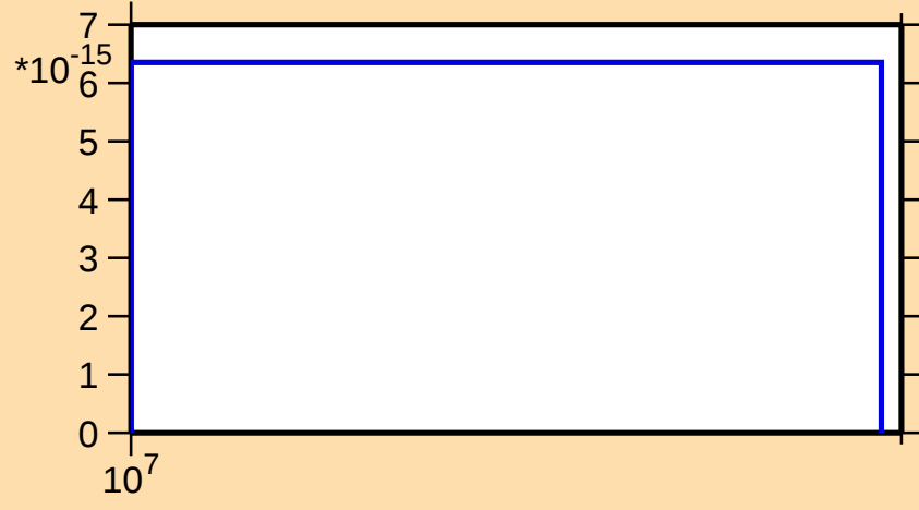
\sigma vs. E for ^{193}\text{Au}(\text{mt } 45)
