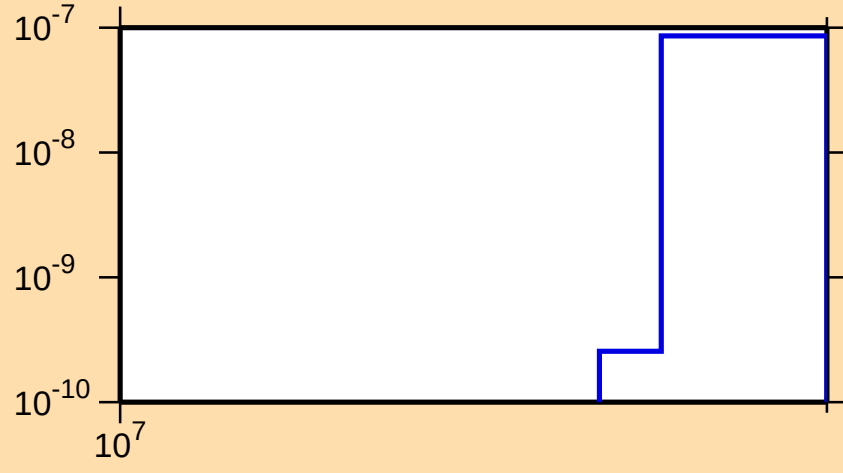
\sigma vs. E for ^{196}\text{Au}(n,nt)
