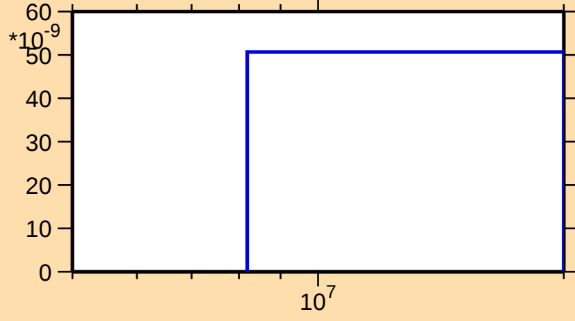
\sigma vs. E for ^{196}\text{Au}(n,\text{nd})
