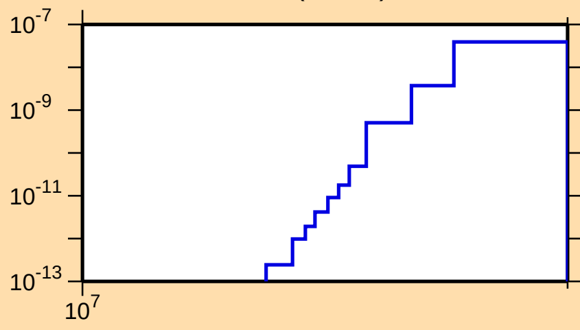
\sigma vs. E for ^{196}\text{Au}(n,2n\alpha)
