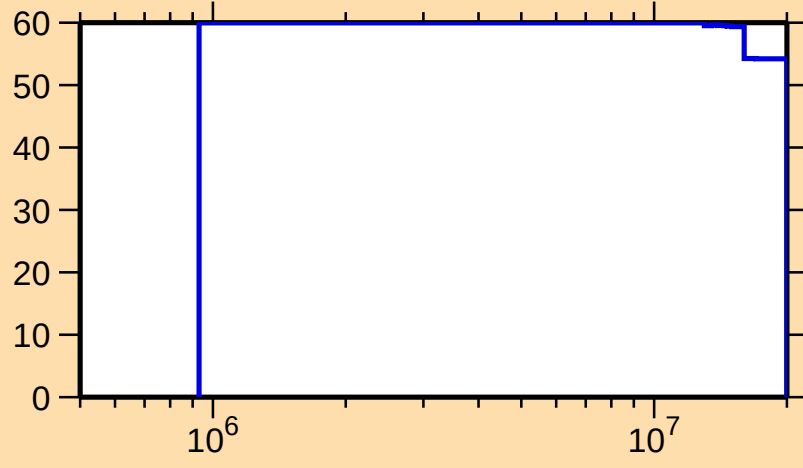
\Delta\sigma/\sigma vs. E for ^{196}\text{Au}(n,p)
