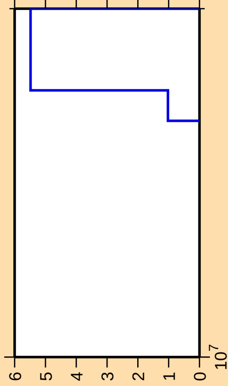
\Delta\sigma/\sigma vs. E for ^{196}\text{Au}(n,p\alpha)
