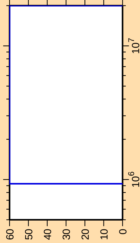
\Delta\sigma/\sigma vs. E for ^{196}\text{Au}(n,\alpha)
