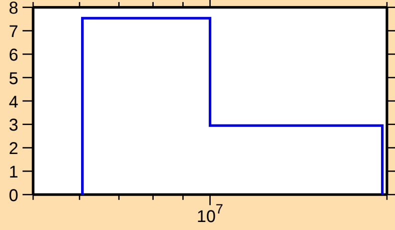
\Delta\sigma/\sigma vs. E for ^{196}\text{Au}(n,\text{tot.})
