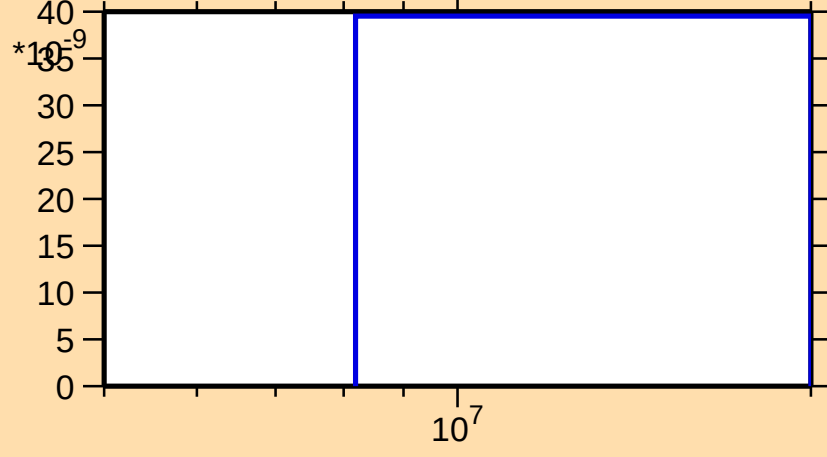
\sigma vs. E for ^{196}\text{Au}(n,nd)
