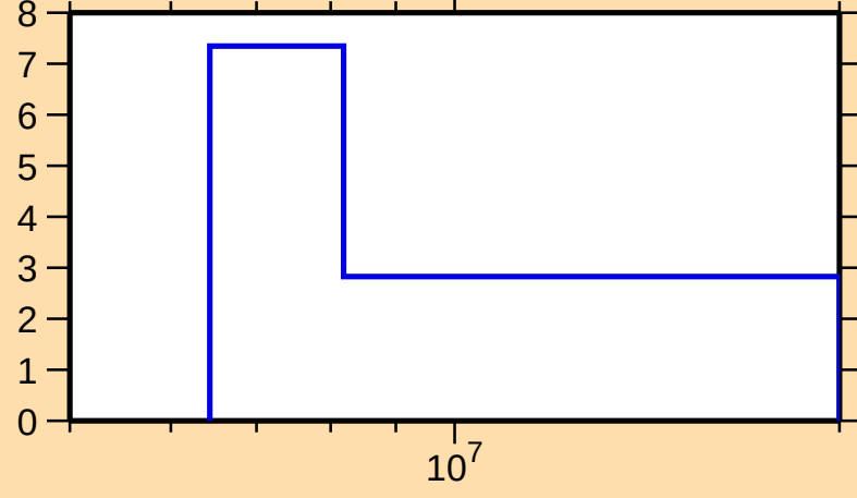
\Delta\sigma/\sigma vs. E for ^{196}\text{Au}(n,\text{tot.})
