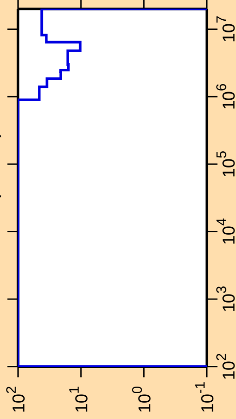
\Delta\sigma/\sigma vs. E for ^{196}\text{Au}(n,\text{inel.})
