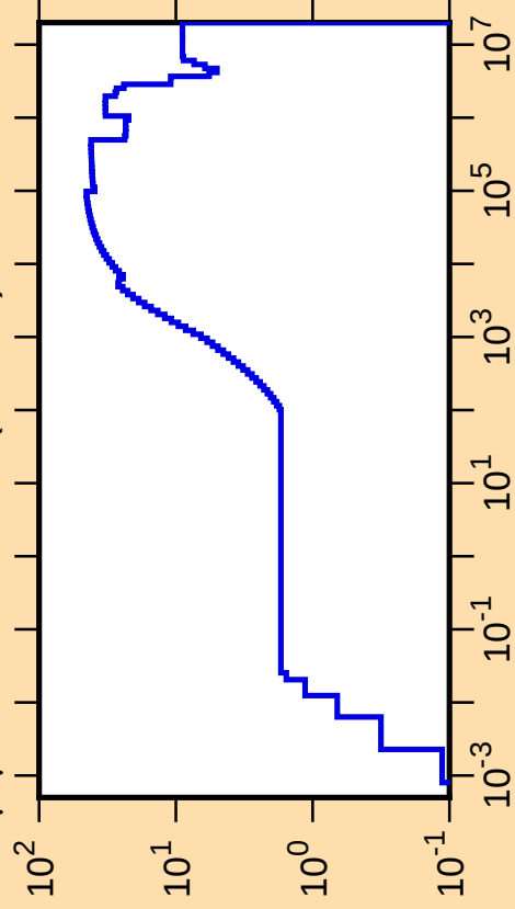
\Delta\mu/\mu vs. E for ^{199}\text{Au}(\text{mt251})
