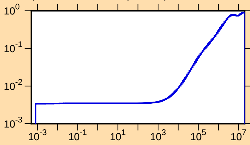
\mu vs. E for ^{199}\text{Au}(\text{mt251})
