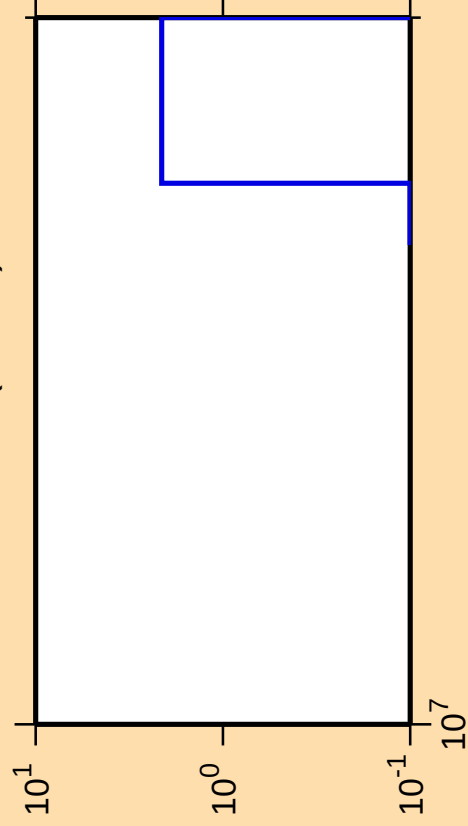
\Delta\sigma/\sigma vs. E for ^{199}\text{Au}(n,\text{He3})
