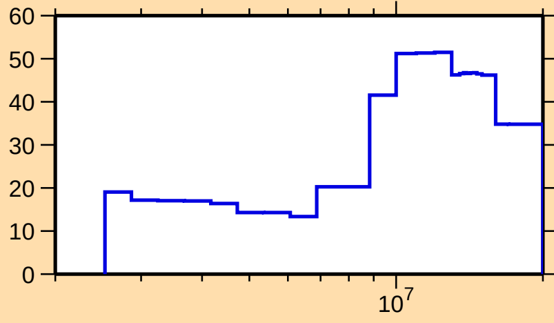
\Delta\sigma/\sigma vs. E for ^{199}\text{Au}(n,n\text{cont.})
