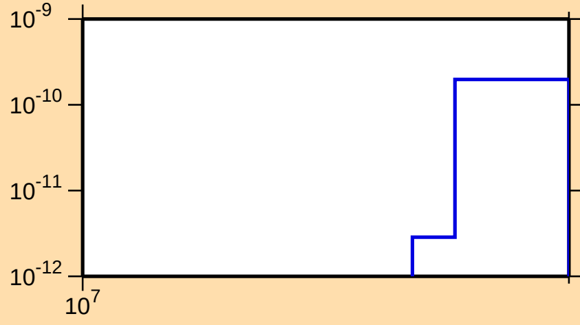
\sigma vs. E for ^{199}\text{Au}(n,2n\alpha)
