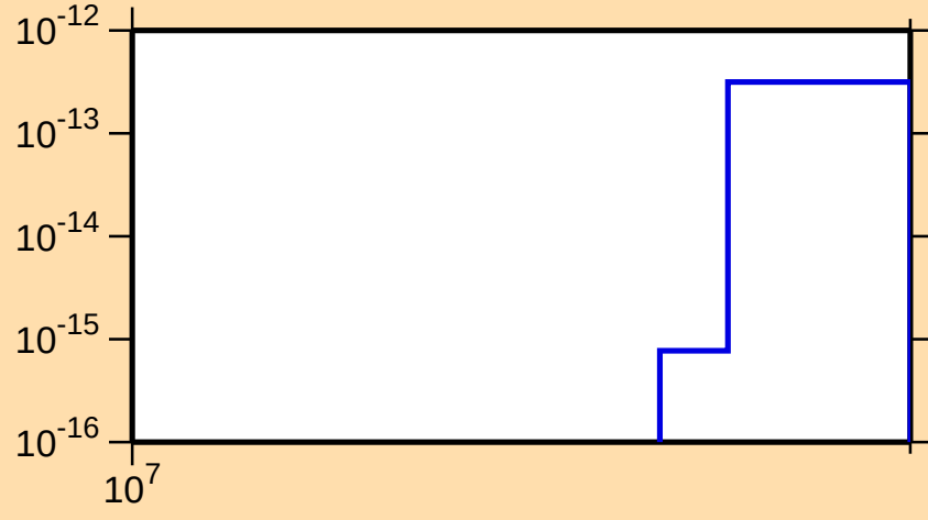
\sigma vs. E for ^{199}\text{Au}(n,\text{He3})
