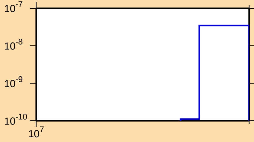
\sigma vs. E for ^{199}\text{Au}(n,nt)
