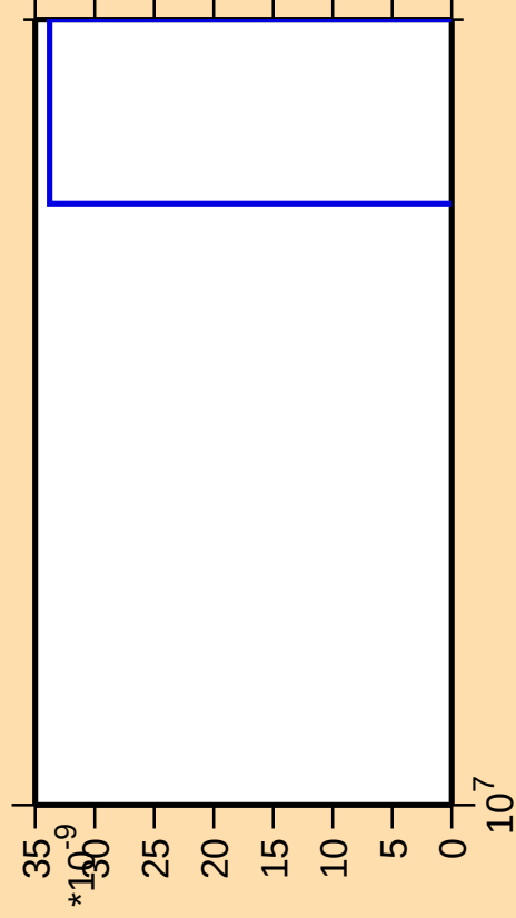
\Delta\sigma/\sigma vs. E for ^{199}\text{Au}(\text{mt } 42)
