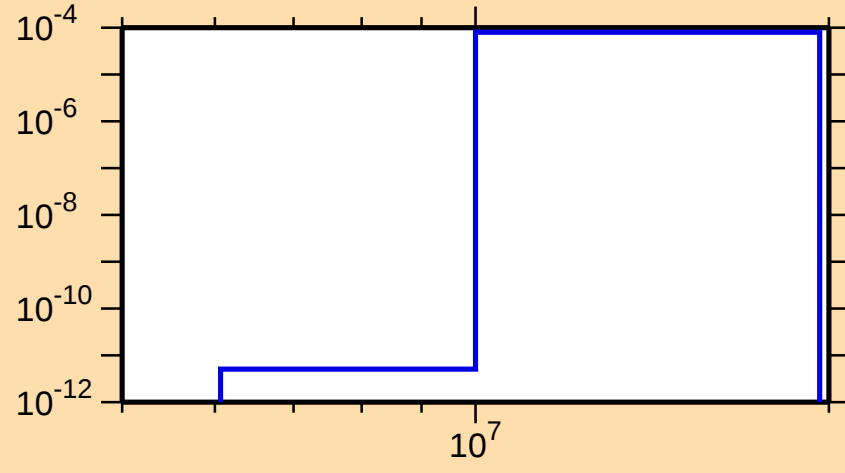
\sigma vs. E for ^{199}\text{Au}(n,np)
