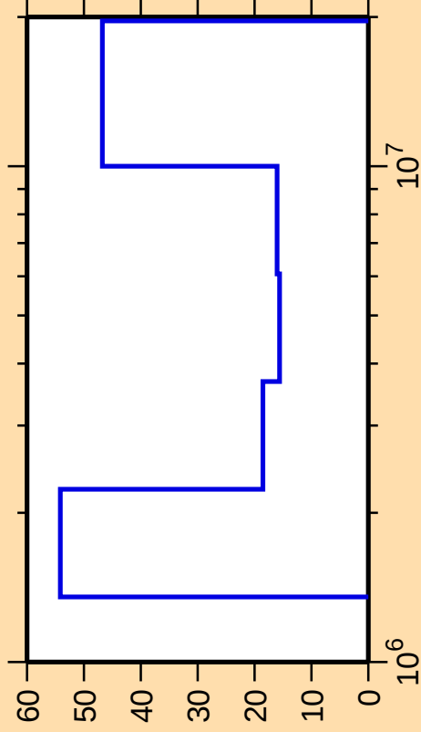
\Delta\sigma/\sigma vs. E for ^{199}\text{Au}(n,n\text{cont.})
