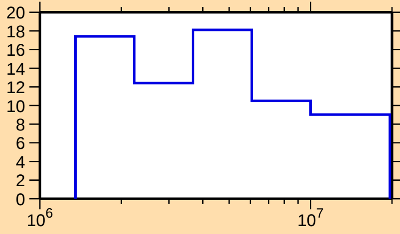
\Delta\sigma/\sigma vs. E for ^{199}\text{Au}(n,\text{el.})
