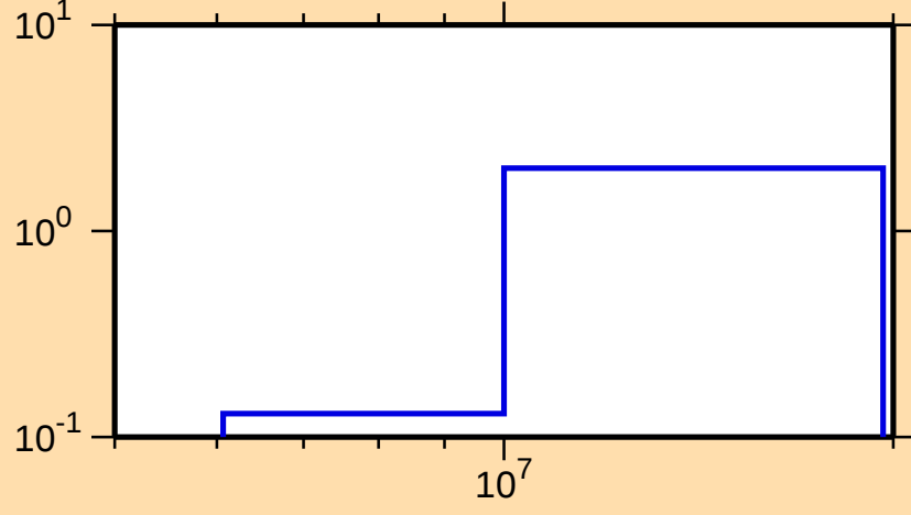
\sigma vs. E for ^{199}\text{Au}(n,2n)
