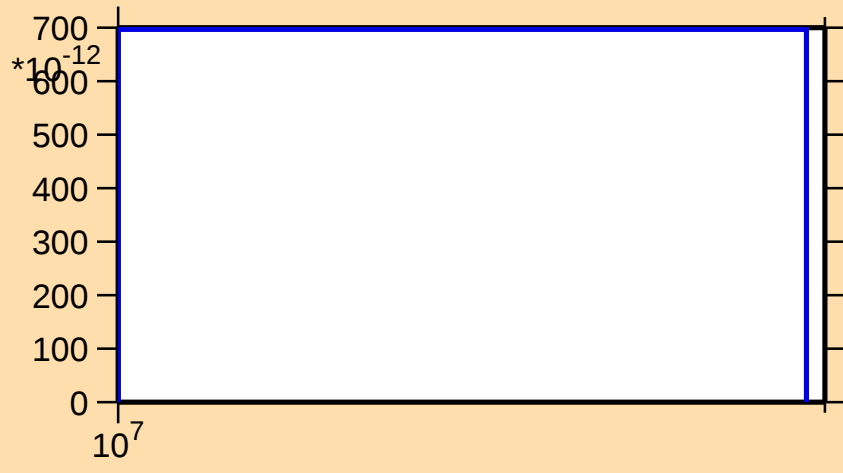
\sigma vs. E for ^{199}\text{Au}(n,\text{nd})
