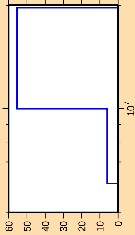
\Delta\sigma/\sigma vs. E for ^{199}\text{Au}(n,np)
