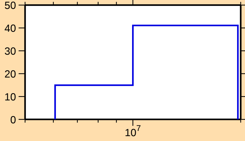
\Delta\sigma/\sigma vs. E for ^{199}\text{Au}(n,\text{inel.})
