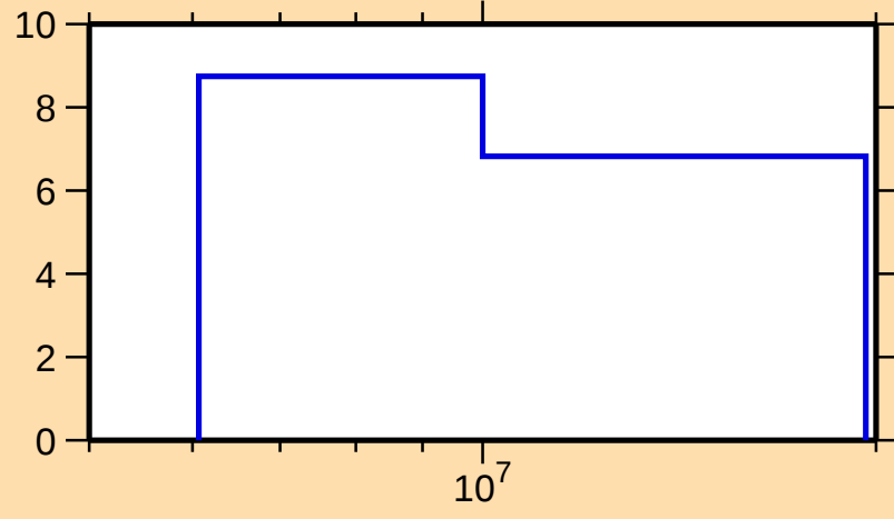
\Delta\sigma/\sigma vs. E for ^{199}\text{Au}(n,\text{nonel.})
