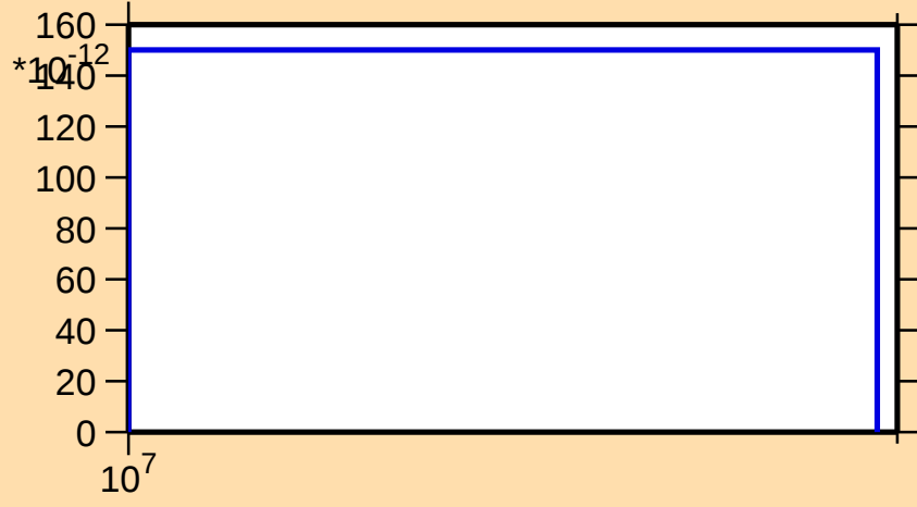
\sigma vs. E for ^{199}\text{Au}(n,2np)
