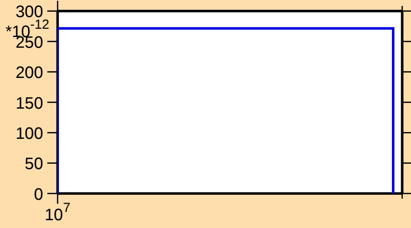
\sigma vs. E for ^{199}\text{Au}(n,nt)
