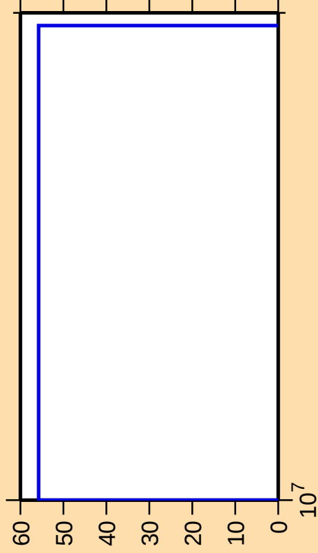
\Delta\sigma/\sigma vs. E for ^{199}\text{Au}(n,3n)
