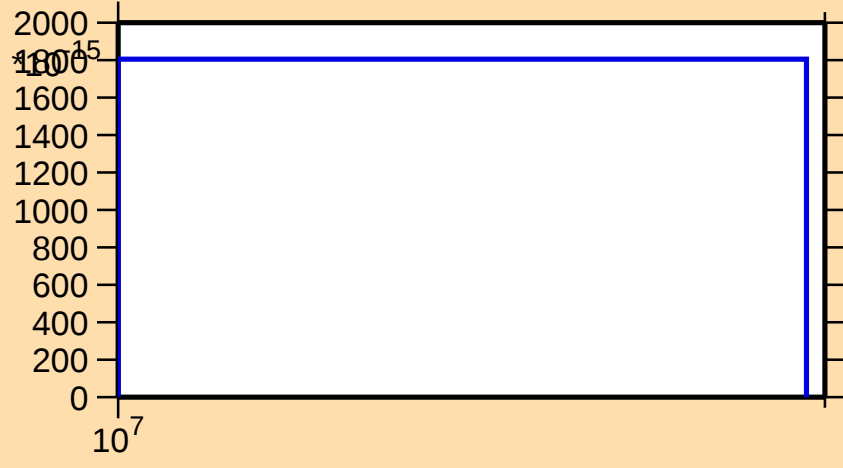
\sigma vs. E for ^{199}\text{Au}(n,2n\alpha)
