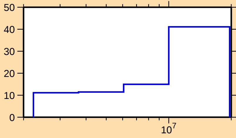
\Delta\sigma/\sigma vs. E for ^{199}\text{Au}(n,\text{inel.})
