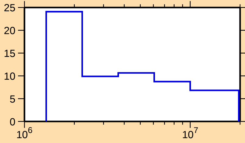
\Delta\sigma/\sigma vs. E for ^{199}\text{Au}(n,\text{nonel.})
