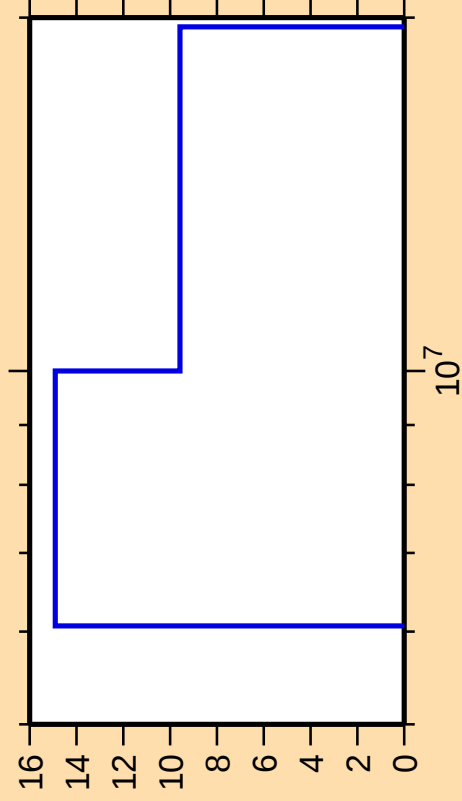
\Delta\sigma/\sigma vs. E for ^{199}\text{Au}(n,2n)
