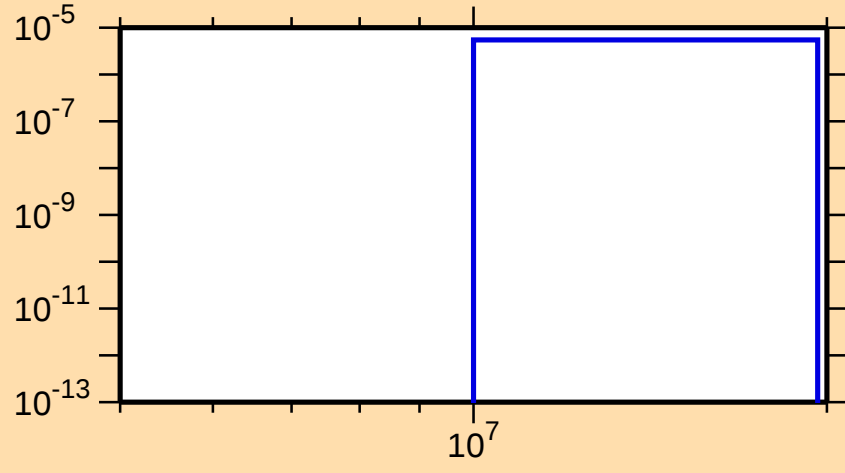
\sigma vs. E for ^{199}\text{Au}(n,t)
