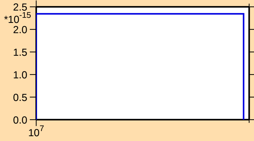
\sigma vs. E for ^{199}\text{Au}(n,\text{He}3)
