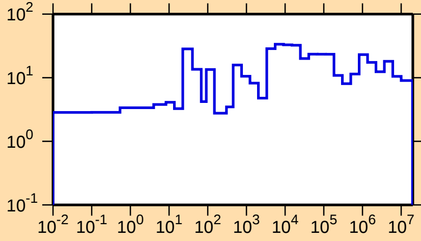
\Delta\sigma/\sigma vs. E for ^{199}\text{Au}(n,\text{el.})
