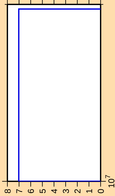
\Delta\sigma/\sigma vs. E for ^{199}\text{Au}(n,2n\alpha)
