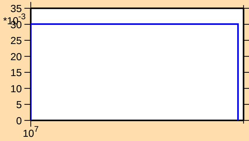
\sigma vs. E for ^{199}\text{Au}(n,3n)
