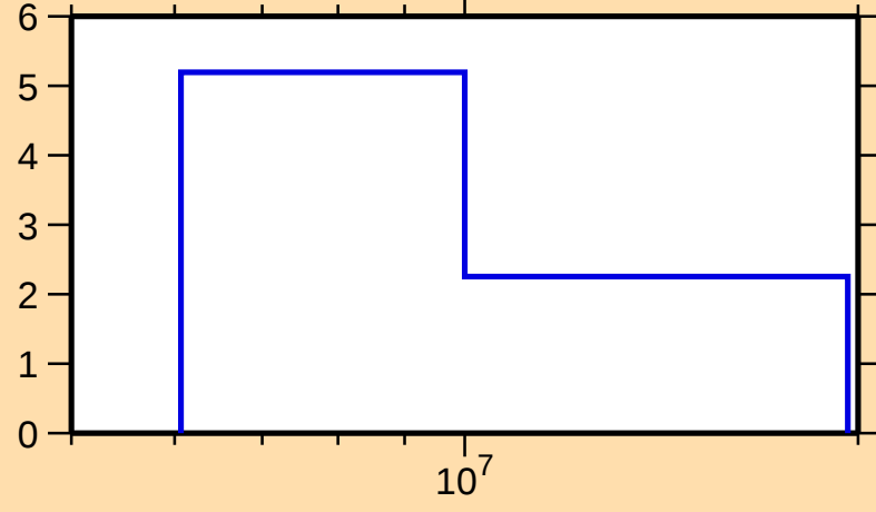
\Delta\sigma/\sigma vs. E for ^{199}\text{Au}(n,\text{tot.})
