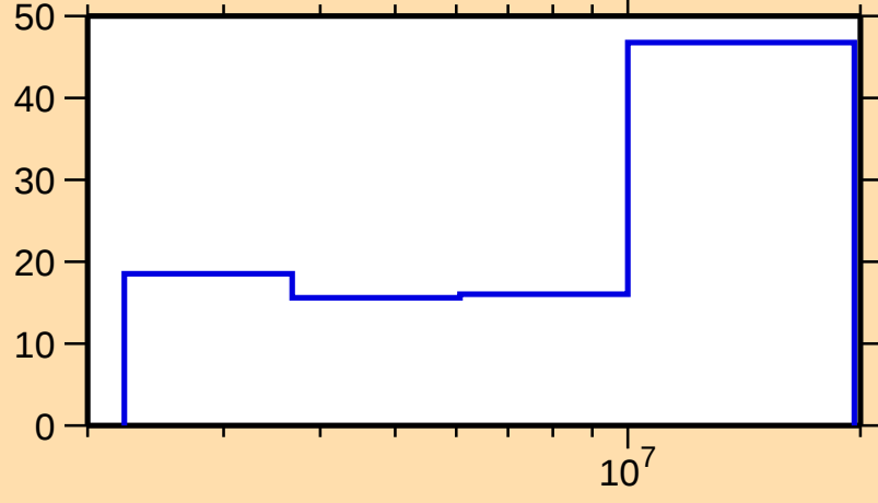
\Delta\sigma/\sigma vs. E for ^{199}\text{Au}(n,n\text{cont.})
