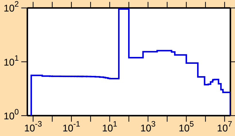
\sigma vs. E for ^{199}\text{Au}(n,\text{el.})
