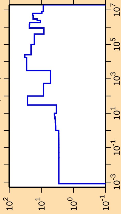
\Delta\sigma/\sigma vs. E for ^{199}\text{Au}(n,\text{el.})
