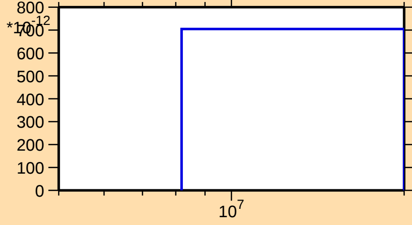
\sigma vs. E for ^{199}\text{Au}(n,\text{nd})
