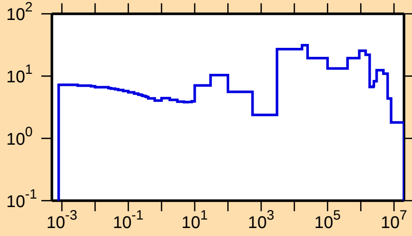
\Delta\sigma/\sigma vs. E for ^{199}\text{Au}(n,\text{tot.})
