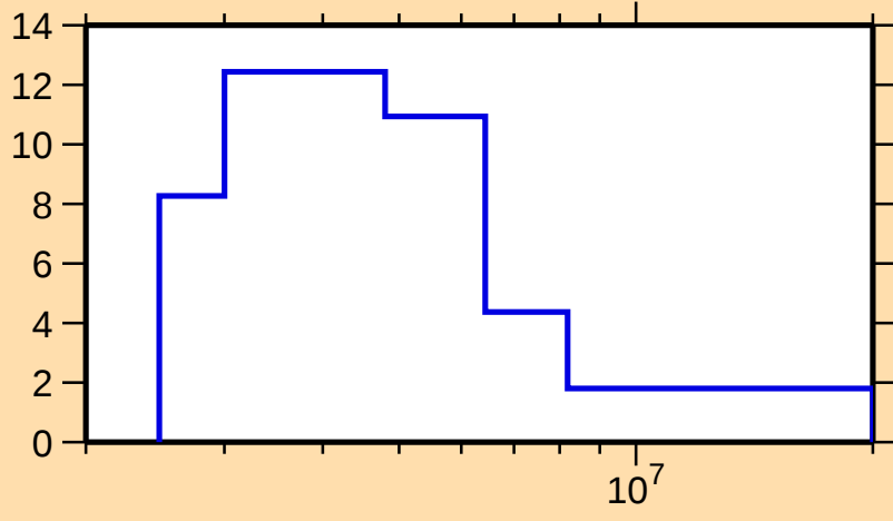
\Delta\sigma/\sigma vs. E for ^{199}\text{Au}(n,\text{tot.})
