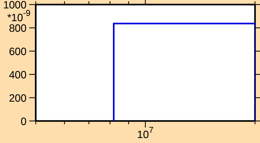
\sigma vs. E for ^{199}\text{Au}(n,n\alpha)
