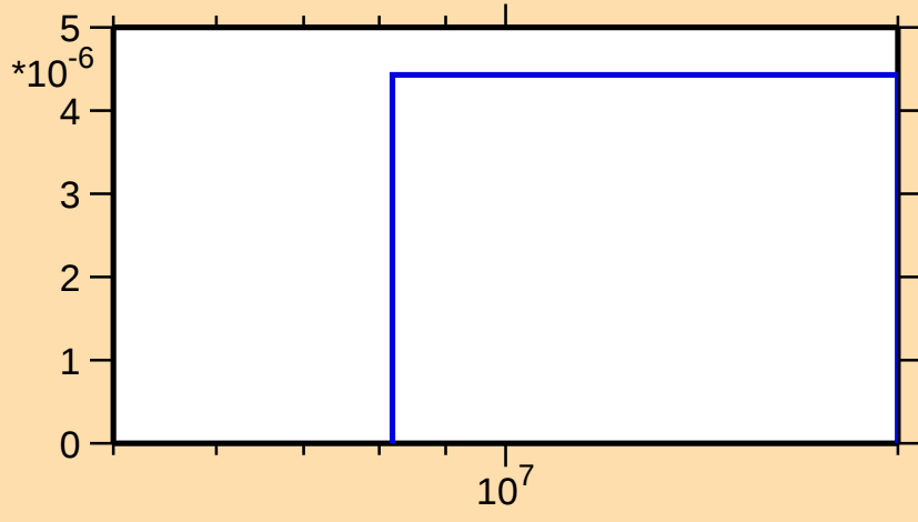
\sigma vs. E for ^{199}\text{Au}(n,t)
