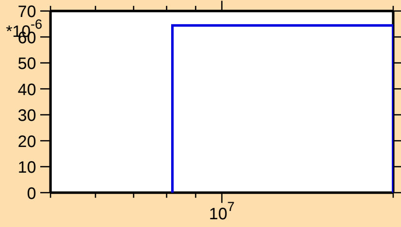
\sigma vs. E for ^{199}\text{Au}(n,np)
