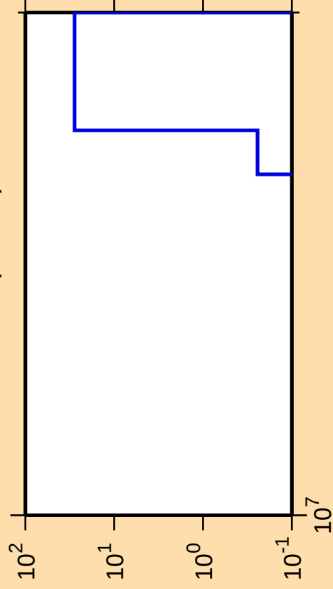
\Delta\sigma/\sigma vs. E for ^{200}\text{Au}(n,\text{He}3)
