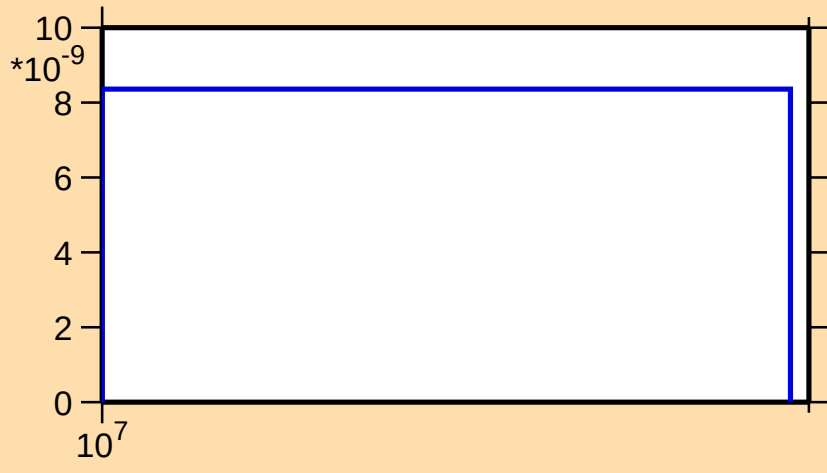
\sigma vs. E for ^{200}\text{Au}(n,\text{nd})
