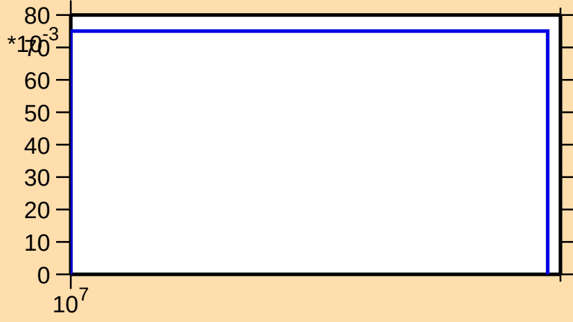
\sigma vs. E for ^{200}\text{Au}(n,3n)
