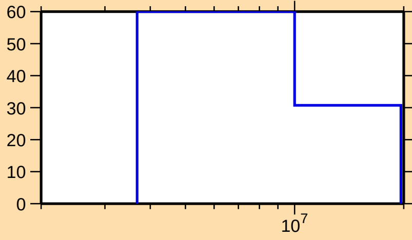
\Delta\sigma/\sigma vs. E for ^{200}\text{Au}(n,2n)
