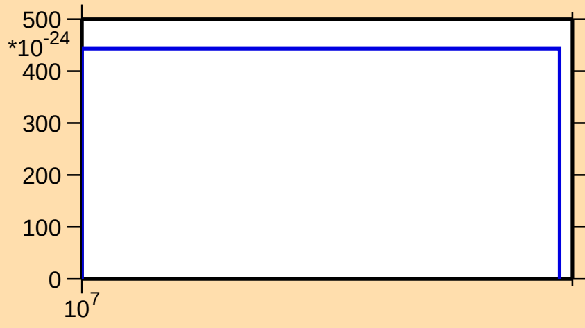
\sigma vs. E for ^{200}\text{Au}(\text{mt } 42)
