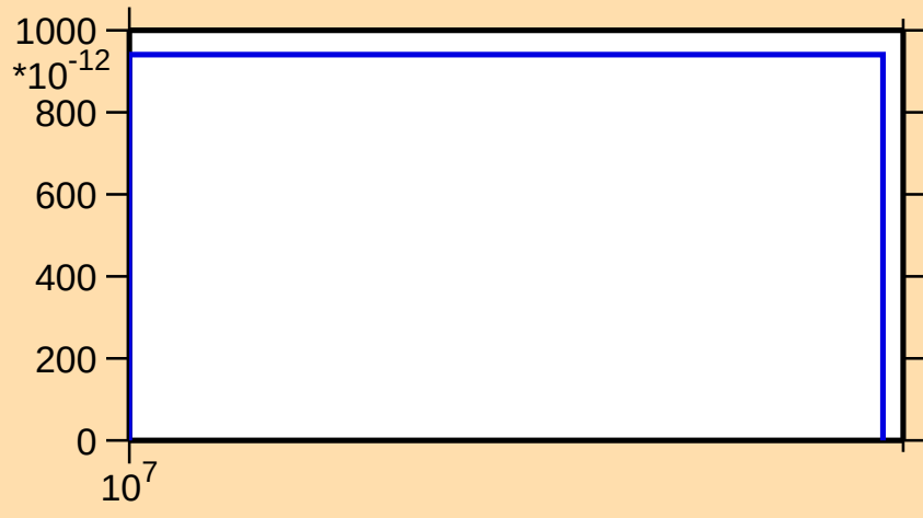
\sigma vs. E for ^{200}\text{Au}(n,nt)
