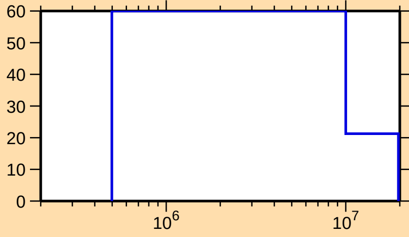
\Delta\sigma/\sigma vs. E for ^{200}\text{Au}(n, n_1)
