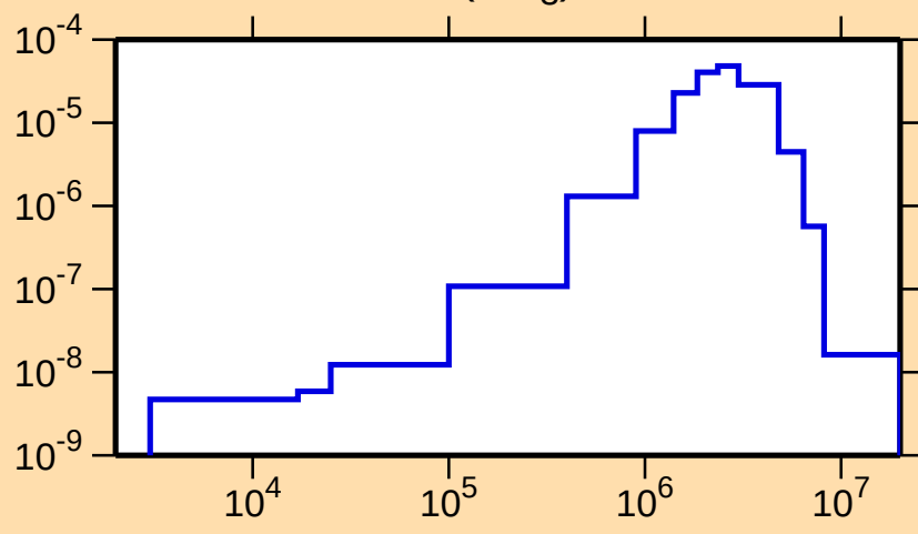
\sigma vs. E for ^{200}\text{Au}(n,n_3)
