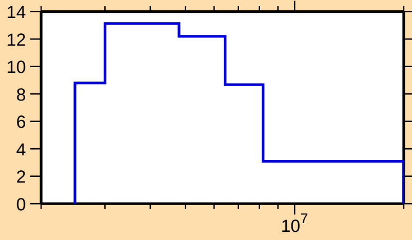
\Delta\sigma/\sigma vs. E for ^{200}\text{Au}(n,\text{tot.})
