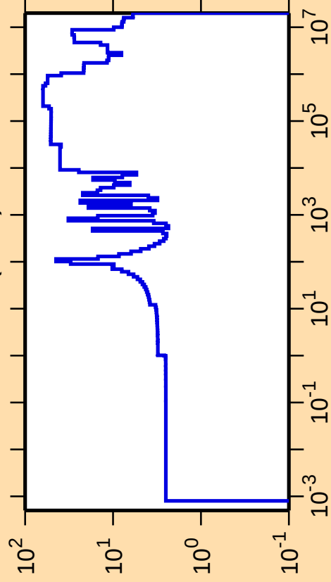
\Delta\sigma/\sigma vs. E for ^{201}\text{Au}(n,\text{el.})
