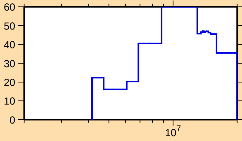
\Delta\sigma/\sigma vs. E for ^{201}\text{Au}(n,n\text{cont.})
