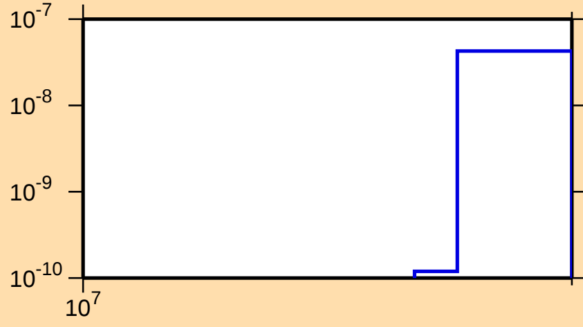
\sigma vs. E for ^{201}\text{Au}(n,\text{nd})
