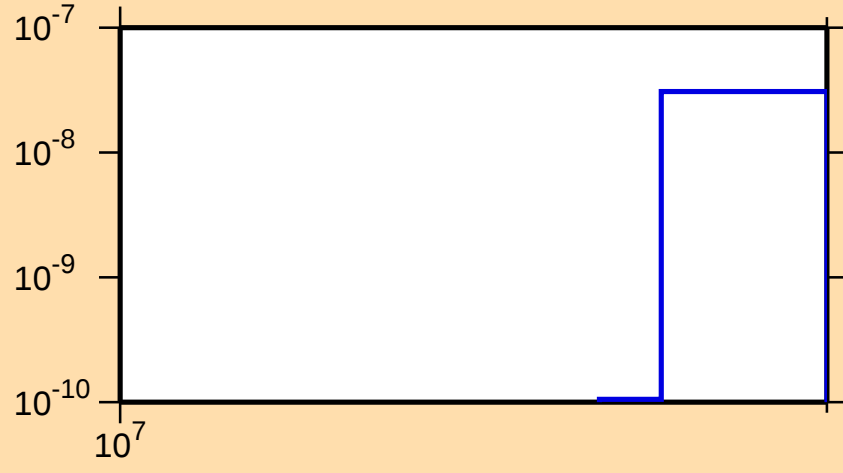
\sigma vs. E for ^{201}\text{Au}(n,nt)
