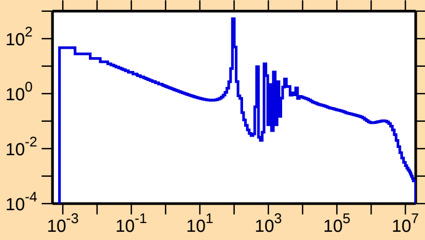
\sigma vs. E for ^{201}\text{Au}(n,\gamma)
