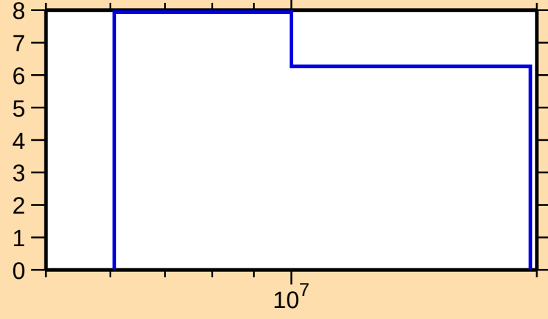
\Delta\sigma/\sigma vs. E for ^{201}\text{Au}(n,\text{nonel.})
