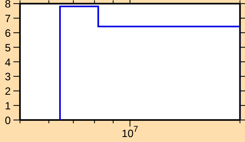
\Delta\sigma/\sigma vs. E for ^{201}\text{Au}(n,\text{nonel.})
