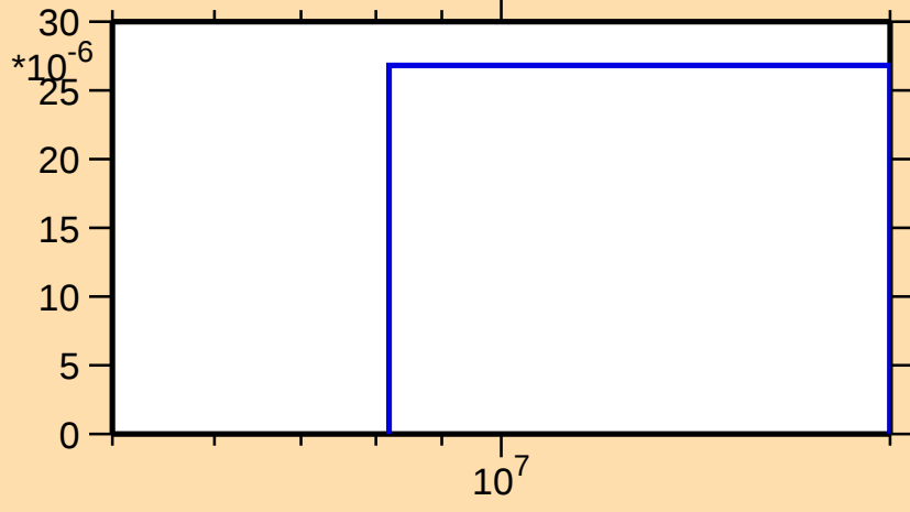
\sigma vs. E for ^{201}\text{Au}(n,np)
