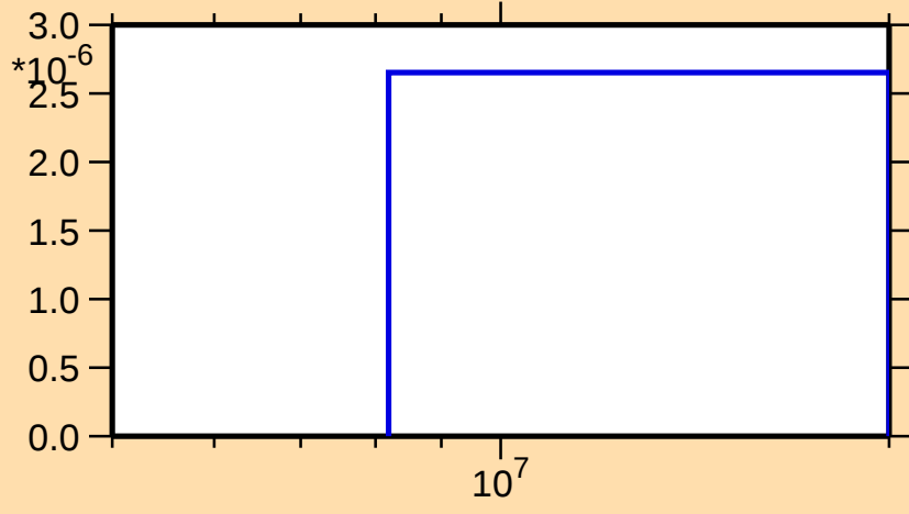
\sigma vs. E for ^{201}\text{Au}(n,t)
