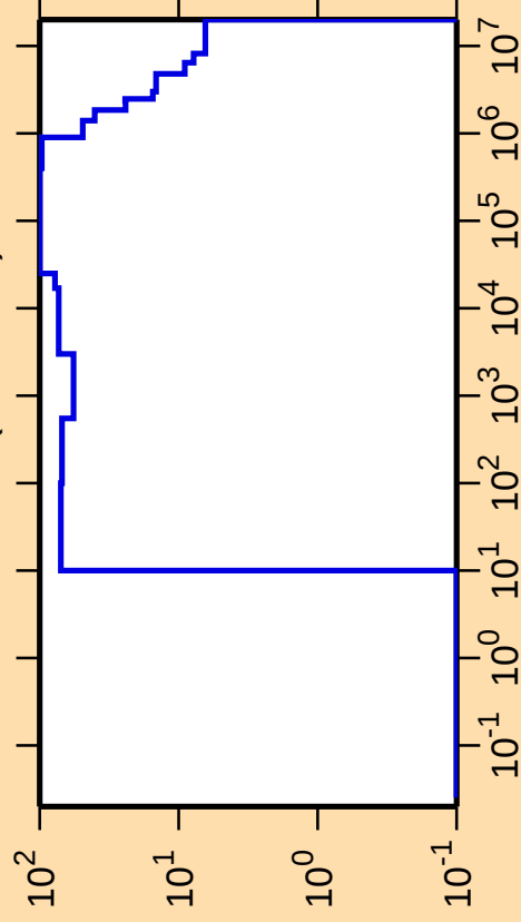
\Delta\sigma/\sigma vs. E for ^{201}\text{Au}(n,\text{nonel.})
