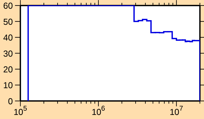
\Delta\sigma/\sigma vs. E for ^{207}\text{Au}(n,n_1)
