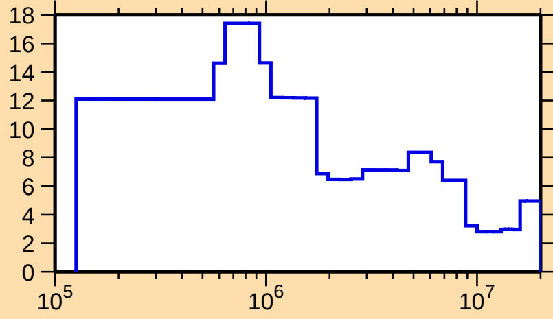
\Delta\sigma/\sigma vs. E for ^{207}\text{Au}(n,\text{tot.})
