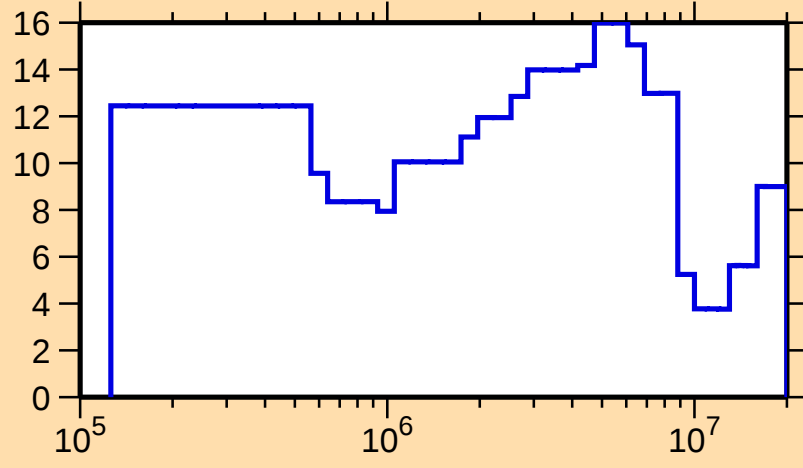
\Delta\sigma/\sigma vs. E for ^{207}\text{Au}(n,\text{el.})
