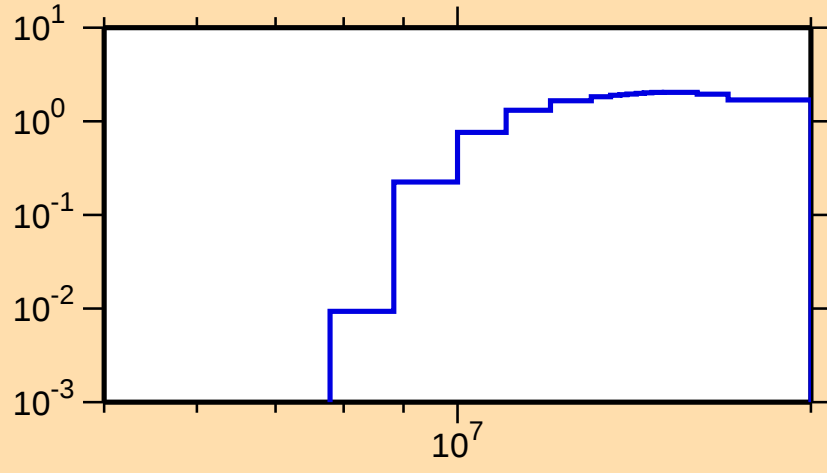
\sigma vs. E for ^{207}\text{Au}(n,3n)
