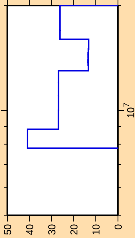
\Delta\sigma/\sigma vs. E for ^{207}\text{Au}(n,3n)
