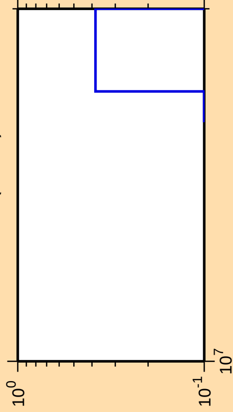
\Delta\sigma/\sigma vs. E for ^{207}\text{Au}(n,3n\alpha)
