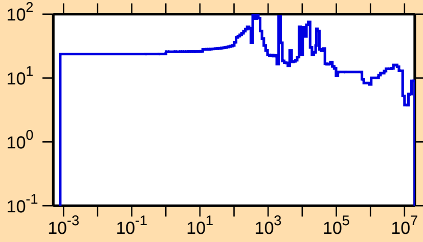
\Delta\sigma/\sigma vs. E for ^{207}\text{Au}(n,\text{el.})
