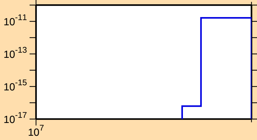
\sigma vs. E for ^{207}\text{Au}(\text{mt } 11)
