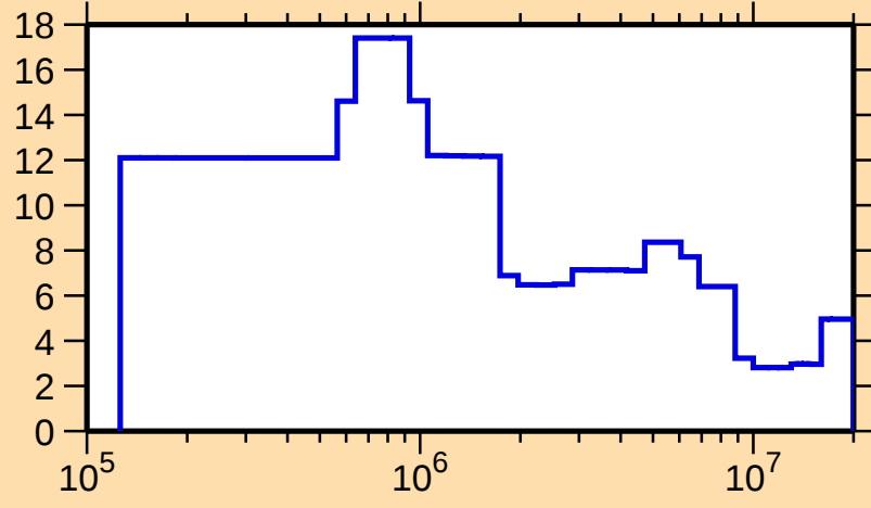
\Delta\sigma/\sigma vs. E for ^{207}\text{Au}(n,\text{tot.})
