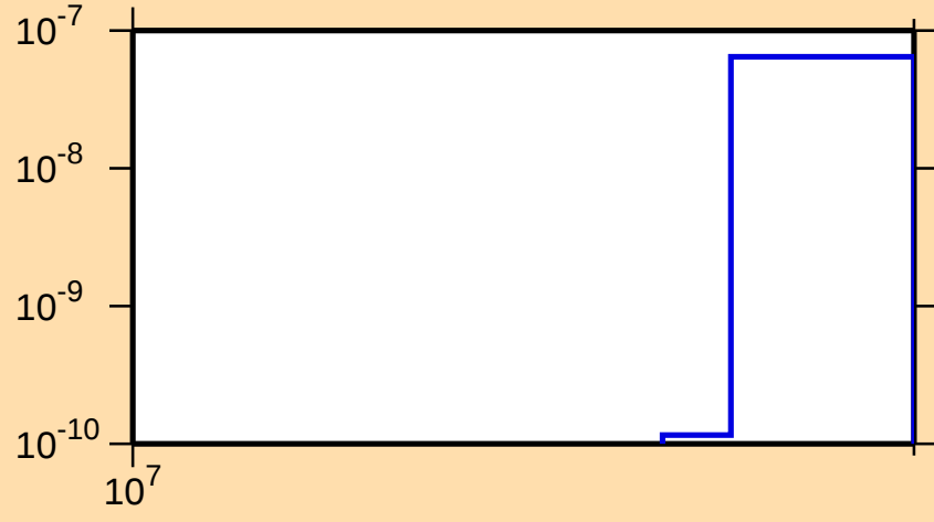
\sigma vs. E for ^{207}\text{Au}(n,2np)
