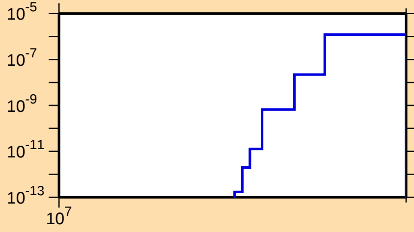
\sigma vs. E for ^{207}\text{Au}(n,\text{nd})
