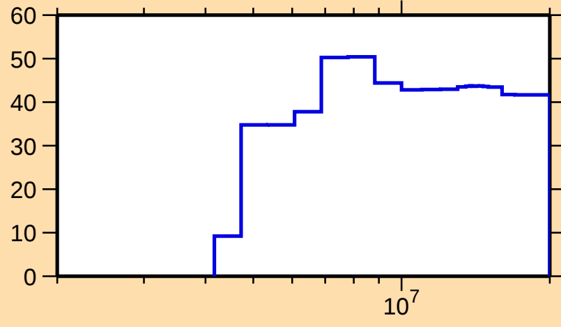
\Delta\sigma/\sigma vs. E for ^{207}\text{Au}(n,n\text{cont.})
