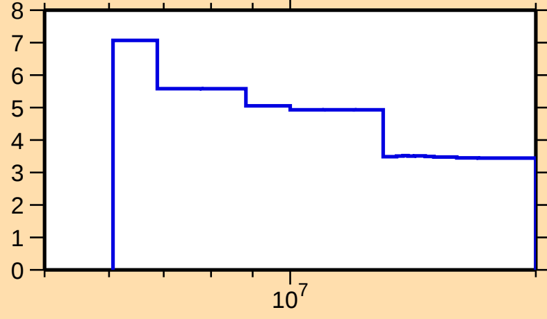
\Delta\sigma/\sigma vs. E for ^{207}\text{Au}(n,\text{nonel.})
