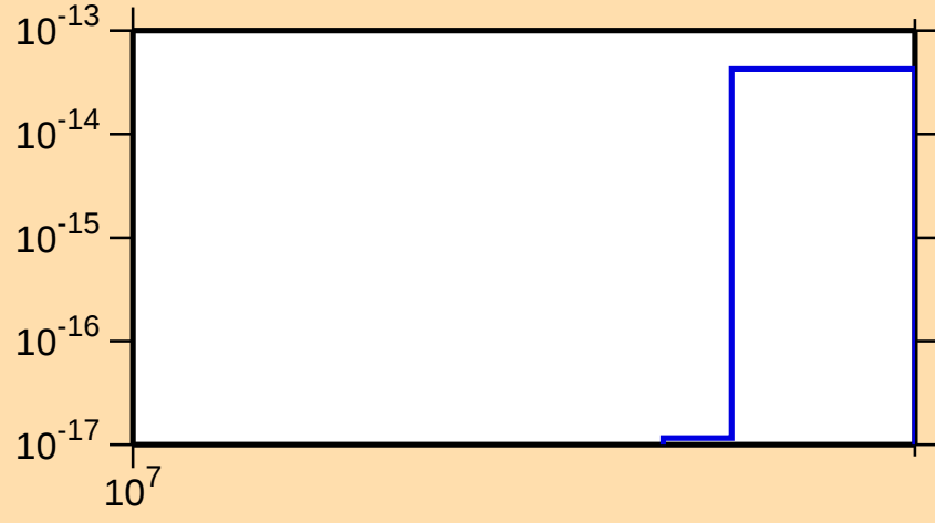
\sigma vs. E for ^{207}\text{Au}(n,3n\alpha)
