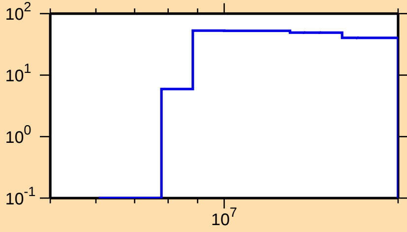
\Delta\sigma/\sigma vs. E for ^{207}\text{Au}(n,p)
