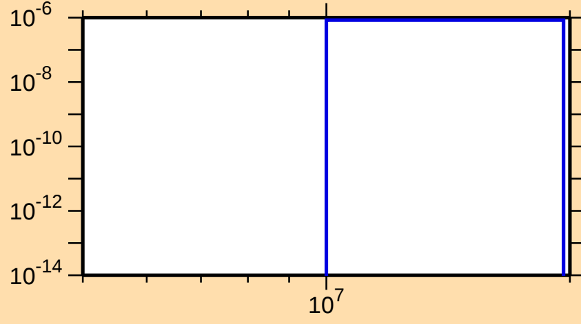
\sigma vs. E for ^{207}\text{Au}(n,nt)
