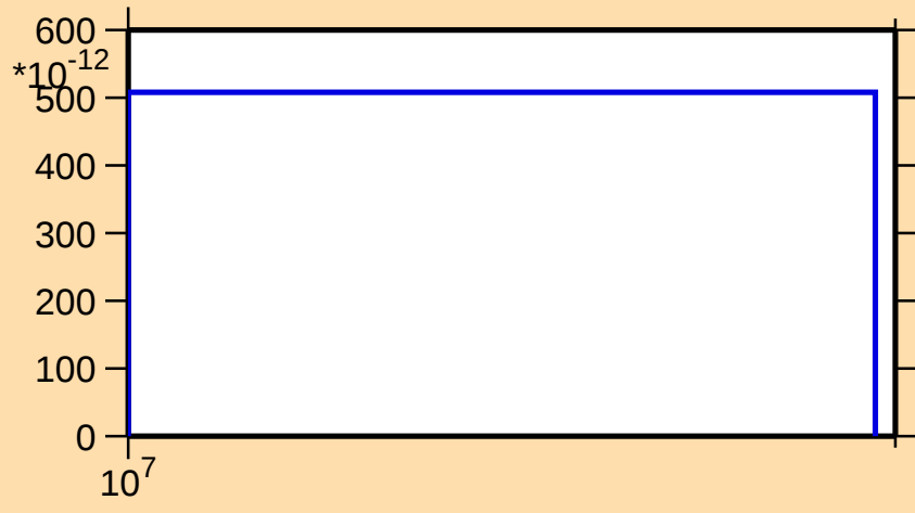
\sigma vs. E for ^{207}\text{Au}(n,2np)
