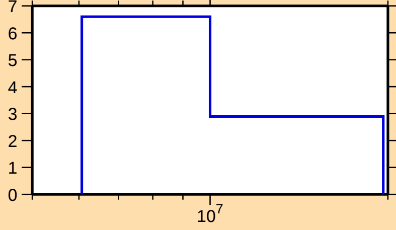
\Delta\sigma/\sigma vs. E for ^{207}\text{Au}(n,\text{tot.})
