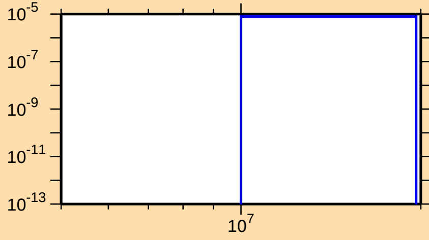
\sigma vs. E for ^{207}\text{Au}(n,np)
