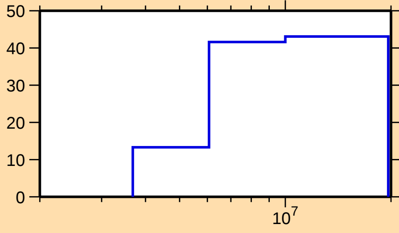
\Delta\sigma/\sigma vs. E for ^{207}\text{Au}(n,n\text{cont.})
