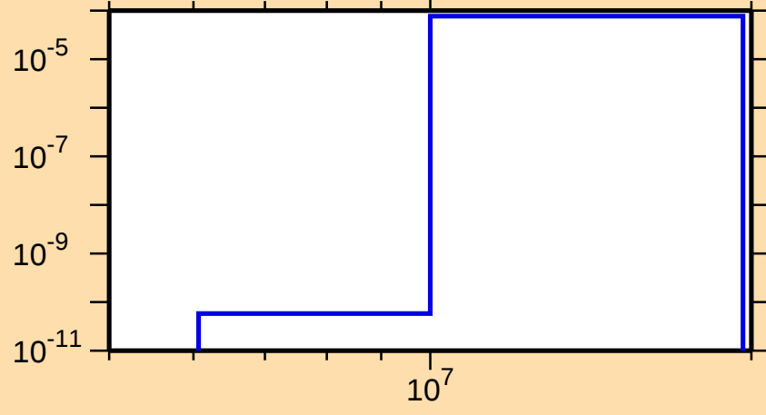
\sigma vs. E for ^{207}\text{Au}(n,p)
