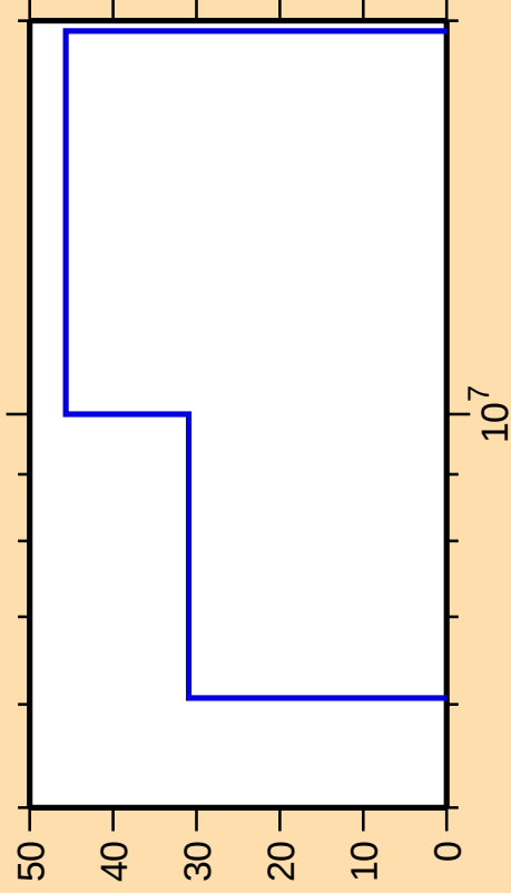
\Delta\sigma/\sigma vs. E for ^{207}\text{Au}(n,p)
