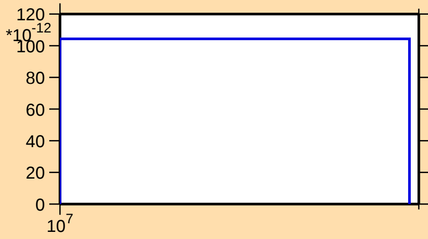
\sigma vs. E for ^{207}\text{Au}(n,2n\alpha)
