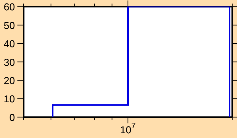
\Delta\sigma/\sigma vs. E for ^{207}\text{Au}(n,2n)
