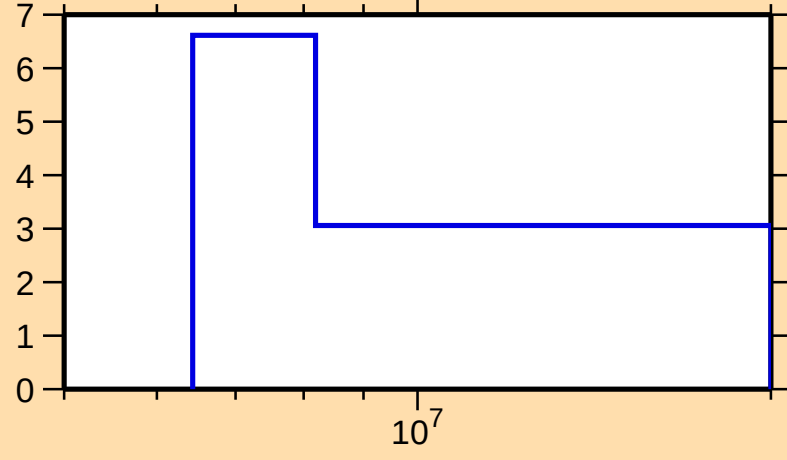
\Delta\sigma/\sigma vs. E for ^{207}\text{Au}(n,\text{tot.})
