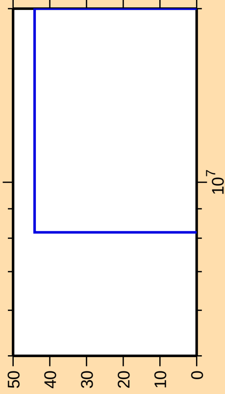
\Delta\sigma/\sigma vs. E for ^{207}\text{Au}(n,np)
