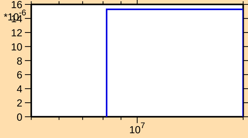
\sigma vs. E for ^{207}\text{Au}(n,t)
