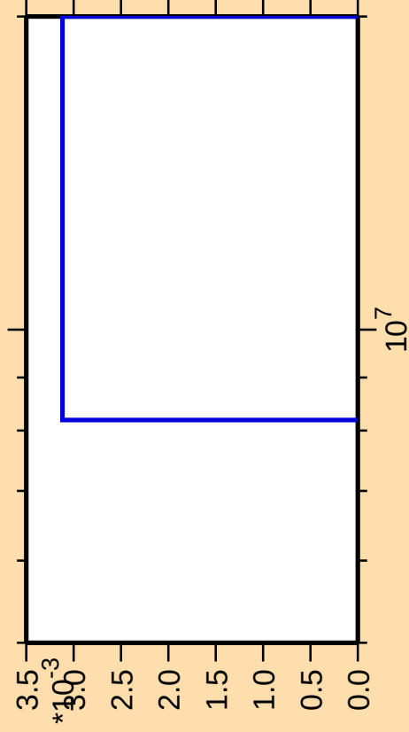
\Delta\sigma/\sigma vs. E for ^{207}\text{Au}(n,3n\alpha)
