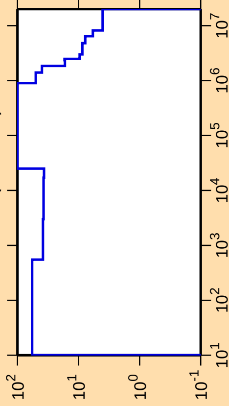
\Delta\sigma/\sigma vs. E for ^{207}\text{Au}(n,\text{nonel.})
