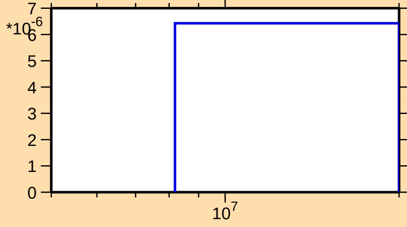
\sigma vs. E for ^{207}\text{Au}(n,np)
