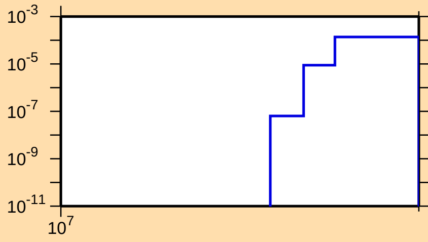
\sigma vs. E for ^{119}\text{Ba}(n,2np)
