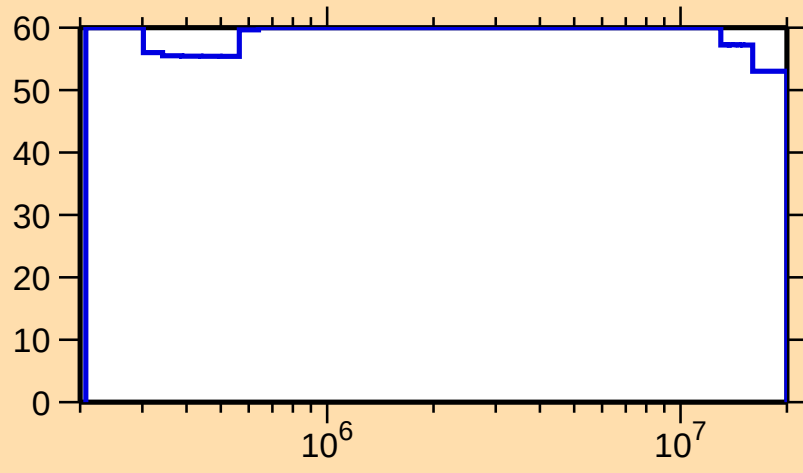
\Delta\sigma/\sigma vs. E for ^{119}\text{Ba}(n,n_1)
