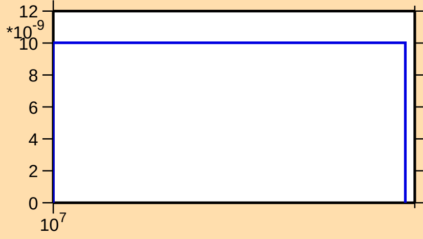
\sigma vs. E for ^{119}\text{Ba}(n,\text{nd})
