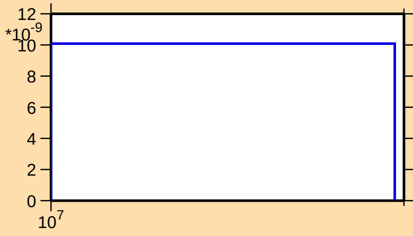
\sigma vs. E for ^{119}\text{Ba}(n,2n\alpha)
