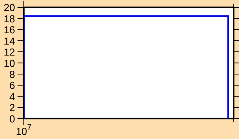
\Delta\sigma/\sigma vs. E for ^{119}\text{Ba}(n,\text{tot.})
