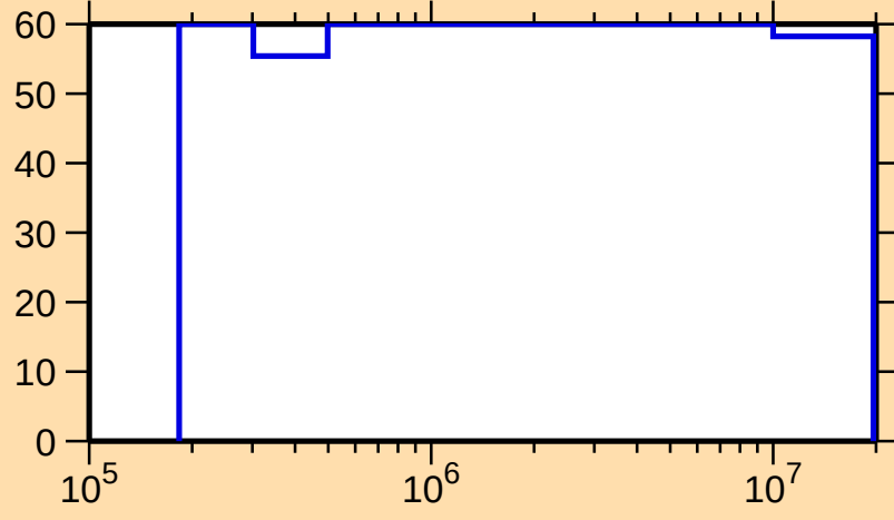
\Delta\sigma/\sigma vs. E for ^{119}\text{Ba}(n,n_1)
