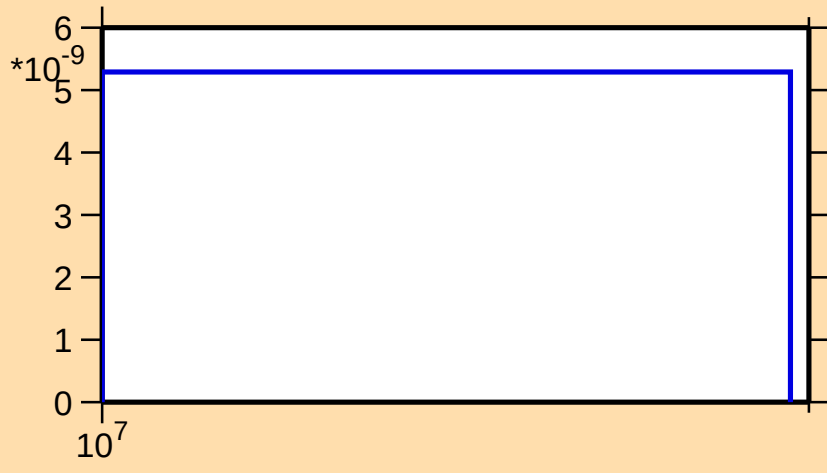
\sigma vs. E for ^{119}\text{Ba} (mt 34)
