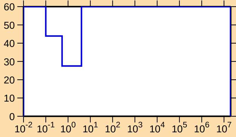
\Delta\sigma/\sigma vs. E for ^{119}\text{Ba}(n,\gamma)
