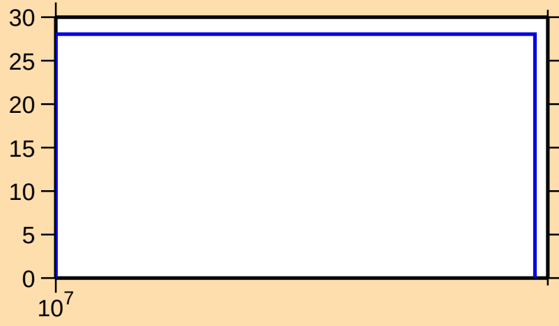
\Delta\sigma/\sigma vs. E for ^{119}\text{Ba}(n,\text{el.})
