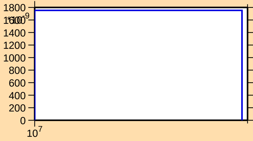
\sigma vs. E for ^{119}\text{Ba}(n,2np)
