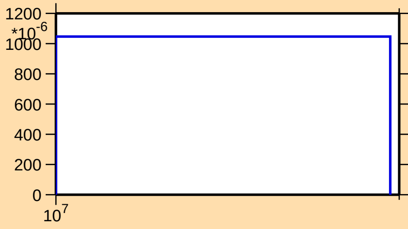
\sigma vs. E for ^{119}\text{Ba}(n,2n)
