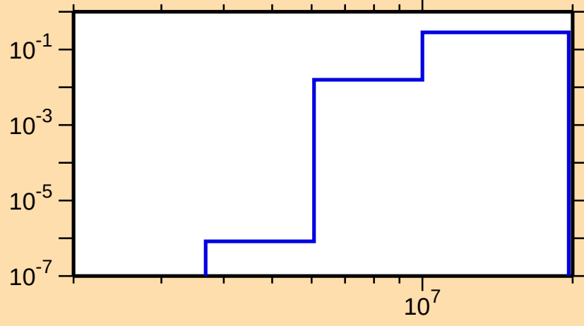
\sigma vs. E for ^{119}\text{Ba}(n,np)
