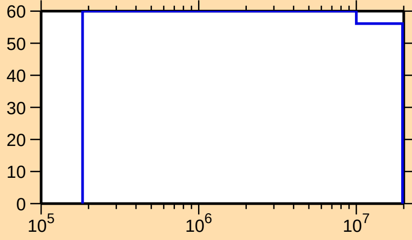
\Delta\sigma/\sigma vs. E for ^{119}\text{Ba}(n,\text{inel.})
