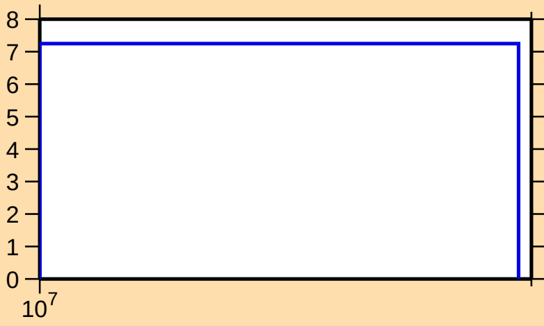
\Delta\sigma/\sigma vs. E for ^{119}\text{Ba}(n,\text{nonel.})
