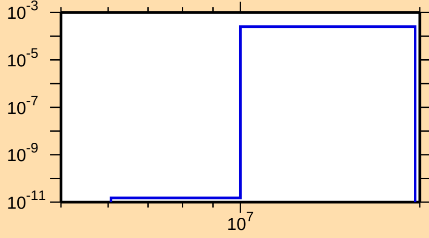
\sigma vs. E for ^{119}\text{Ba}(n,t)
