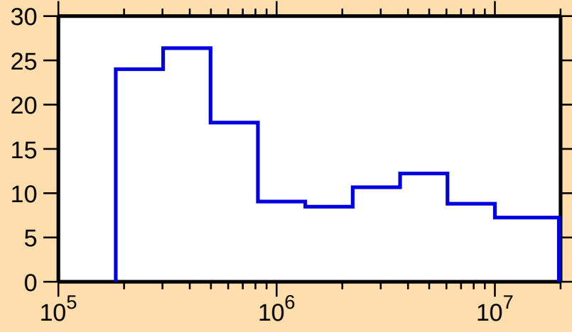
\Delta\sigma/\sigma vs. E for ^{119}\text{Ba}(n,\text{nonel.})
