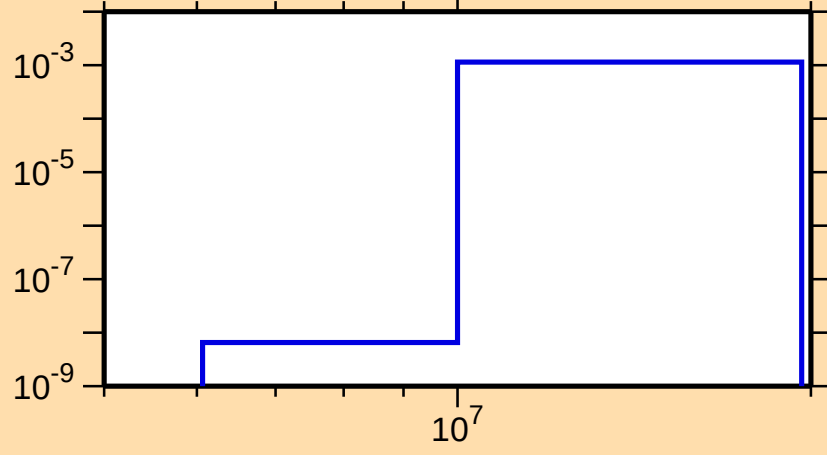
\sigma vs. E for ^{119}\text{Ba}(n,\text{pd})
