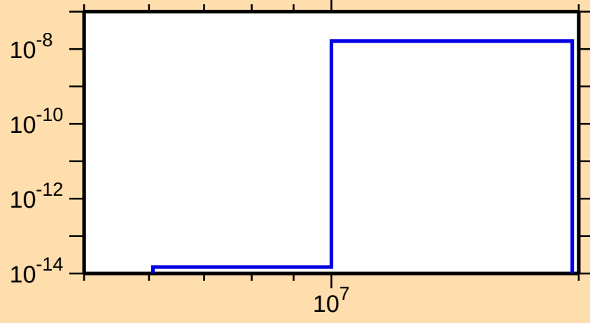
\sigma vs. E for ^{119}\text{Ba}(\text{mt117})
