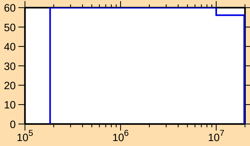
\Delta\sigma/\sigma vs. E for ^{119}\text{Ba}(n,\text{inel.})
