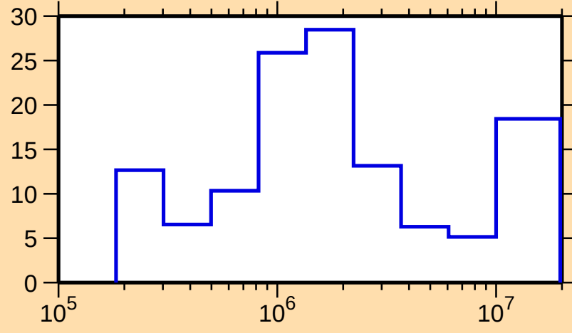
\Delta\sigma/\sigma vs. E for ^{119}\text{Ba}(n,\text{tot.})
