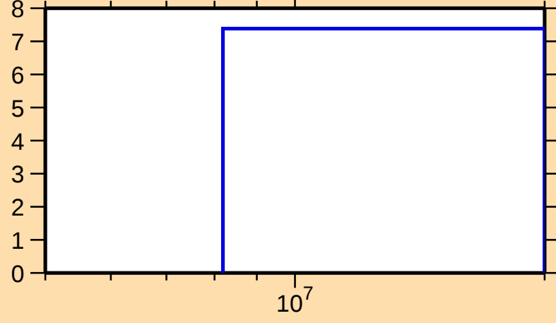
\Delta\sigma/\sigma vs. E for ^{119}\text{Ba}(n,\text{nonel.})
