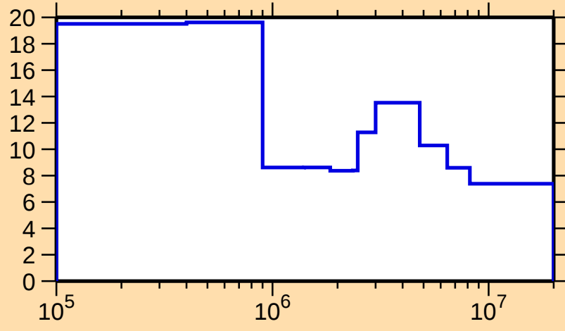
\Delta\sigma/\sigma vs. E for ^{119}\text{Ba}(n,\text{nonel.})
