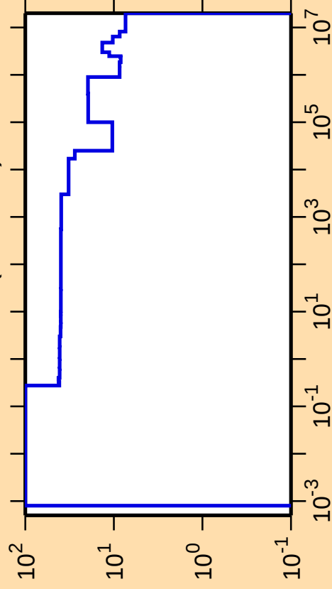
\Delta\sigma/\sigma vs. E for ^{119}\text{Ba}(n,\text{nonel.})
