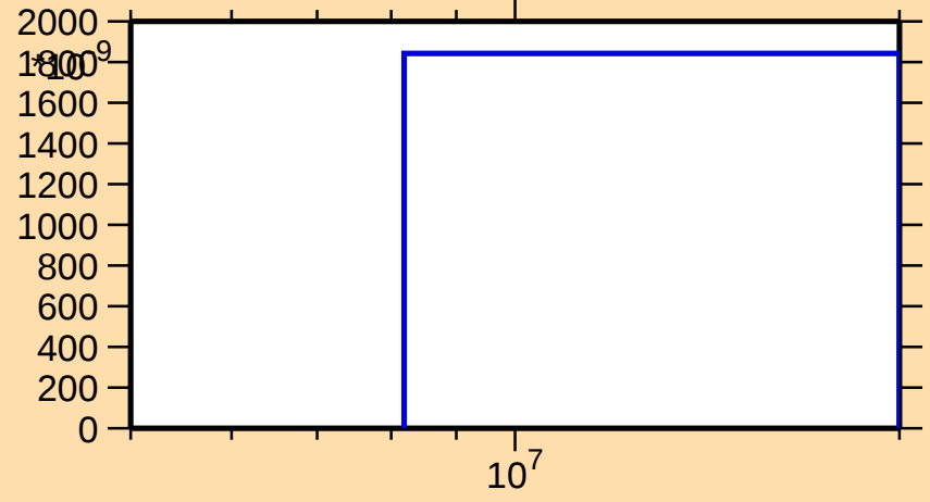
\sigma vs. E for ^{119}\text{Ba} (mt 45)
