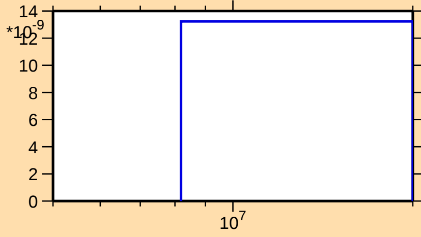
\sigma vs. E for ^{119}\text{Ba}(\text{mt117})
