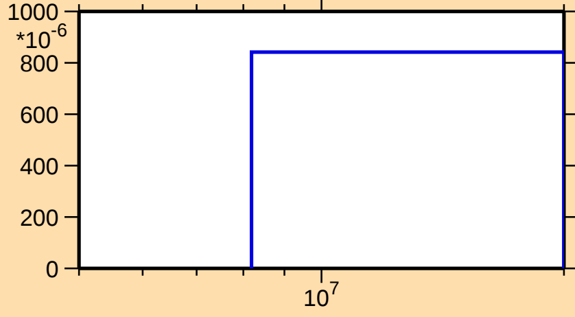
\sigma vs. E for ^{119}\text{Ba}(n,2n)
