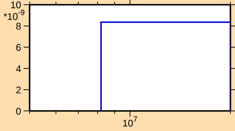
\sigma vs. E for ^{119}\text{Ba}(n,\text{nd})
