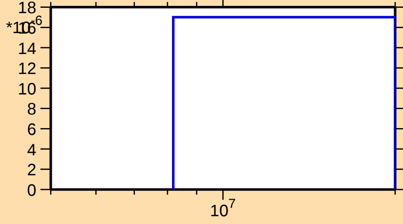
\sigma vs. E for ^{119}\text{Ba}(n,\text{pt})
