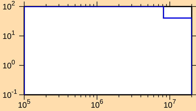
\Delta\sigma/\sigma vs. E for ^{119}\text{Ba}(n,n\text{cont.})
