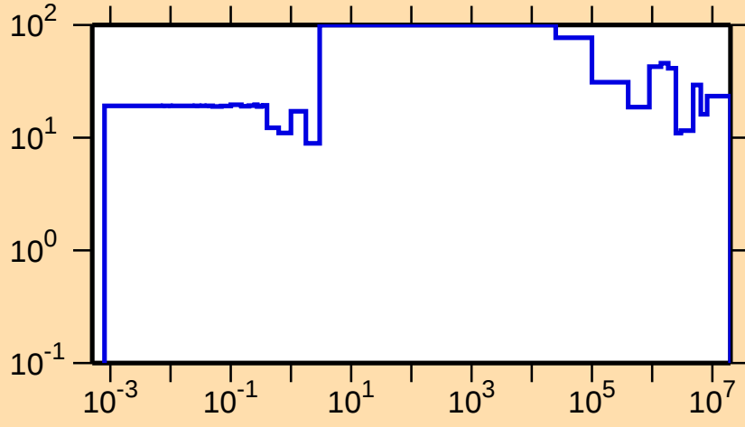
\Delta\sigma/\sigma vs. E for ^{119}\text{Ba}(n,\text{el.})
