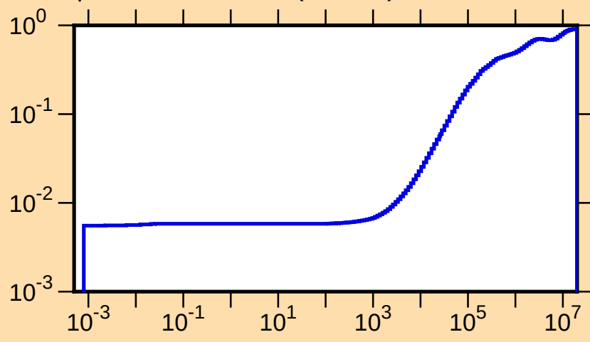
\mu vs. E for ^{122}\text{Ba}(\text{mt251})
