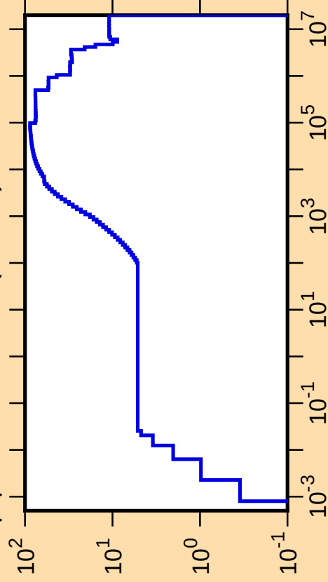
\Delta\mu/\mu vs. E for ^{122}\text{Ba}(\text{mt251})
