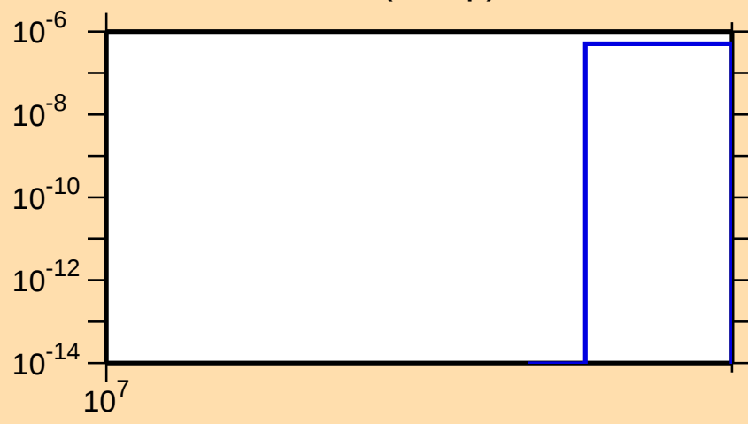
\sigma vs. E for ^{122}\text{Ba}(n,2np)
