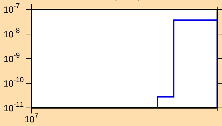
\sigma vs. E for ^{122}\text{Ba}(n,\text{nd})
