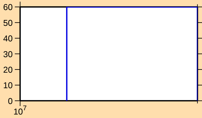
\Delta\sigma/\sigma vs. E for ^{122}\text{Ba}(n,2n)
