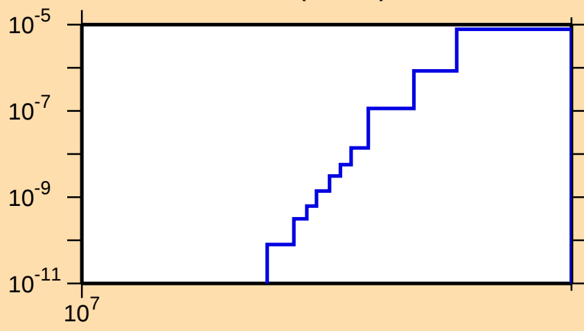
\sigma vs. E for ^{122}\text{Ba}(\text{mt } 45)
