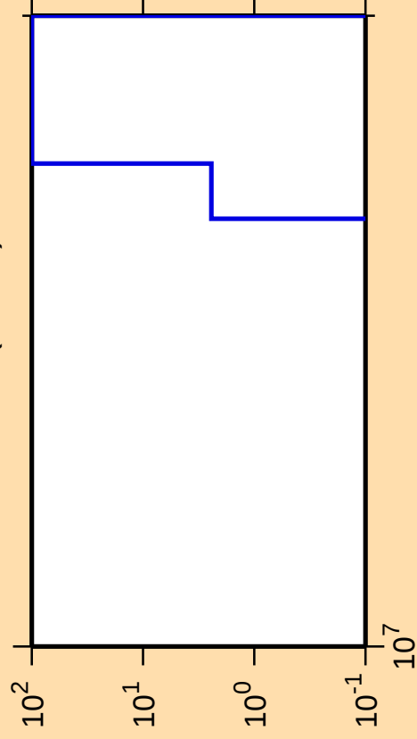
\Delta\sigma/\sigma vs. E for ^{122}\text{Ba} (mt 34)
