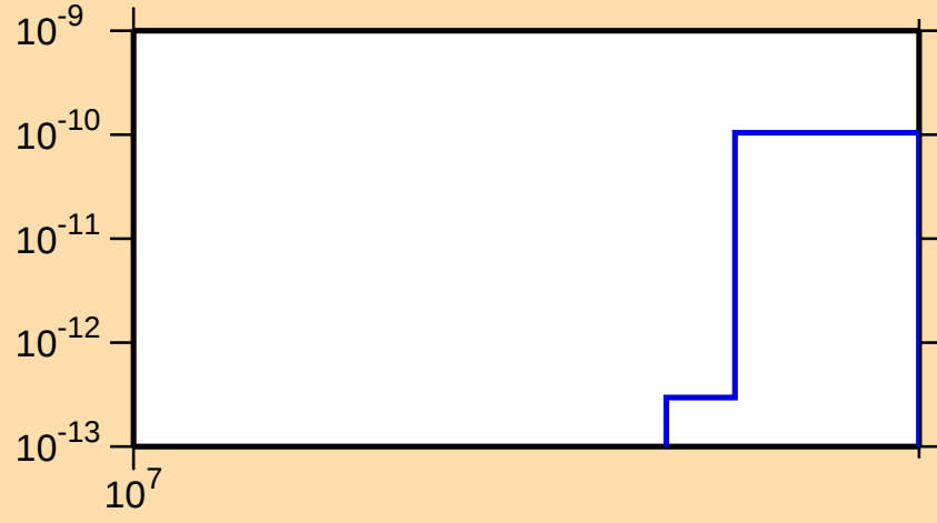
\sigma vs. E for ^{122}\text{Ba} (mt 34)
