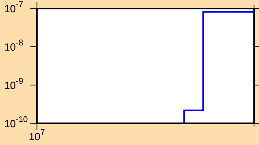
\sigma vs. E for ^{122}\text{Ba}(n,\text{pt})
