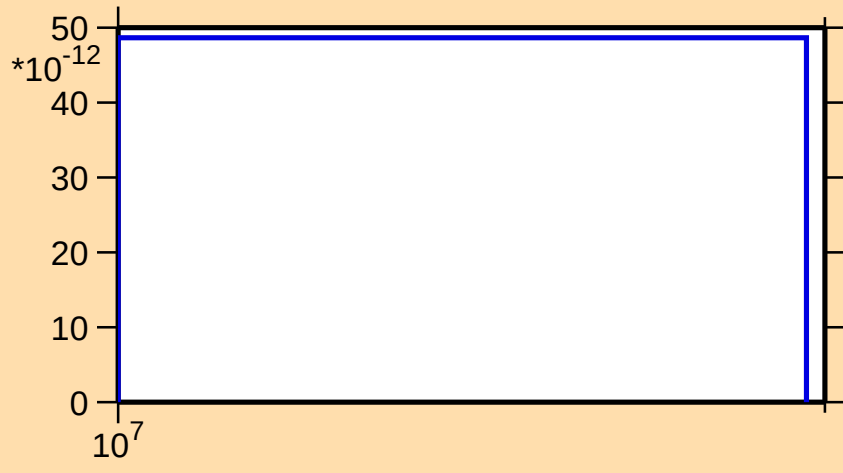
\sigma vs. E for ^{122}\text{Ba}(n,2n\alpha)
