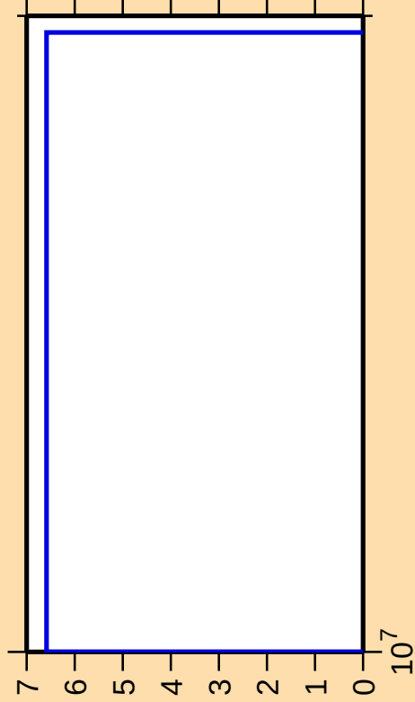
\Delta\sigma/\sigma vs. E for ^{122}\text{Ba} (mt 34)
