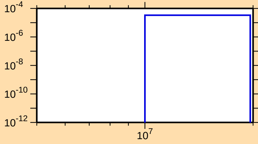
\sigma vs. E for ^{122}\text{Ba}(n,t)
